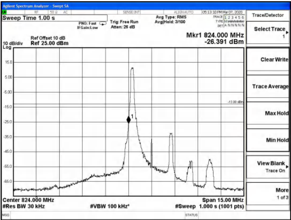
LTE Band26, 3MHz bandwidth, QPSK,(1,0) Mode , Below 824MHz
