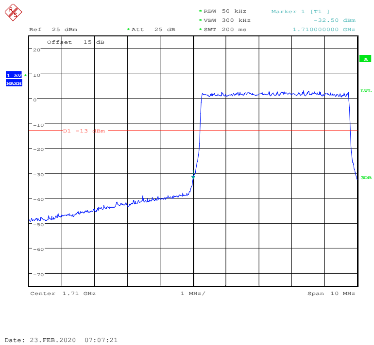
LTE Band66, 5MHz bandwidth, 16QAM,(25,0) Mode , Below 1710MHz
