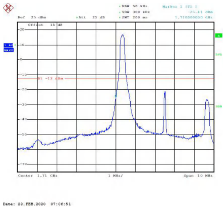
LTE Band66, 5MHz bandwidth, 16QAM,(1,0) Mode , Below 1710MHz
