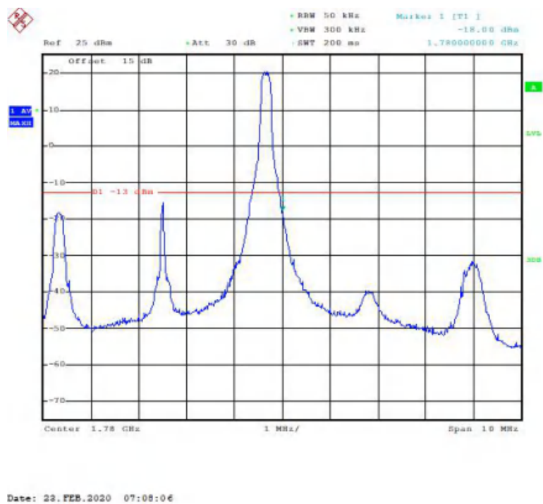
LTE Band66, 5MHz bandwidth, 16QAM,(1,25) Mode, Above 1780MHz
