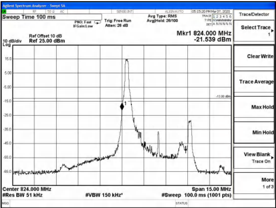
LTE Band26, 5MHz bandwidth, QPSK,(1,0) Mode , Below 824MHz
