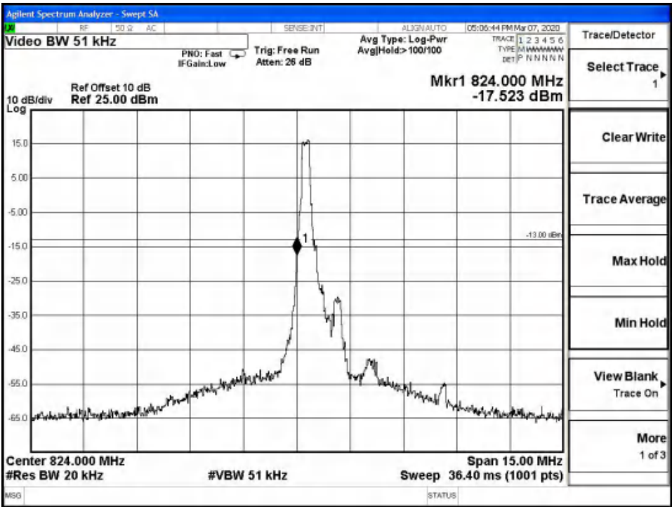
LTE Band26, 1.4MHz bandwidth, 16QAM,(1,0) Mode , Below 824MHz
