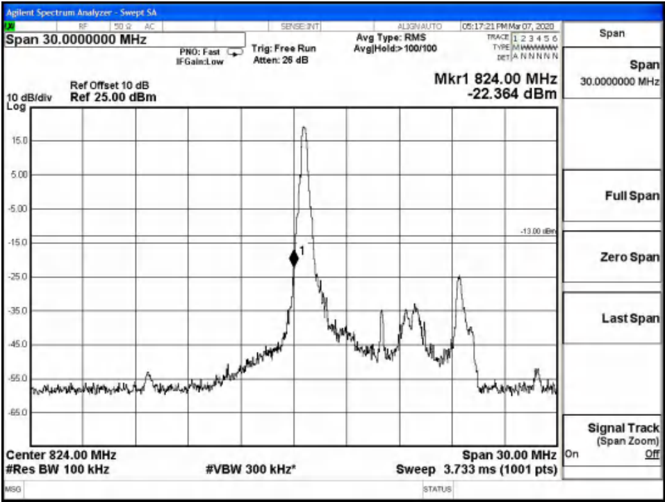
LTE Band26, 10MHz bandwidth, 16QAM,(1,0) Mode , Below 824MHz
