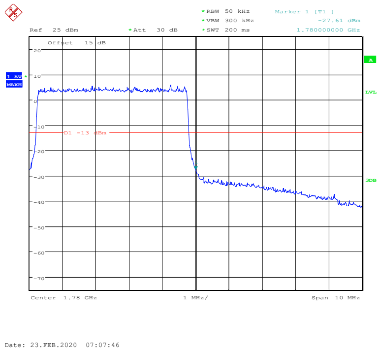
LTE Band66, 5MHz bandwidth, 16QAM,(25,0) Mode, Above 1780MHz
