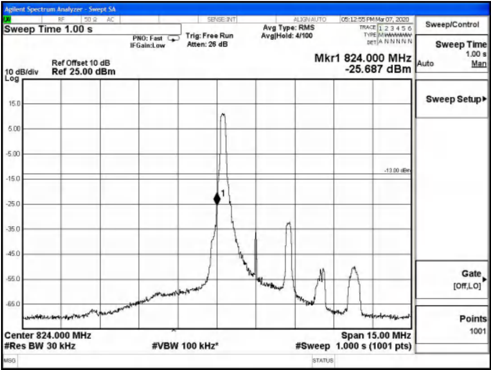
LTE Band26, 3MHz bandwidth, 16QAM,(1,0) Mode , Below 824MHz
