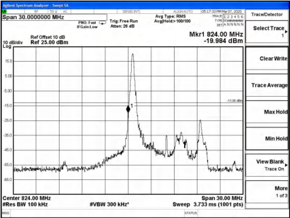
LTE Band26, 10MHz bandwidth, QPSK,(1,0) Mode , Below 824MHz
