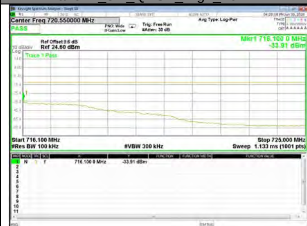
Band12_3M_QPSK_High_Full-RB
