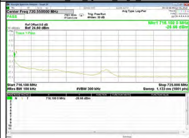
Band12_3M_QPSK_High_Full-RB
