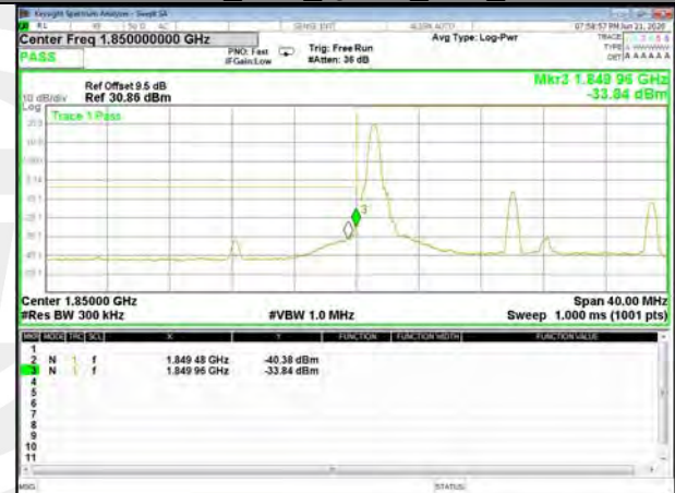
Band25_20M_QPSK_Low_Full-RB
