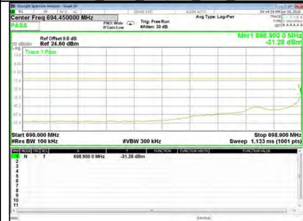
Band12_1.4M_16QAM_Low_Full-RB
