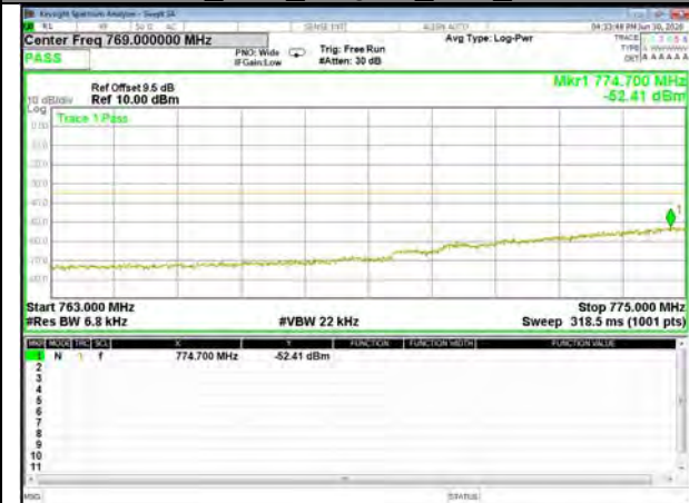
Band13_10M_16QAM_High_1-RB
