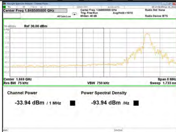
Band25_20M_QPSK_Low_Full-RB
