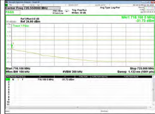
Band12_1.4M_16QAM_Low_1-RB
