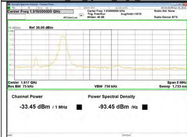
Band25_3M_QPSK_High_Full-RB
