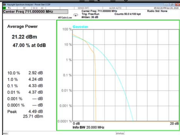
Band12_1_Q16_High
