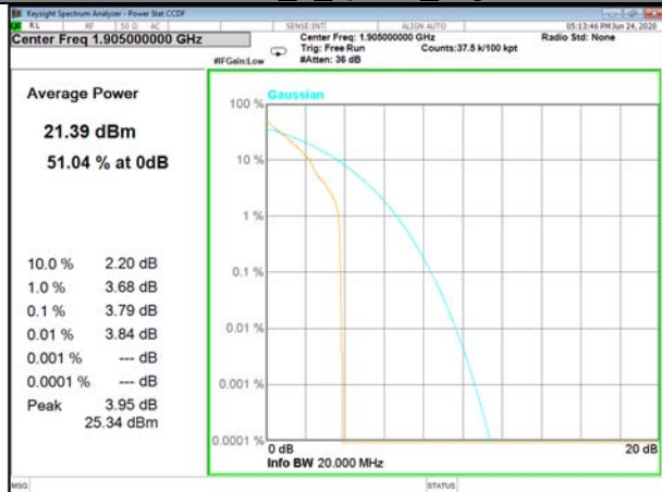
Band25_1_Q16_High
