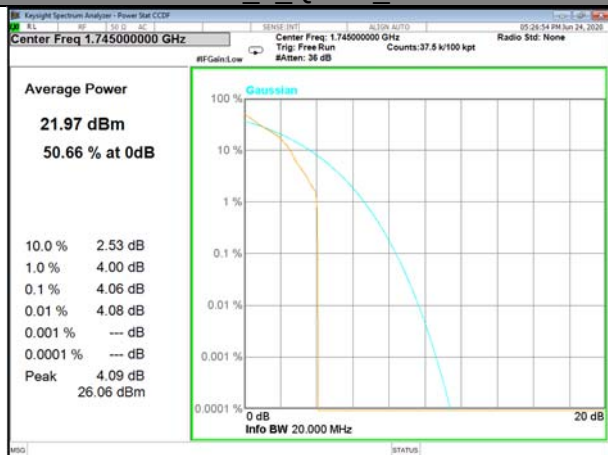
Band66_1_QPSK_Middle
