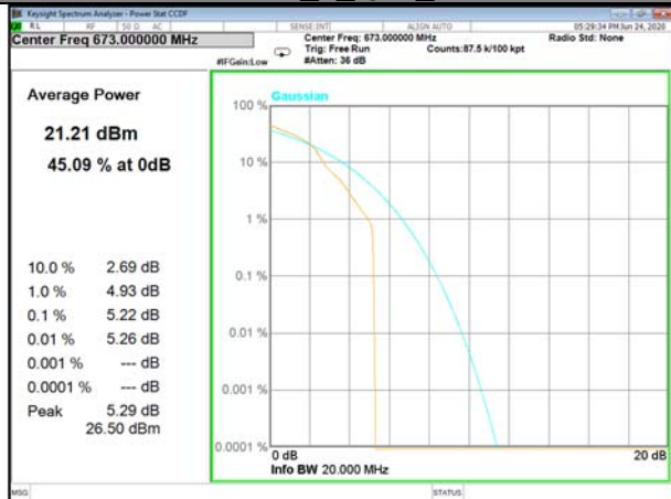
Band71_1_QPSK_Middle
