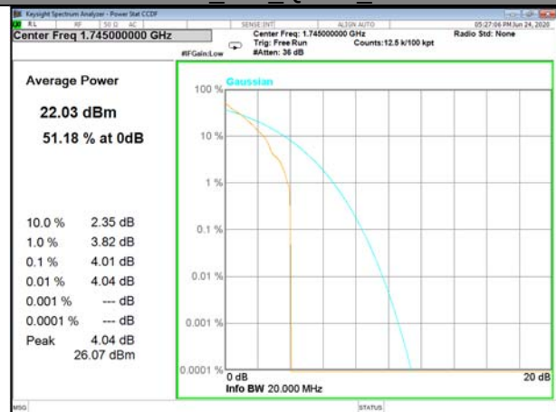
Band66_100_QPSK_Middle
