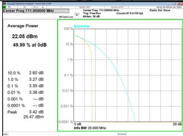
Band12_1_Q16_High
