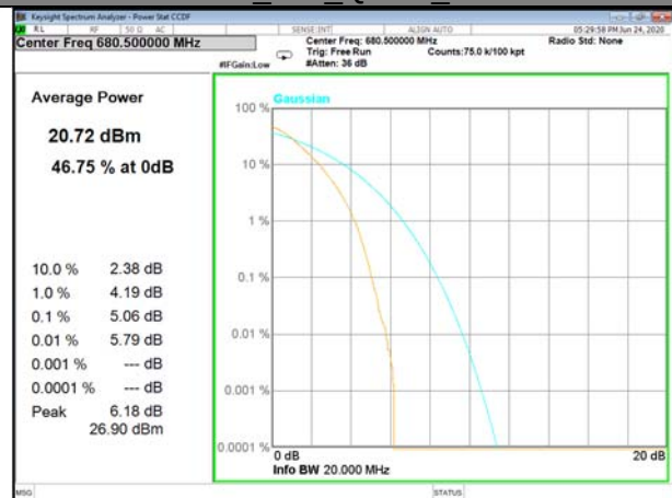
Band71_100_QPSK_Middle
