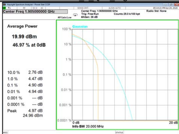
Band25_1_Q16_High
