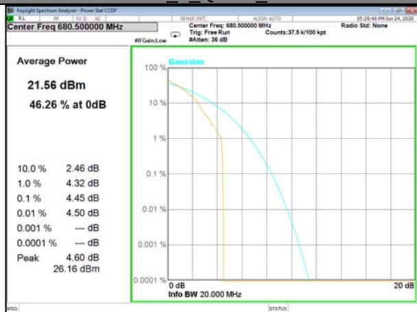
Band71_1_QPSK_Middle
