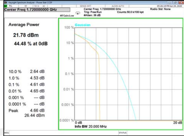
Band66_100_Q16_Low
