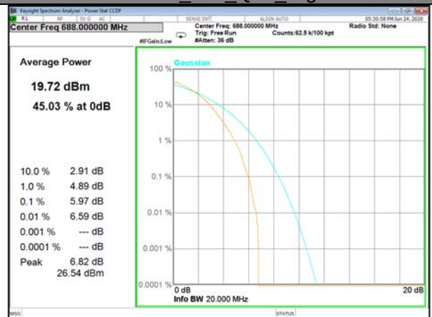
Band71_100_Q16_High
