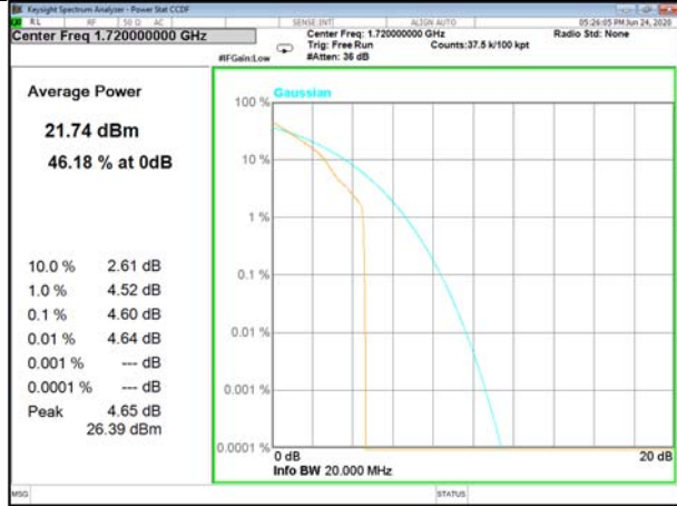
Band66_1_Q16_Low
