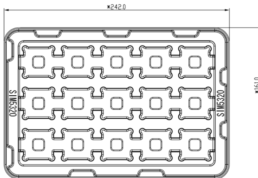
Figure 314: Tray drawing
