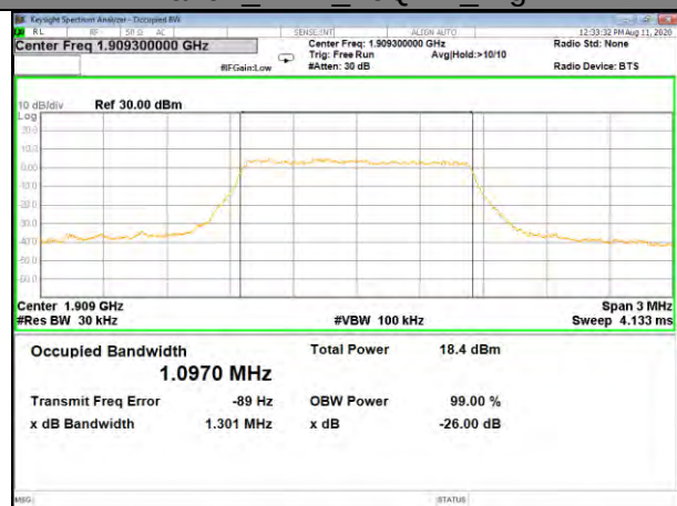
Band2_1.4M_16QAM_High
