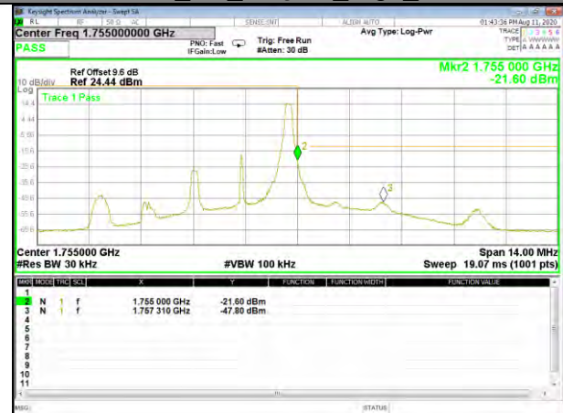
Band4_3M_16QAM_High_1-RB
