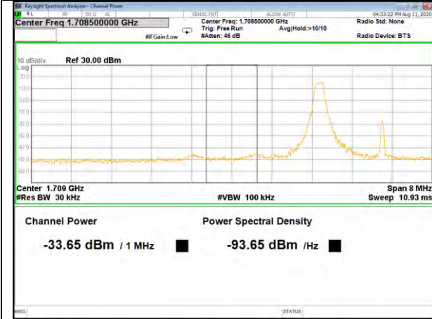
Band4_3M_16QAM_Low_Full-RB
