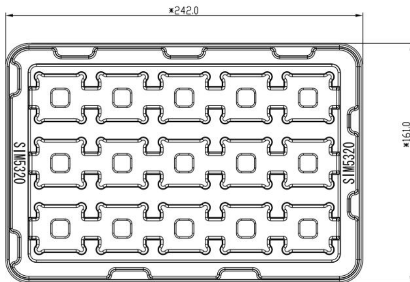
Figure 44: Tray drawing
