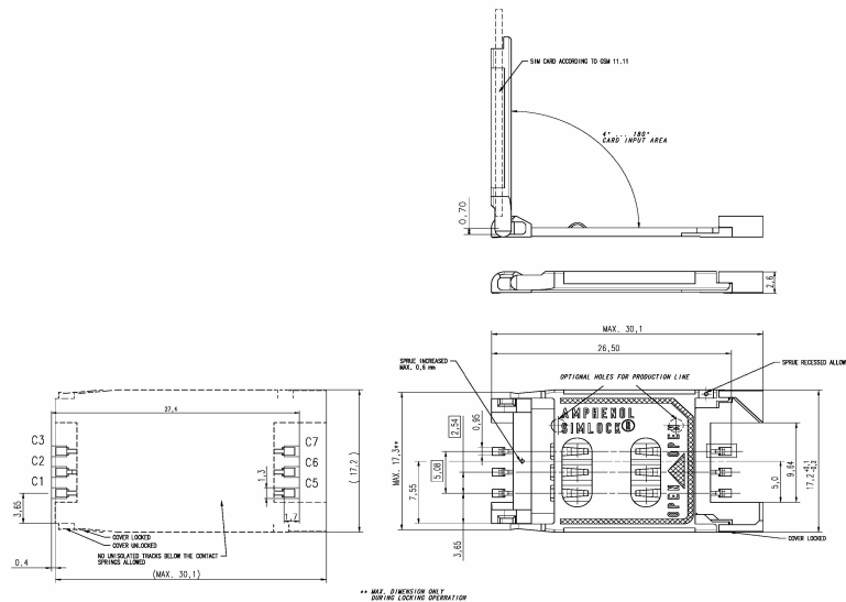
Figure 20: Amphenol SIM card socket
