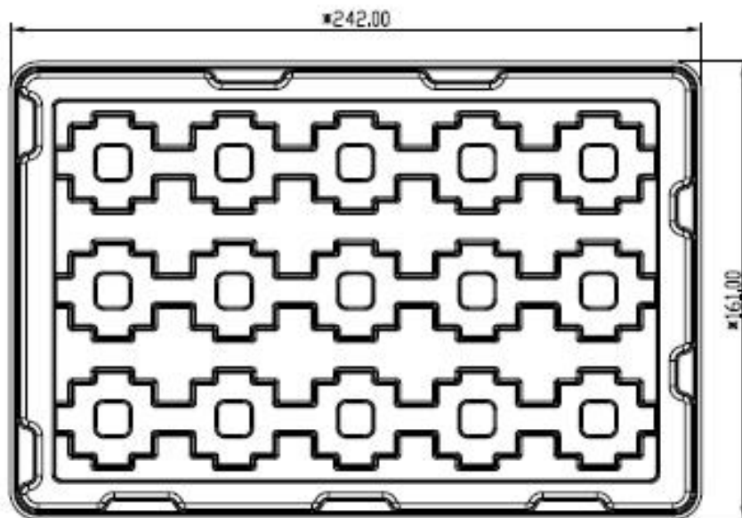
Figure 37: Tray drawing
