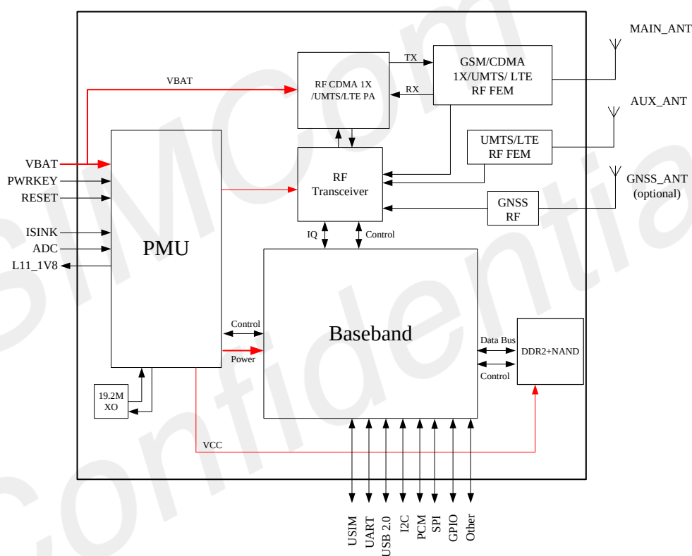
Figure 1: SIM7500V Block Diagram
