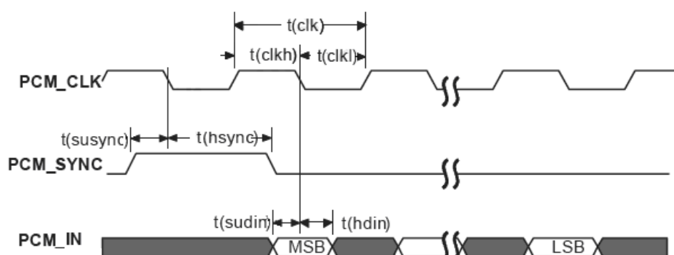
Figure 21: PCM_SYNC timing
