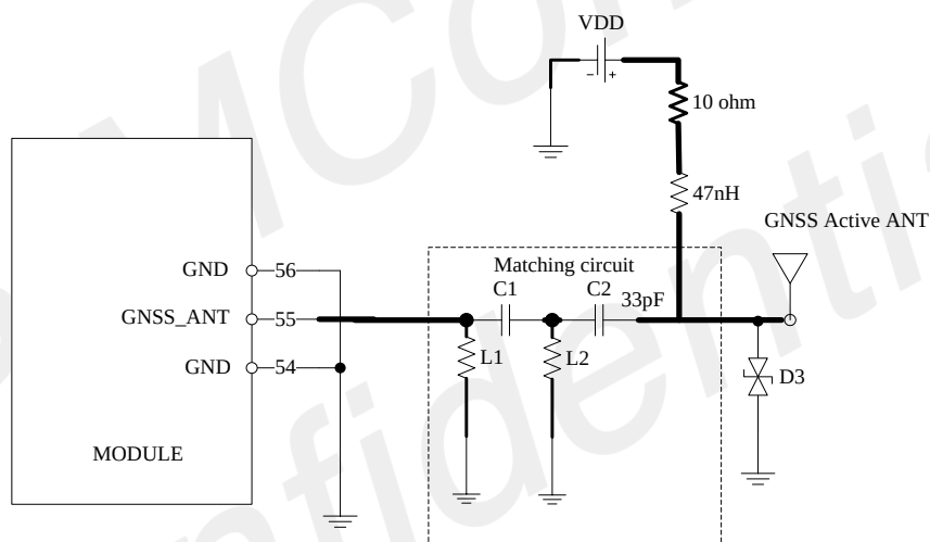
Figure 31: Active antenna circuit
