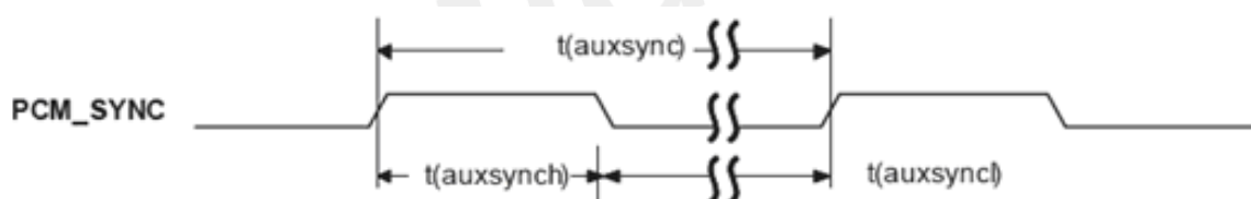
Figure 21: PCM_SYNC timing
