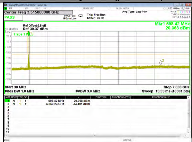
B71_3.75K_1#0_QPSK_High_CDT_Spurious
