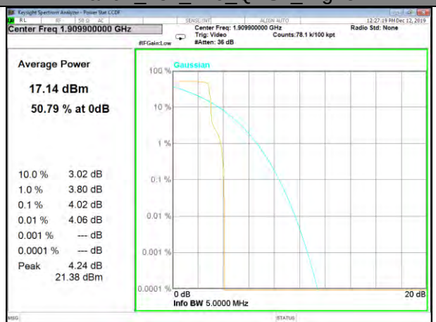
Band2_15k_1#0_QPSk_Higher
