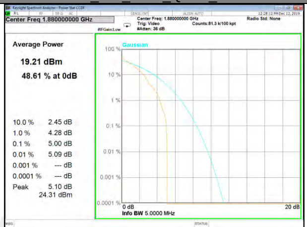
Band2_3.75k_1#0_QPSk_Middle
