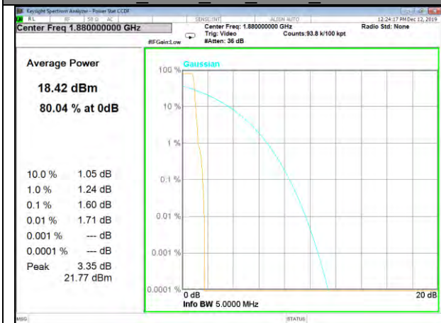
Band2_15k_1#0_BPSk_Higher
