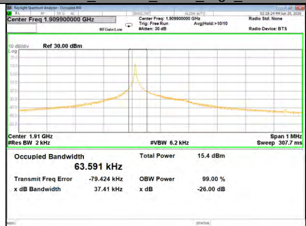
Band2_3.75kHz_BPSK_High_1#0
