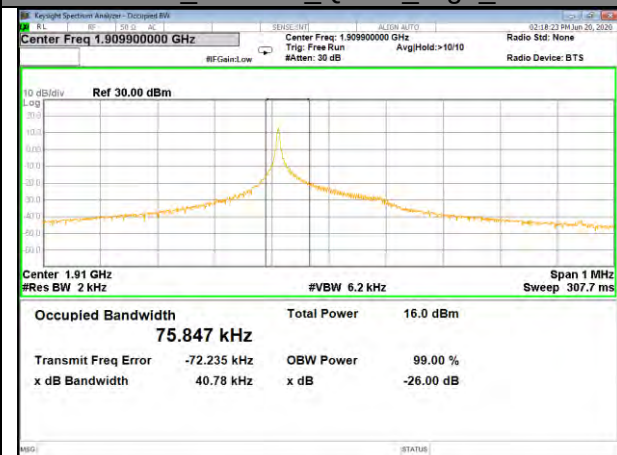
Band2_3.75kHz_QPSK_High_1#0
