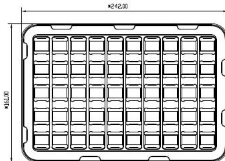
Figure 36: Tray drawing
