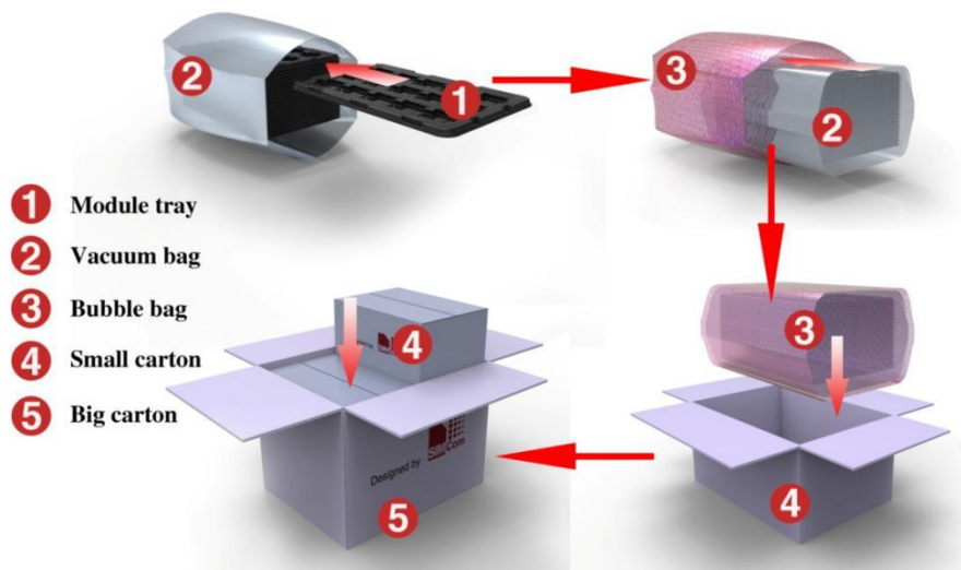
Figure 35: packaging diagram
