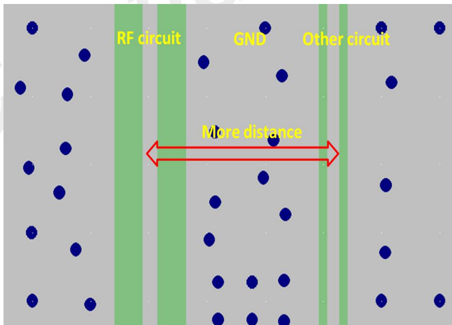
Figure 28: RF trace should be far away from other high speed signal lines
