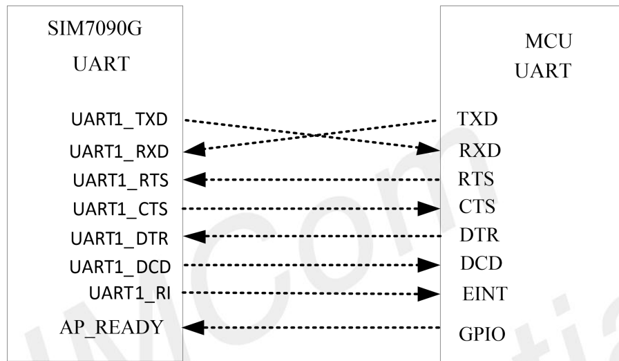
Figure 10: UART full modem
