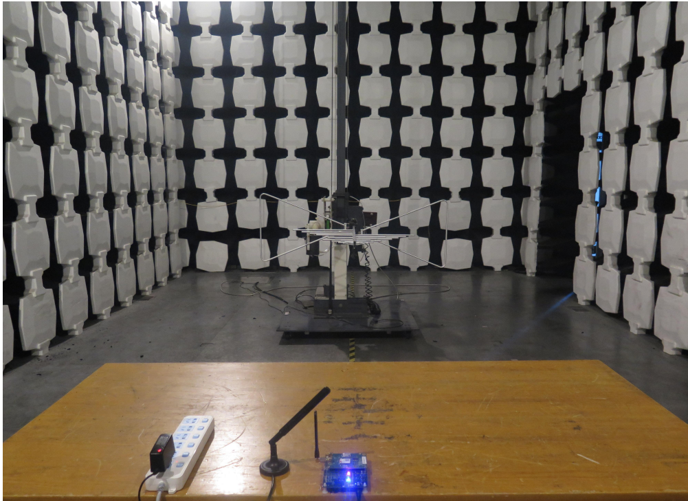
RSE (30MHz-1GHz)
