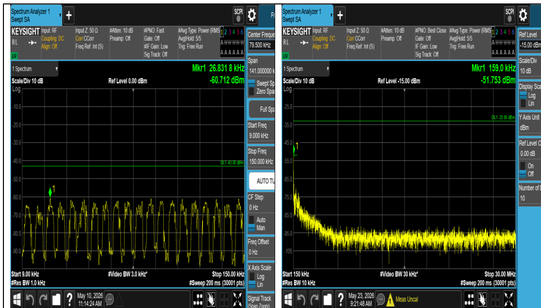
Band2-3MHz-QPSK-19185-1#5-0.009-0.15-PASS
