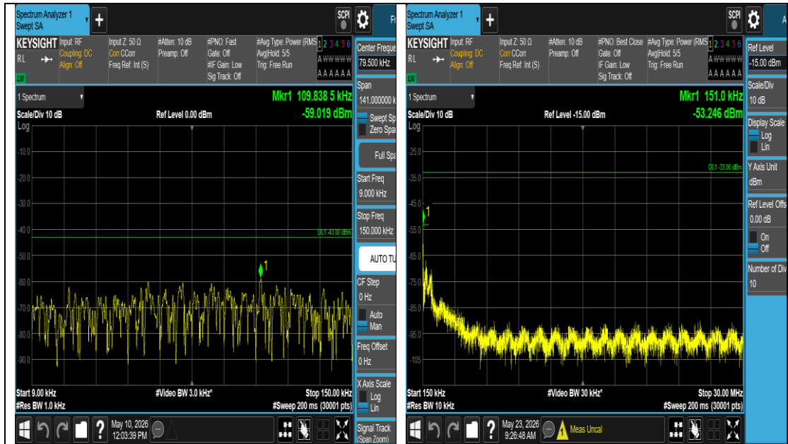
Band2-15MHz-QPSK-19125-1#5-0.009-0.15-PASS
