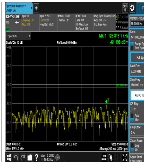
Band2-10MHz-QPSK-19150-1#5-0.009-0.15-PASS
