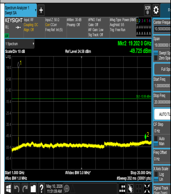
Band2-10MHz-QPSK-19150-1#5-1000-20000-PASS
