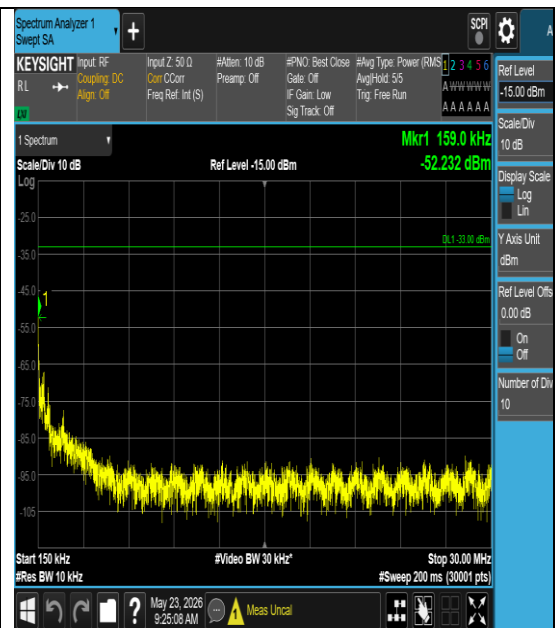
Band2-10MHz-QPSK-19150-1#5-0.15-30-PASS
