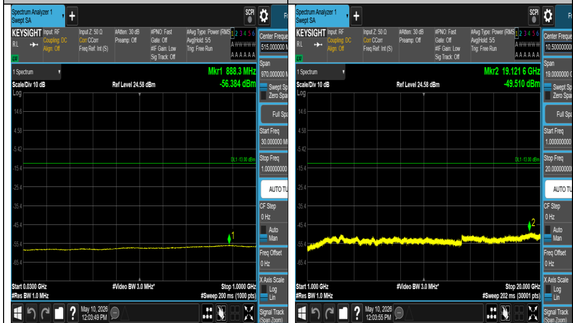
Band2-15MHz-QPSK-19125-1#5-30-1000-PASS
