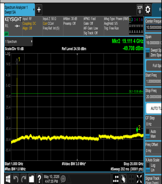
Band25-15MHz-QPSK-26115-1#0-1000-20000- PASS
