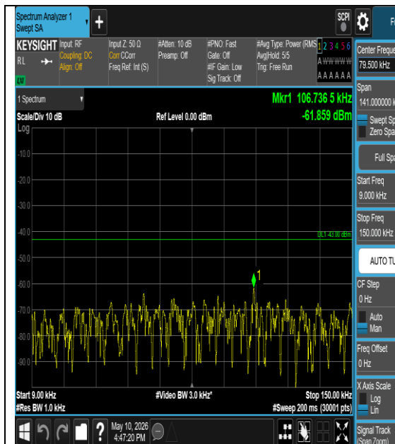
Band25-15MHz-QPSK-26115-1#0-0.009-0.15- PASS
