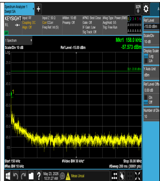
Band25-15MHz-QPSK-26115-1#0-0.15-30-PASS
