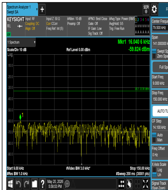
Band26(814-824)-5MHz-16QAM-26785-1#5- 0.009-0.15-PASS
