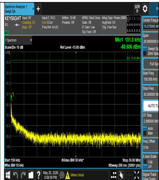
Band26(814-824)-5MHz-16QAM-26715-1#0- 0.15-30-PASS
