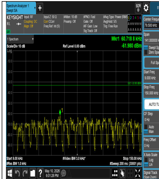
Band26(814-824)-10MHz-QPSK-26740-1#0- 0.009-0.15-PASS
