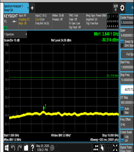
Band26(814-824)-5MHz-16QAM-26715-1#0- 1000-10000-PASS
