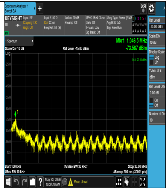
Band26(814-824)-3MHz-QPSK-26705-1#0-0.15- 30-PASS
