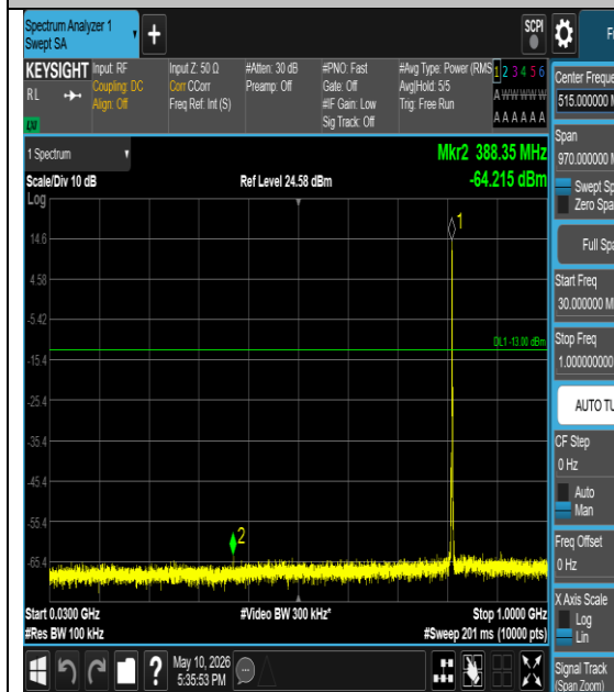
Band26(814-824)-3MHz-QPSK-26705-1#0-30- 1000-PASS
