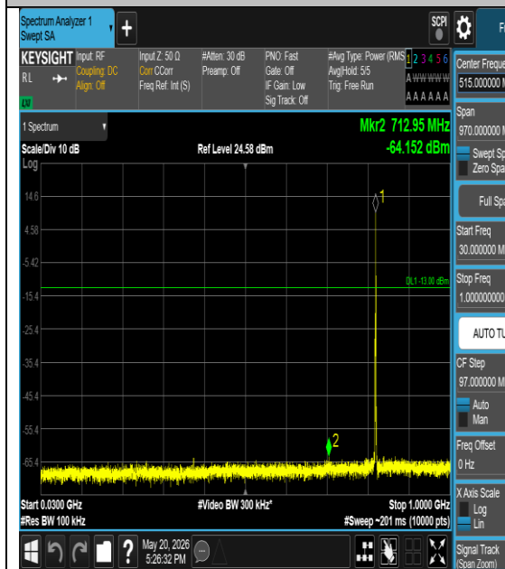
Band26(814-824)-1.4MHz-16QAM-26783-1#5- 30-1000-PASS
