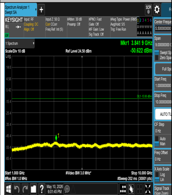
Band26(814-824)-10MHz-QPSK-26740-1#0- 1000-10000-PASS
