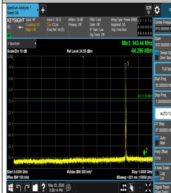
Band26(814-824)-5MHz-16QAM-26715-1#0-30- 1000-PASS
