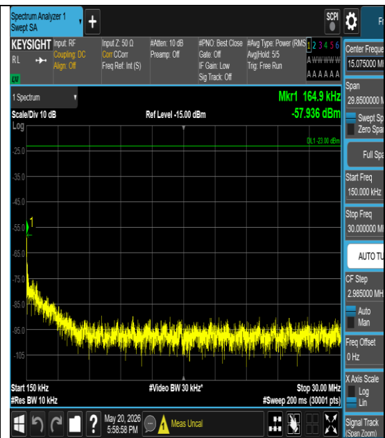
Band26(814-824)-5MHz-16QAM-26785-1#5- 0.15-30-PASS
