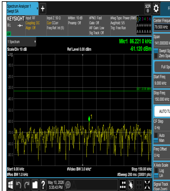
Band26(814-824)-3MHz-QPSK-26705-1#0- 0.009-0.15-PASS
