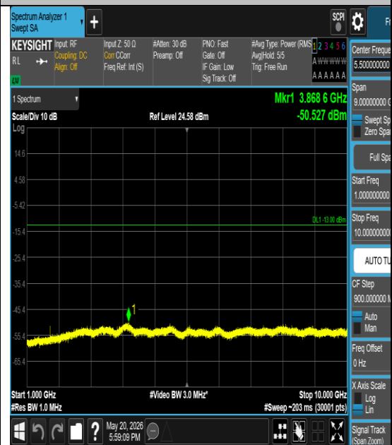
Band26(814-824)-5MHz-16QAM-26785-1#5- 1000-10000-PASS
