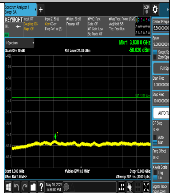
Band26(814-824)-3MHz-QPSK-26705-1#0- 1000-10000-PASS
