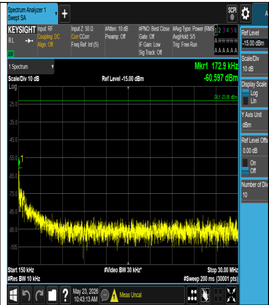
Band26(814-824)-10MHz-QPSK-26740-1#0- 0.15-30-PASS
