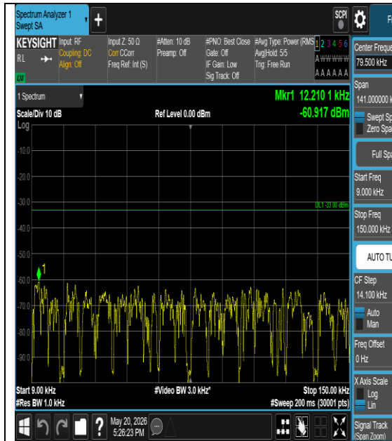
Band26(814-824)-1.4MHz-16QAM-26783-1#5- 0.009-0.15-PASS
