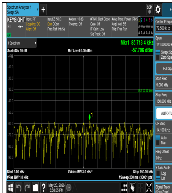
Band26(814-824)-5MHz-16QAM-26715-1#0- 0.009-0.15-PASS
