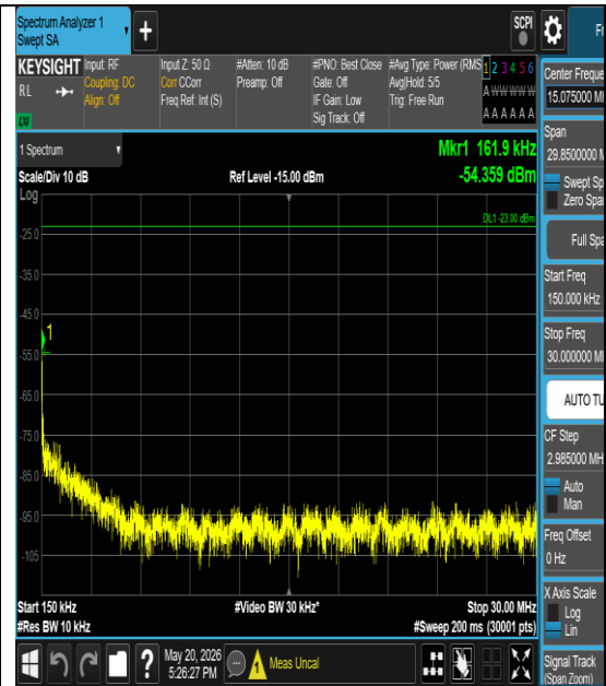
Band26(814-824)-1.4MHz-16QAM-26783-1#5- 0.15-30-PASS
