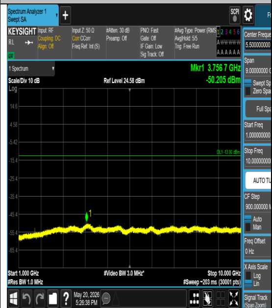
Band26(814-824)-1.4MHz-16QAM-26783-1#5- 1000-10000-PASS
