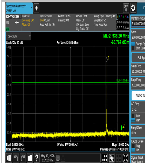
Band26(814-824)-10MHz-QPSK-26740-1#0-30- 1000-PASS
