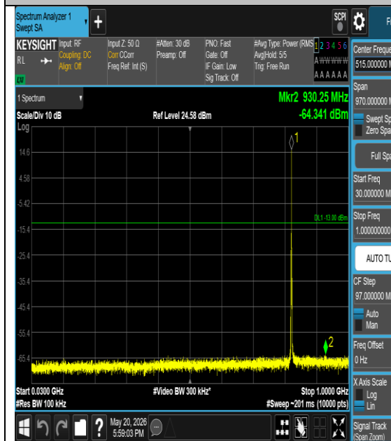
Band26(814-824)-5MHz-16QAM-26785-1#5-30- 1000-PASS
