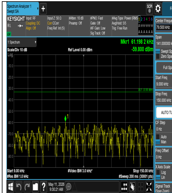
Band26(824-849)-5MHz-QPSK-26815-1#0- 0.009-0.15-PASS
