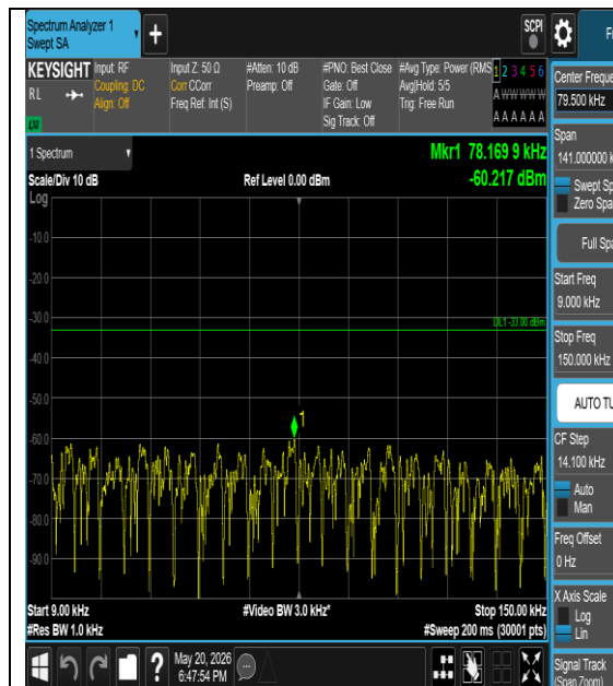
Band26(824-849)-3MHz-16QAM-27025-1#5- 0.009-0.15-PASS
