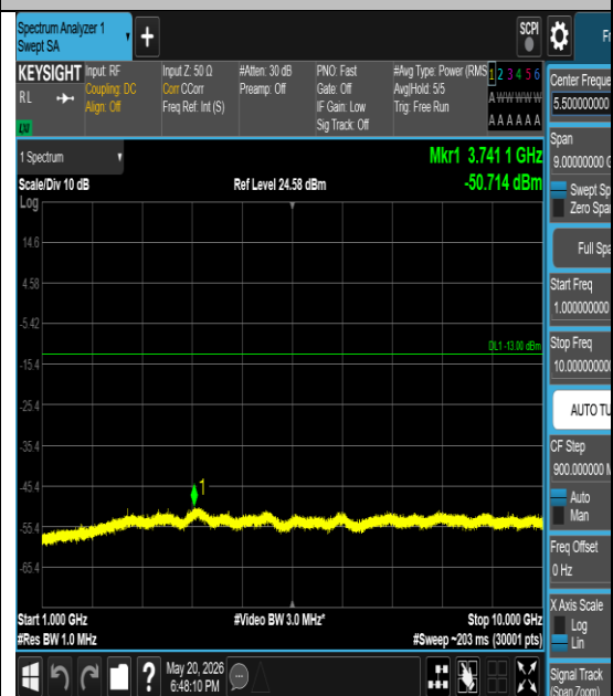
Band26(824-849)-3MHz-16QAM-27025-1#5- 1000-10000-PASS
