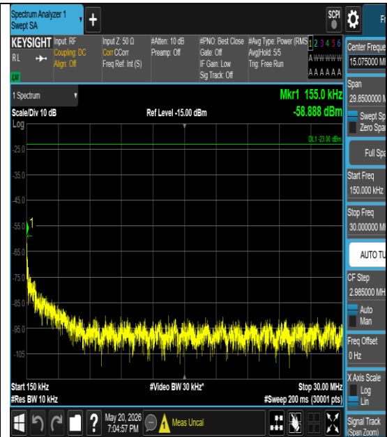
Band26(824-849)-5MHz-16QAM-27015-1#5- 0.15-30-PASS
