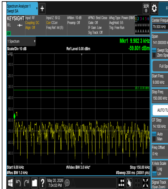
Band26(824-849)-5MHz-16QAM-27015-1#5- 0.009-0.15-PASS
