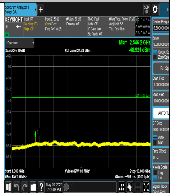
Band26(824-849)-5MHz-16QAM-27015-1#5- 1000-10000-PASS
