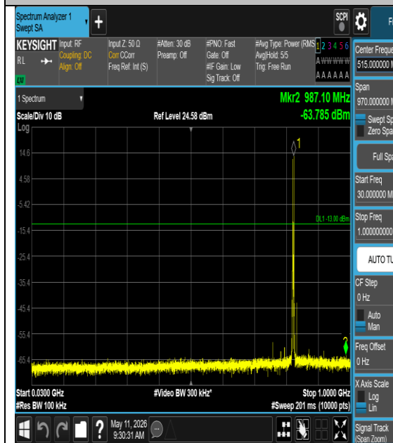
Band26(824-849)-5MHz-QPSK-26815-1#0-30- 1000-PASS
