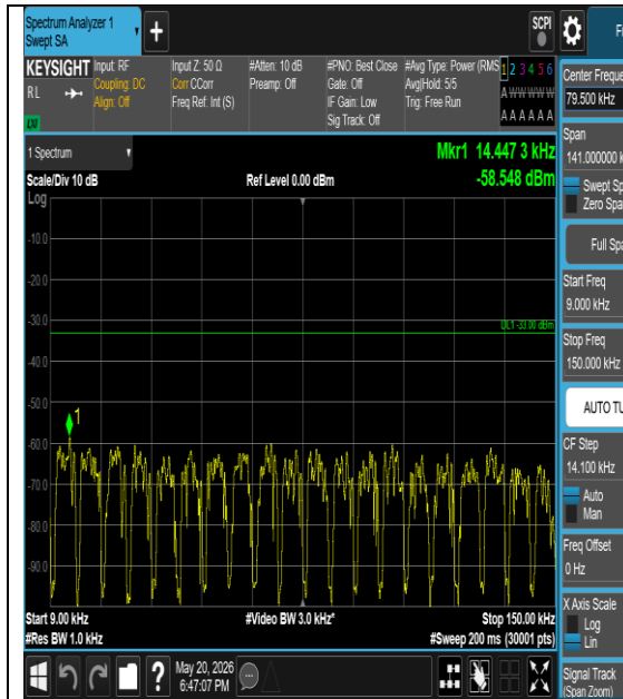
Band26(824-849)-3MHz-16QAM-26805-1#0- 0.009-0.15-PASS
