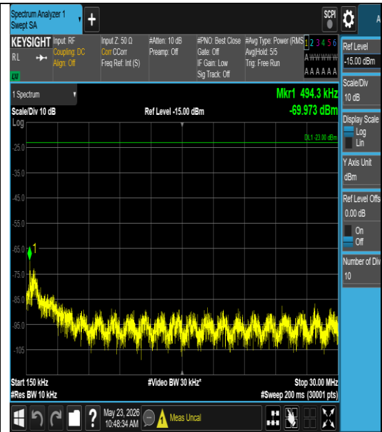
Band26(824-849)-5MHz-QPSK-26815-1#0-0.15- 30-PASS
