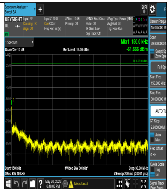
Band26(824-849)-3MHz-16QAM-27025-1#5- 0.15-30-PASS
