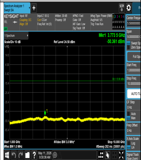
Band26(824-849)-5MHz-QPSK-26815-1#0- 1000-10000-PASS
