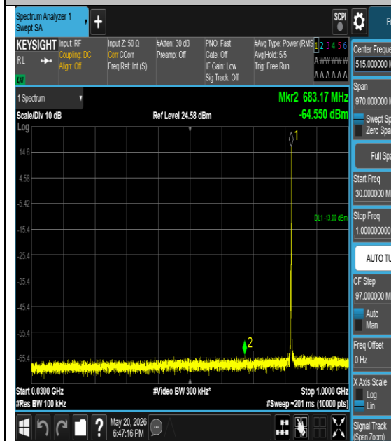
Band26(824-849)-3MHz-16QAM-26805-1#0-30- 1000-PASS
