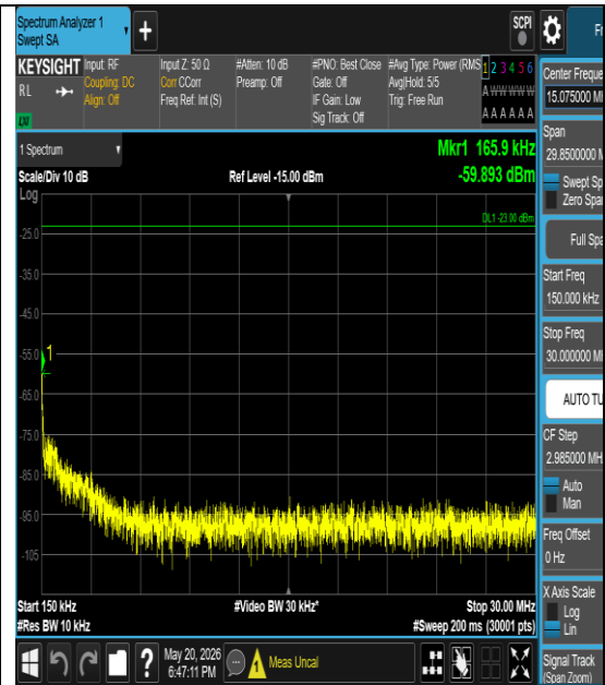
Band26(824-849)-3MHz-16QAM-26805-1#0- 0.15-30-PASS
