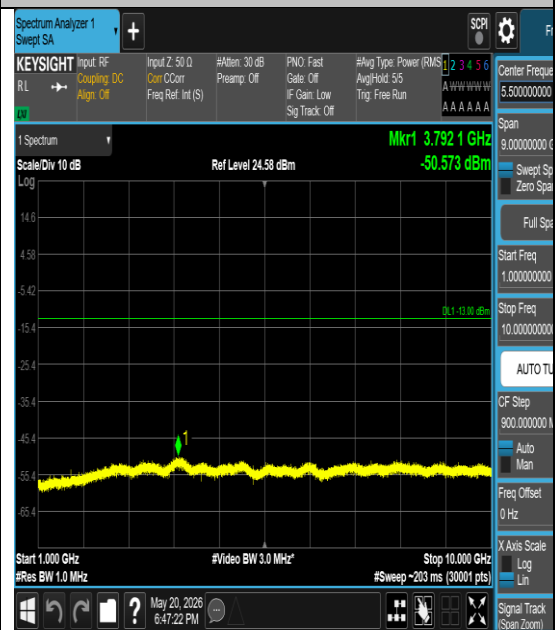
Band26(824-849)-3MHz-16QAM-26805-1#0- 1000-10000-PASS
