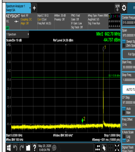
Band26(824-849)-3MHz-16QAM-27025-1#5-30- 1000-PASS
