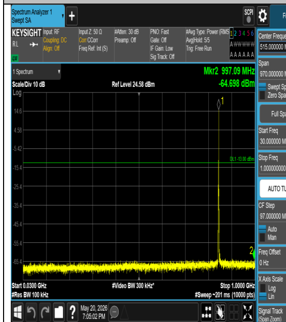
Band26(824-849)-5MHz-16QAM-27015-1#5-30- 1000-PASS
