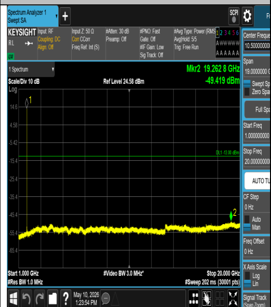
Band4-10MHz-QPSK-20000-1#0-1000-20000-PASS
