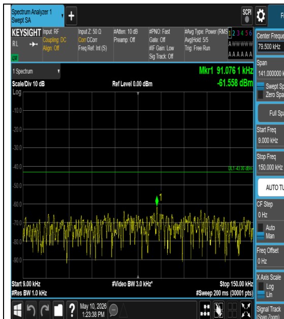
Band4-10MHz-QPSK-20000-1#0-0.009-0.15-PASS
