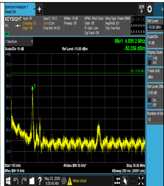
Band4-10MHz-QPSK-20000-1#0-0.15-30-PASS
