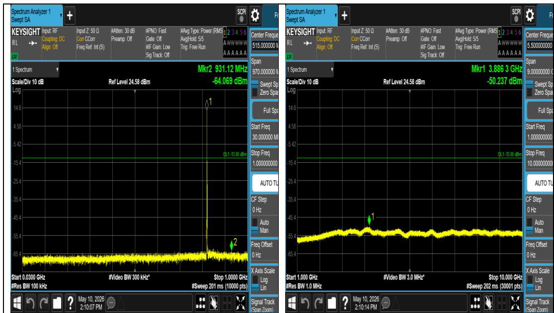
Band5-3MHz-QPSK-20415-1#0-1000-10000-PASS
