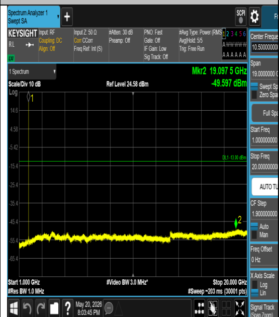
Band66-1.4MHz-16QAM-132665-1#5-1000-20000-PASS
