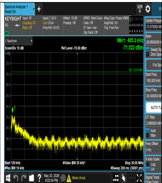
Band66-1.4MHz-16QAM-132665-1#5-0.15-30-PASS
