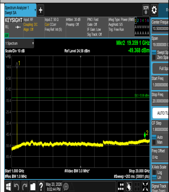
Band66-1.4MHz-16QAM-132322-1#0-1000-20000-PASS
