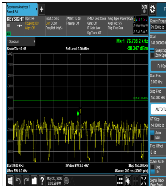
Band66-1.4MHz-16QAM-132665-1#5-0.009-0.15-PASS
