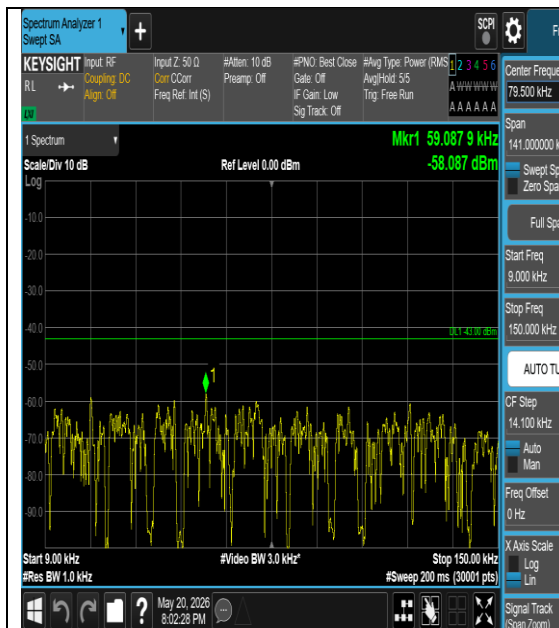
Band66-1.4MHz-16QAM-132322-1#0-0.009-0.15-PASS
