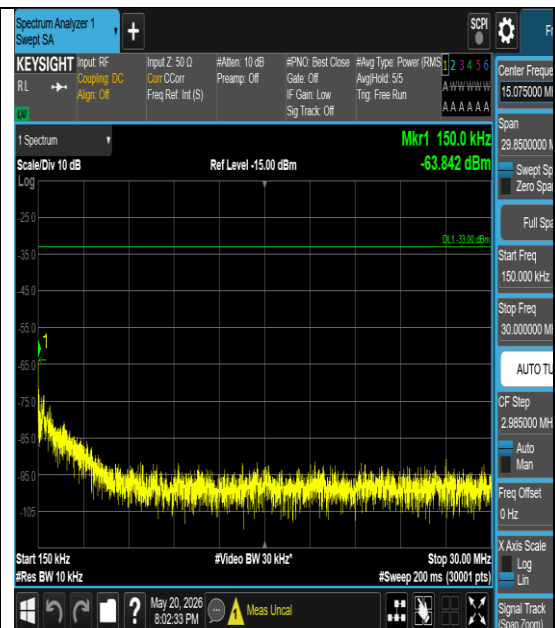
Band66-1.4MHz-16QAM-132322-1#0-0.15-30-PASS
