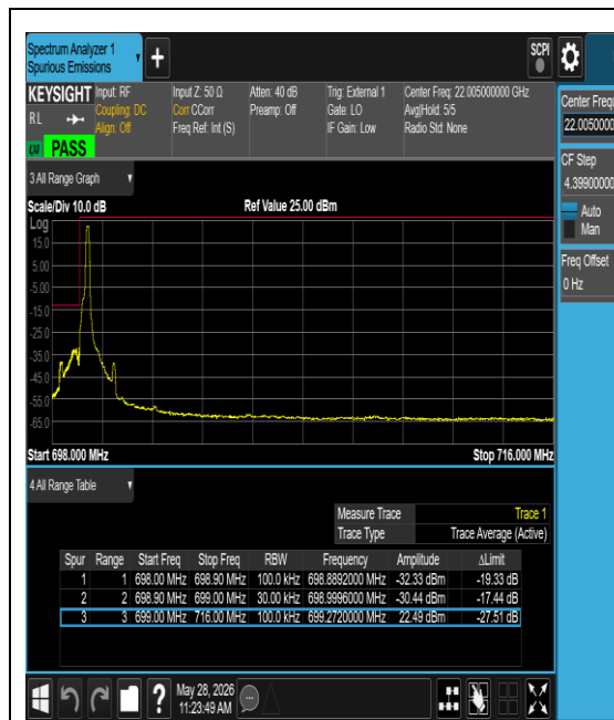
Band12-0.18-BPSK-23012-1@11-15kHz-PASS
