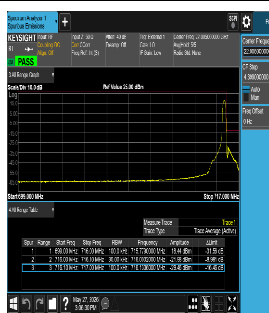
Band12-0.18-QPSK-23178-12@0-15kHz-PASS
