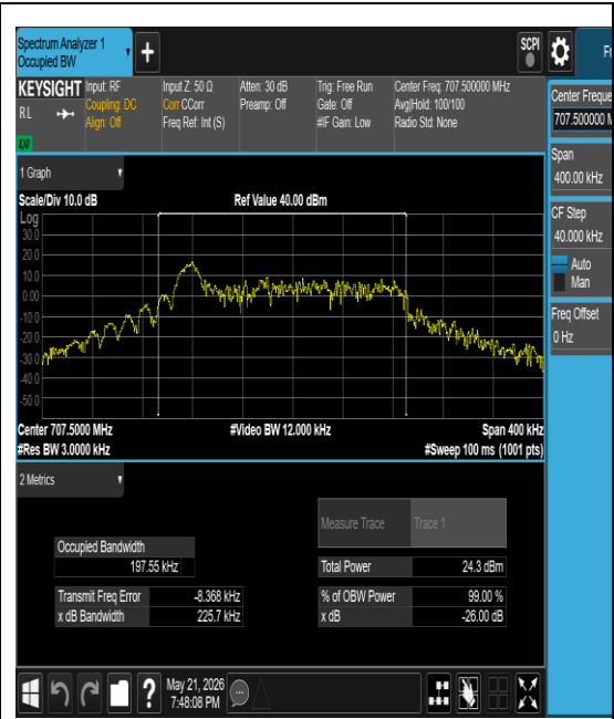
Band12-0.18-BPSK-23095-12@0-15kHz-PASS
