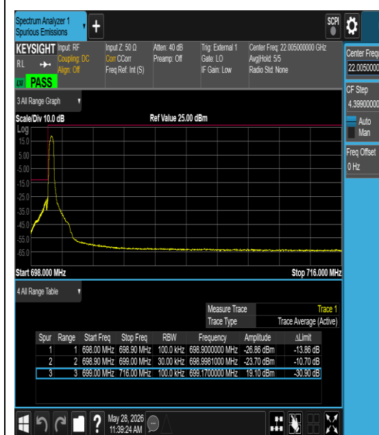
Band12-0.18-QPSK-23012-12@0-15kHz-PASS
