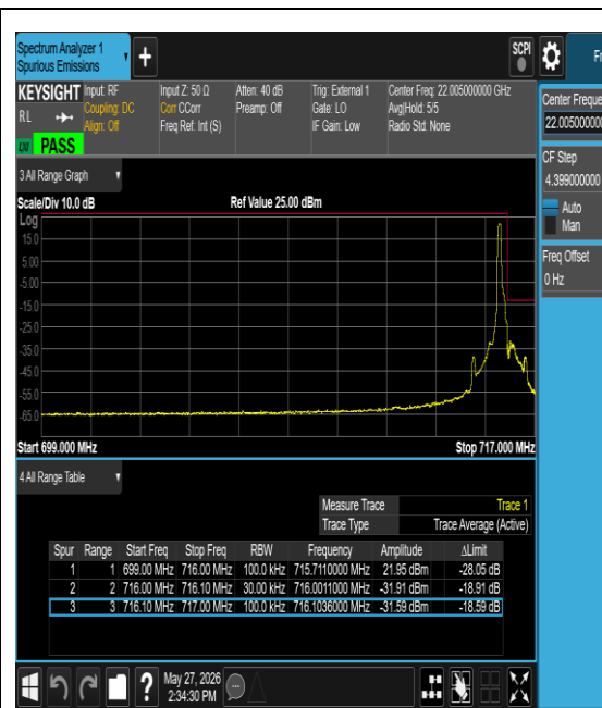
Band12-0.18-QPSK-23178-1@0-15kHz-PASS
