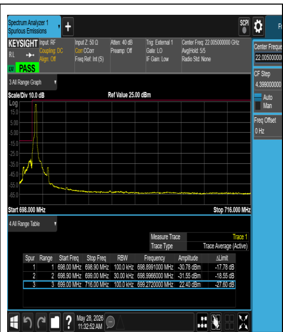
Band12-0.18-QPSK-23012-1@11-15kHz-PASS
