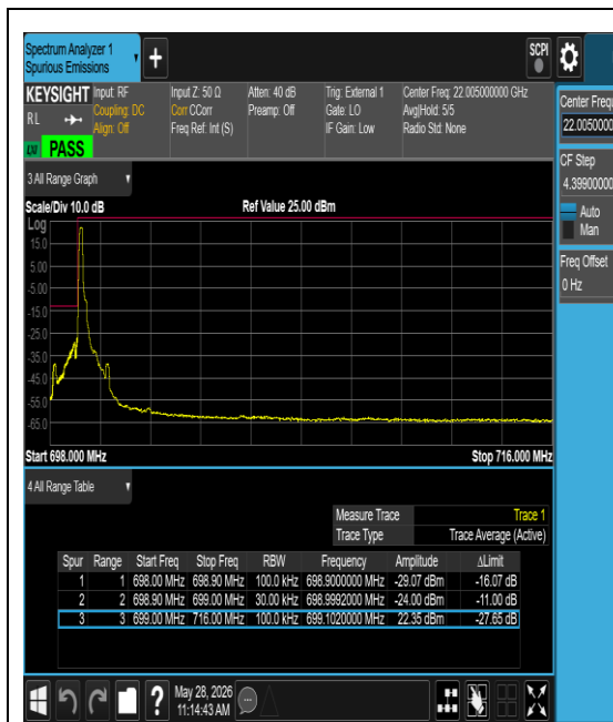
Band12-0.18-QPSK-23012-1@0-15kHz-PASS
