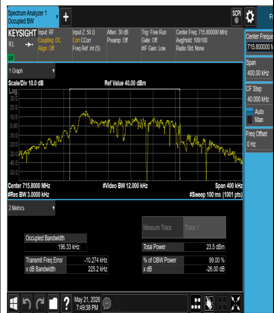
Band12-0.18-BPSK-23178-12@0-15kHz-PASS
