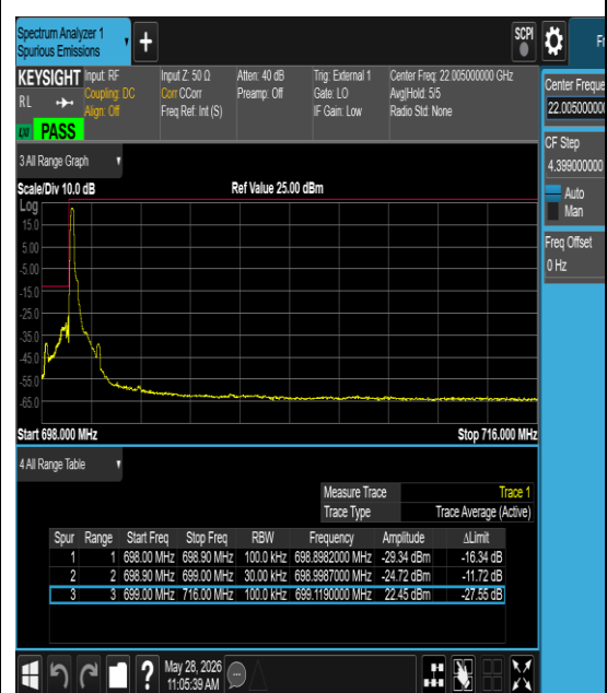
Band12-0.18-BPSK-23012-1@0-15kHz-PASS
