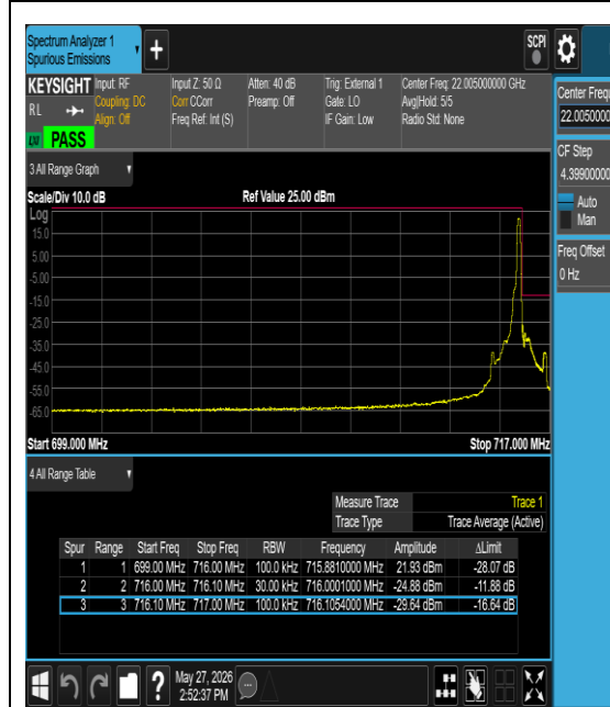
Band12-0.18-QPSK-23178-1@11-15kHz-PASS
