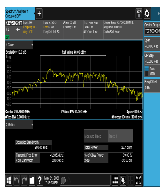
Band12-0.18-QPSK-23095-12@0-15kHz-PASS
