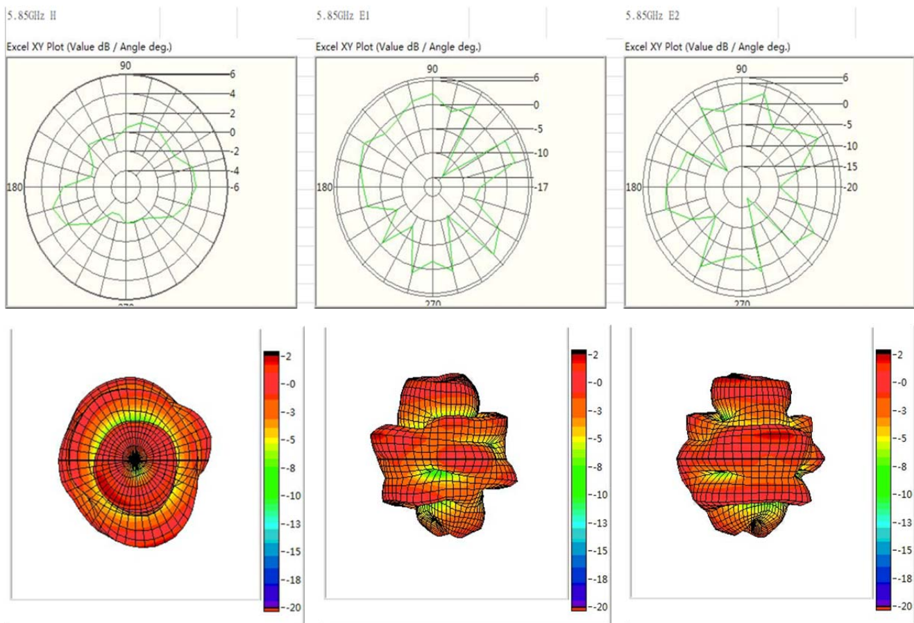
5.85G 2D&3D
