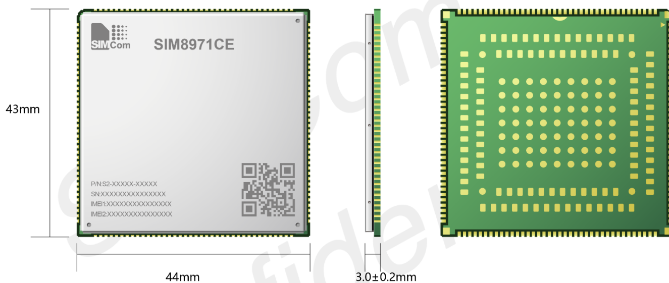
Figure 42: Top- and Bottom-View of the Module
