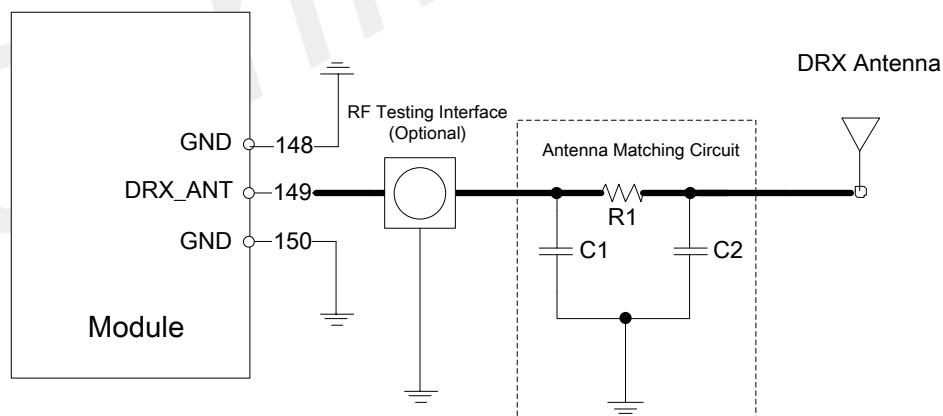
Figure 33: DRX Antenna Reference Design
