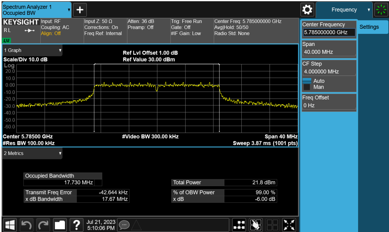
Figure 5: The plots of 6dB Bandwidth, 802.11n(HT20), 5785MHz
