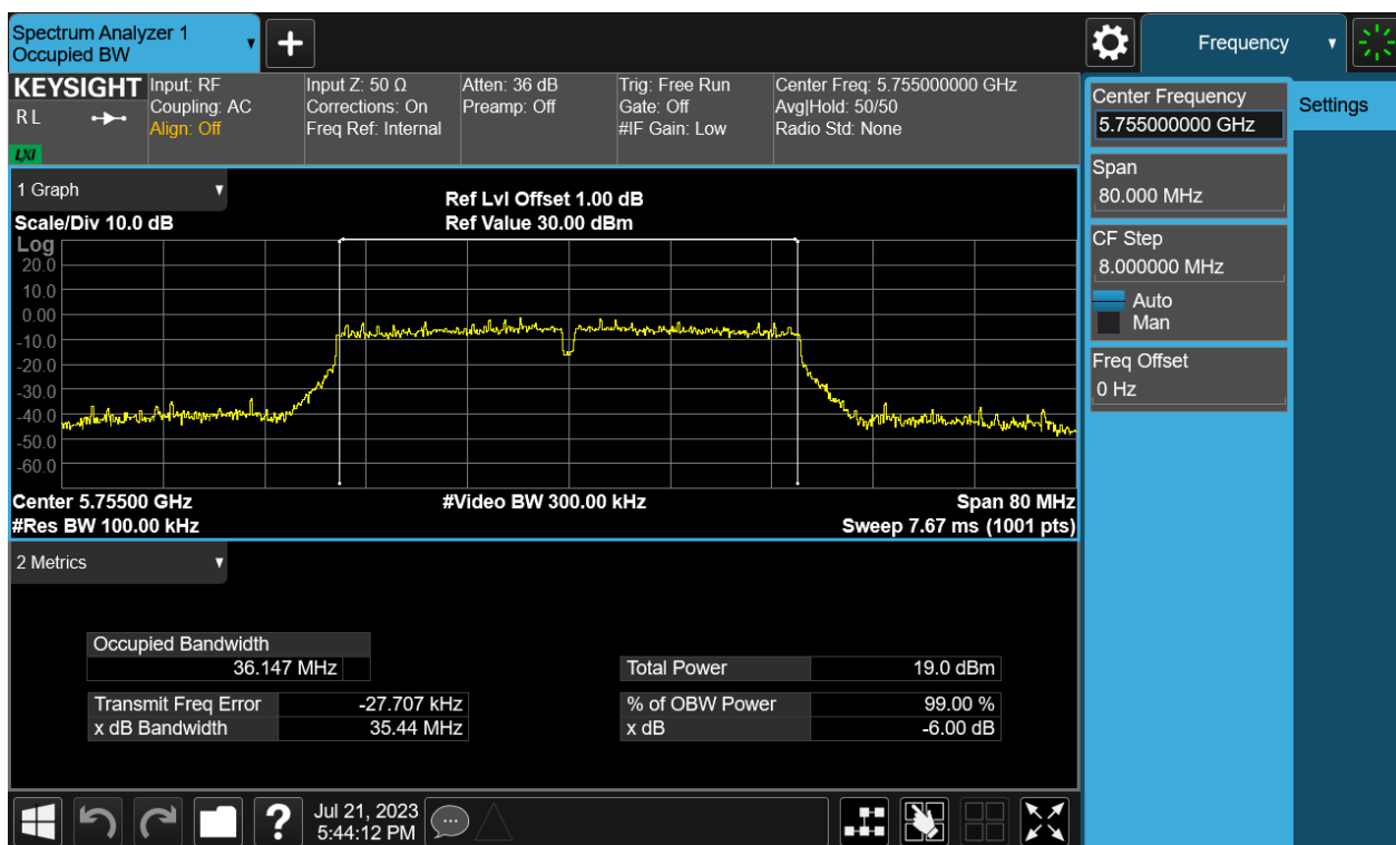
Figure 12: The plots of 6dB Bandwidth, 802.11ac(VHT40), 5755MHz
