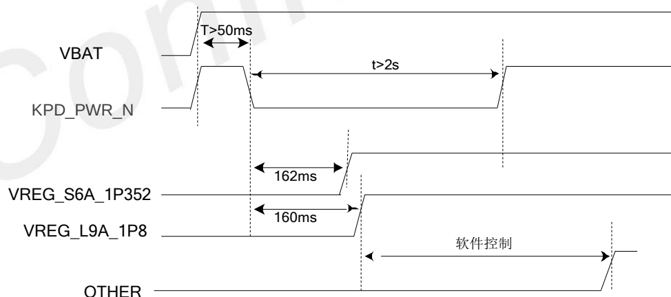
Figure 8: Power Sequence
