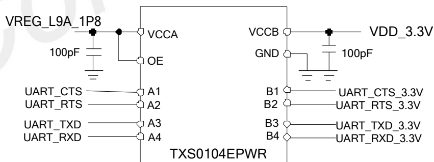
Figure 16: UART Voltage Level Shift Reference Design
