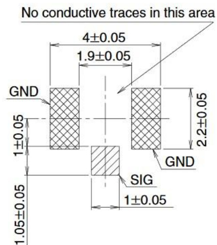
Figure 40: Hirose U.FL-R-SMT Connector's Size and Package
