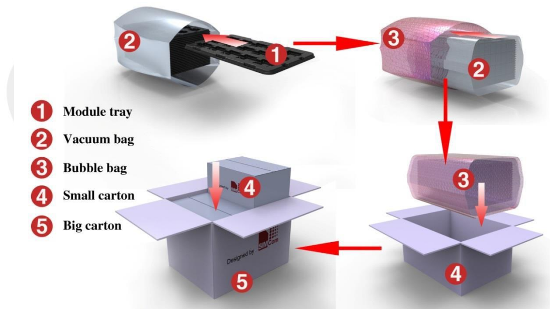
Figure 46: Packaging Diagram
