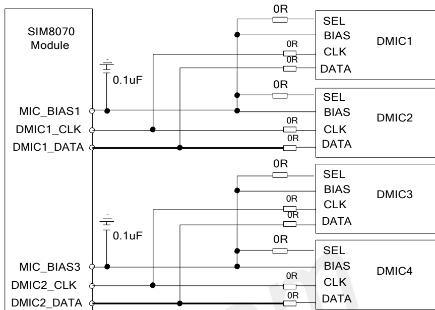
Figure 26: Digital Microphone Reference Design
