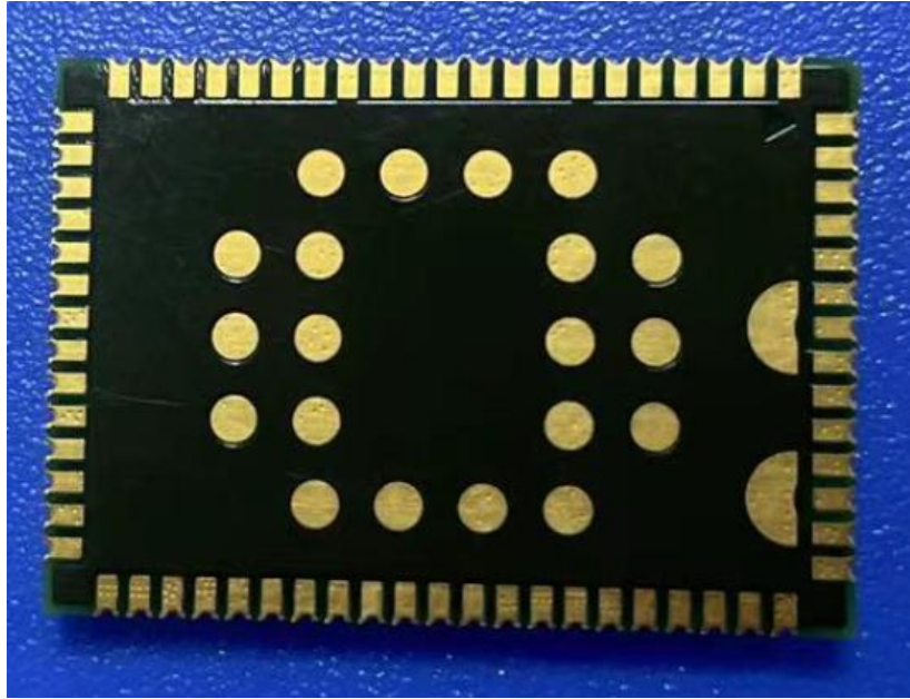
Pic3. EUT's Back
