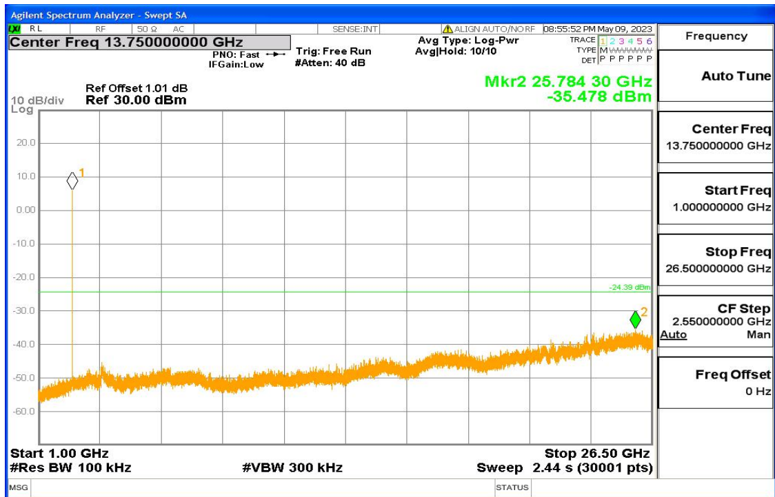
11b Fig3
