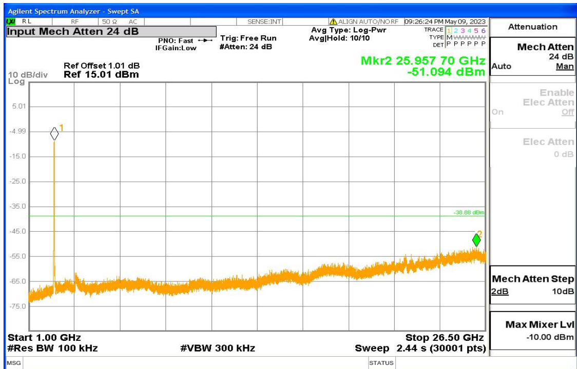
11n-HT40 Fig3
