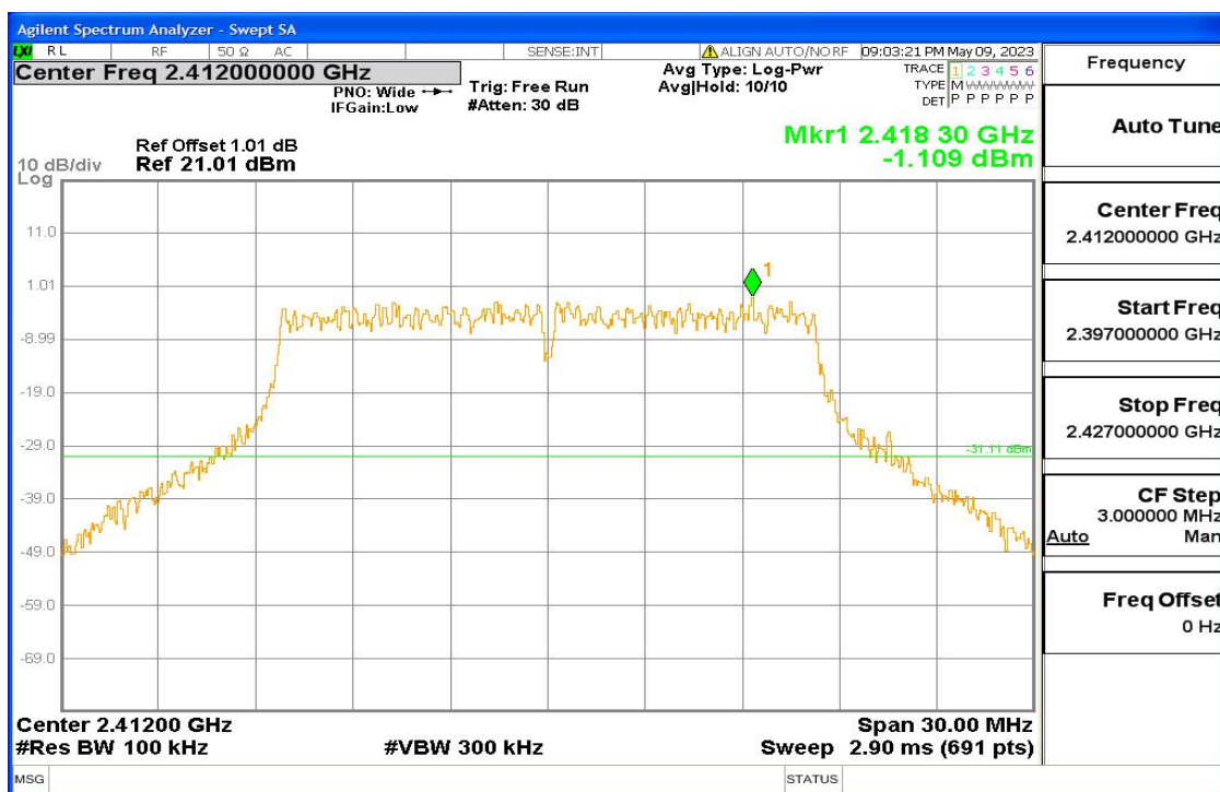
11g Fig1
