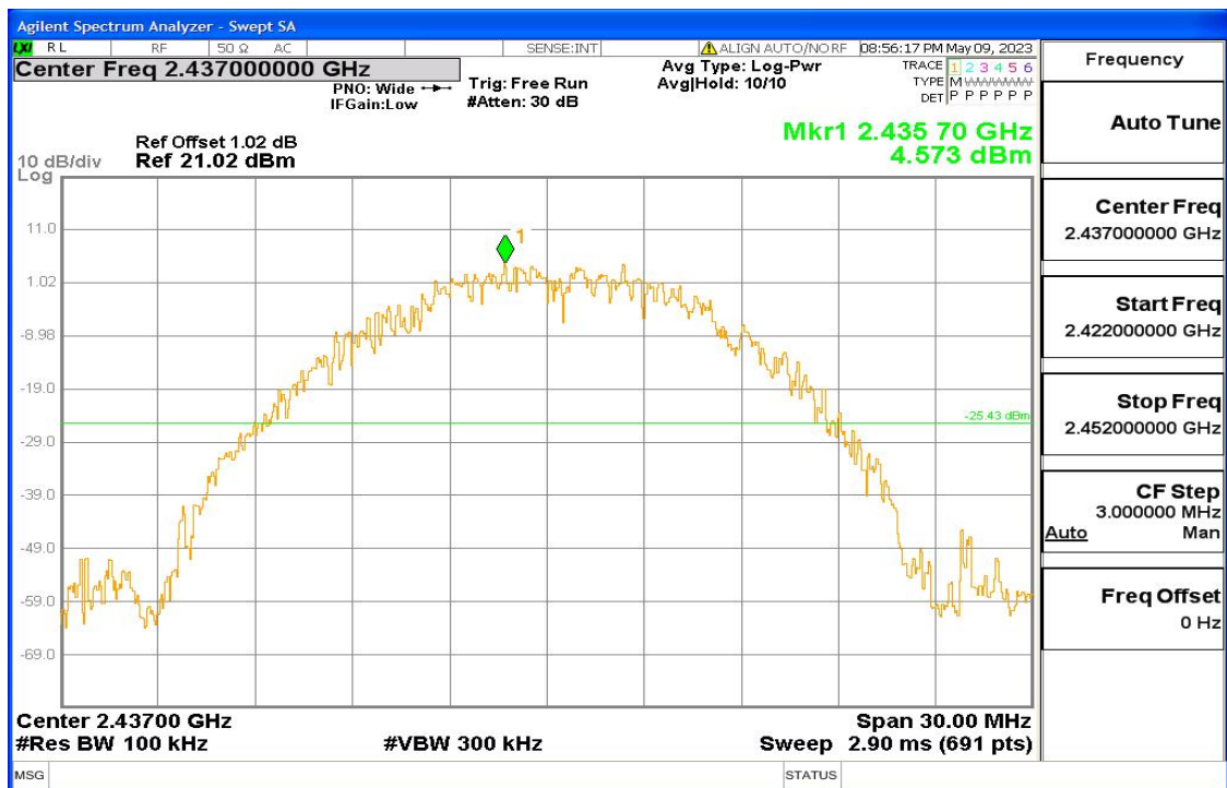
11b Fig4
