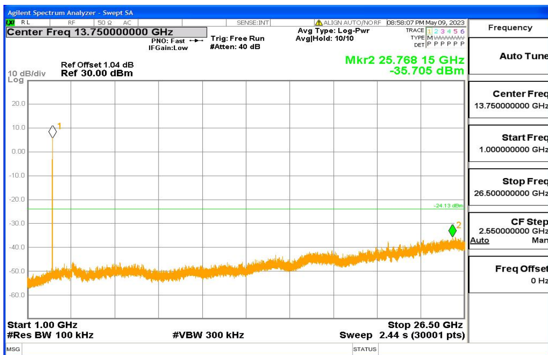
11b Fig9
