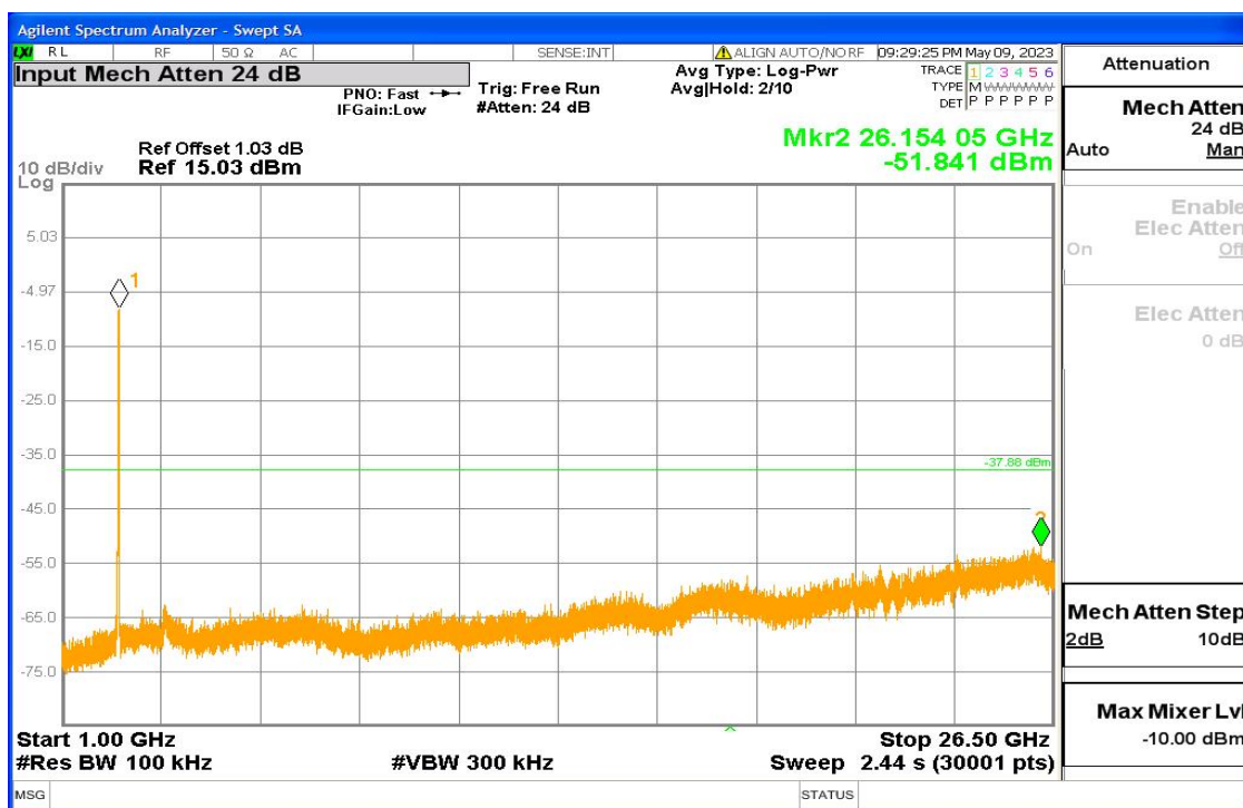
11n-HT40 Fig9
