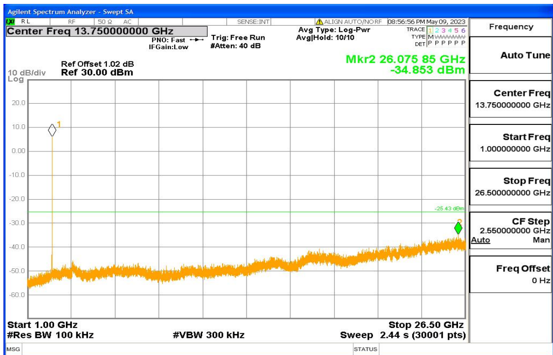
11b Fig6
