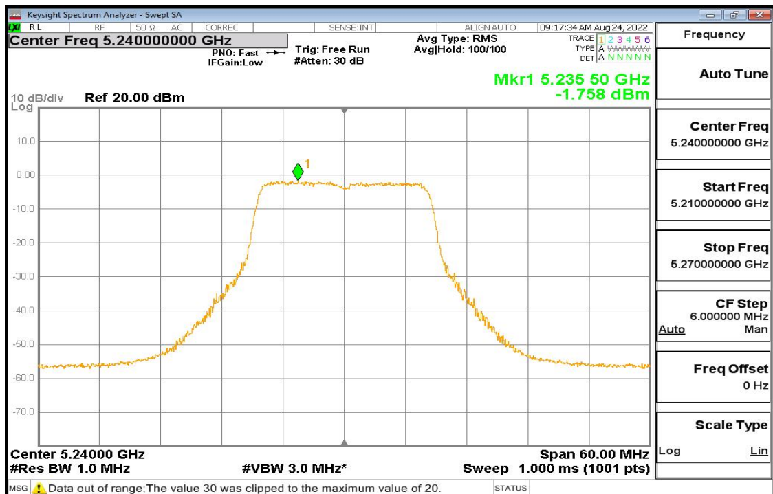
11a Pic3
