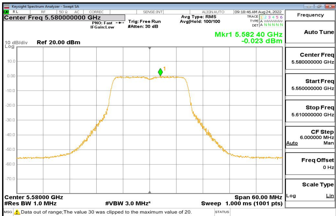
11a Pic8
