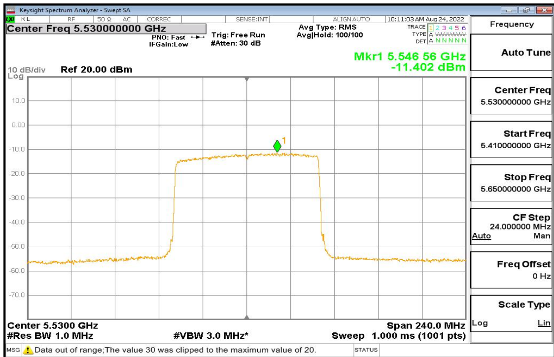
11ax-80 Pic3
