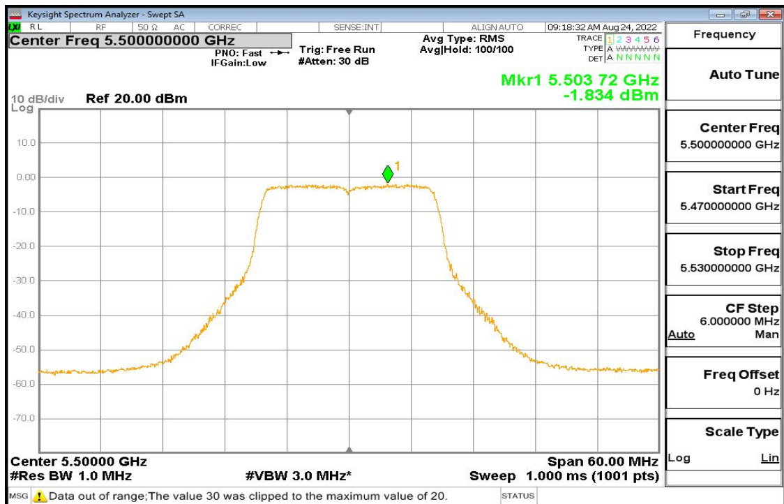
11a Pic7
