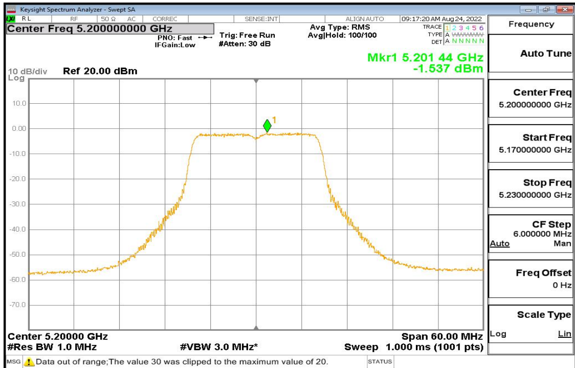
11a Pic2
