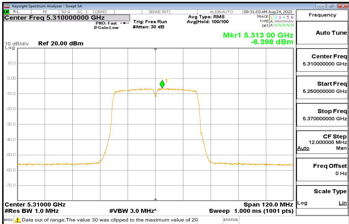
11n-40 Pic4
