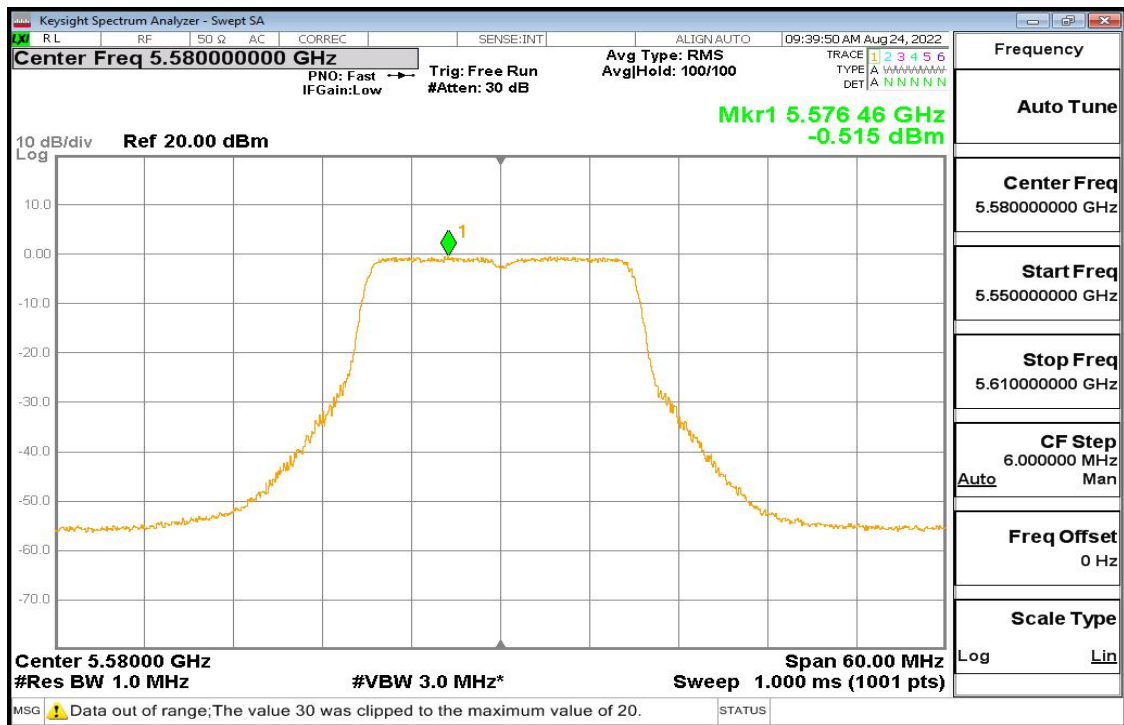
11ac-20 Pic8
