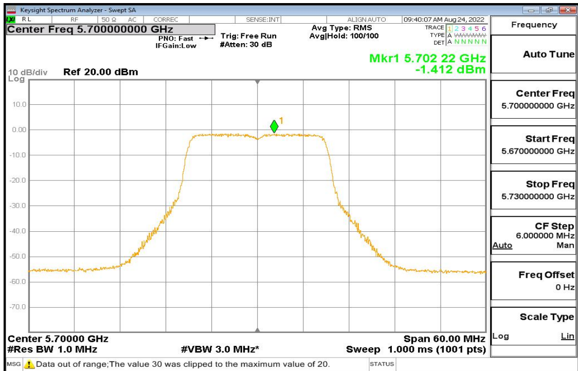
11ac-20 Pic9
