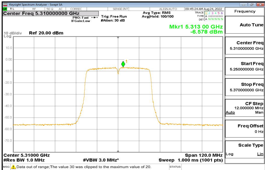
11ac-40 Pic4
