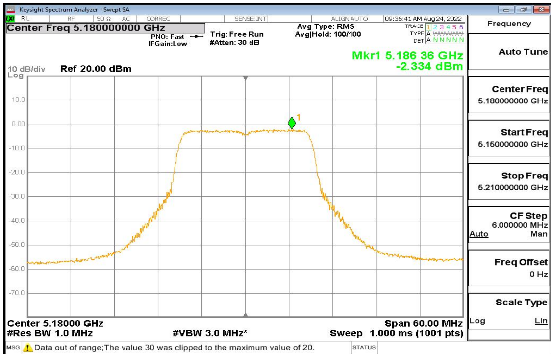
11ac-20 Pic1
