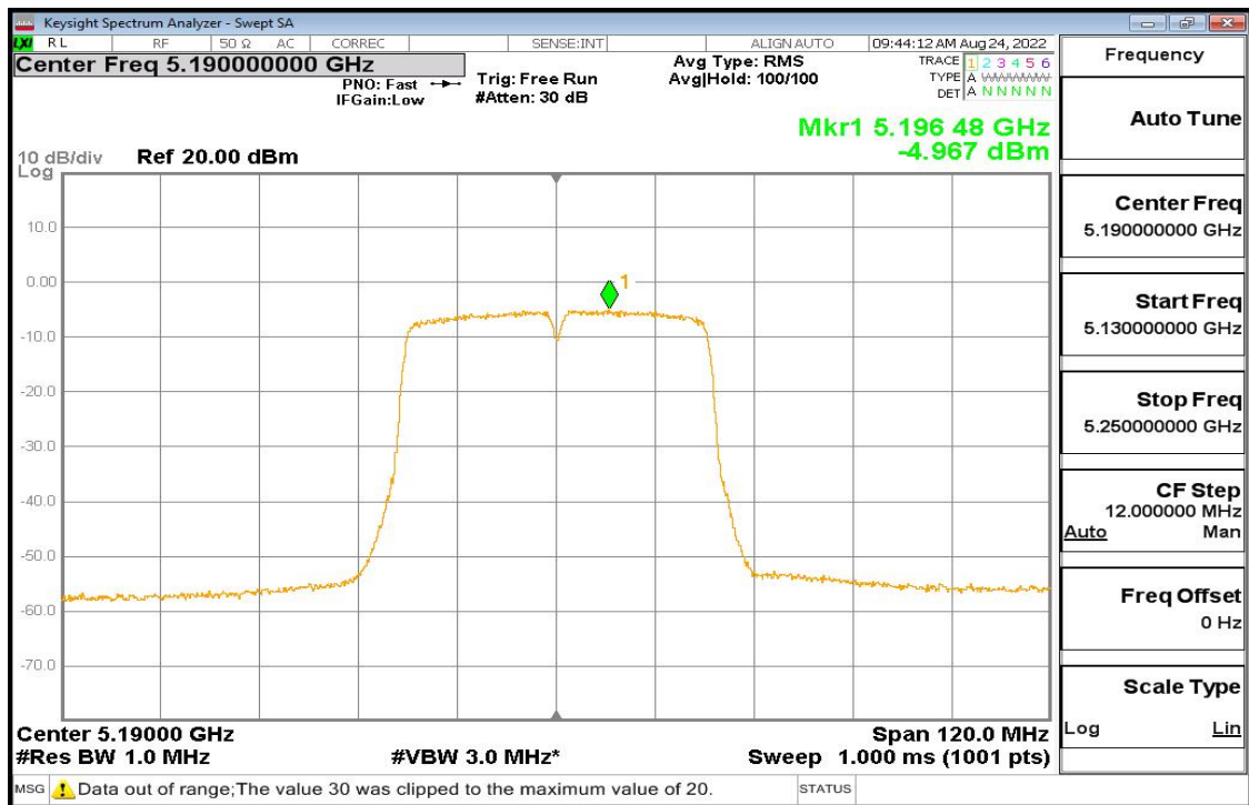
11ac-40 Pic1
