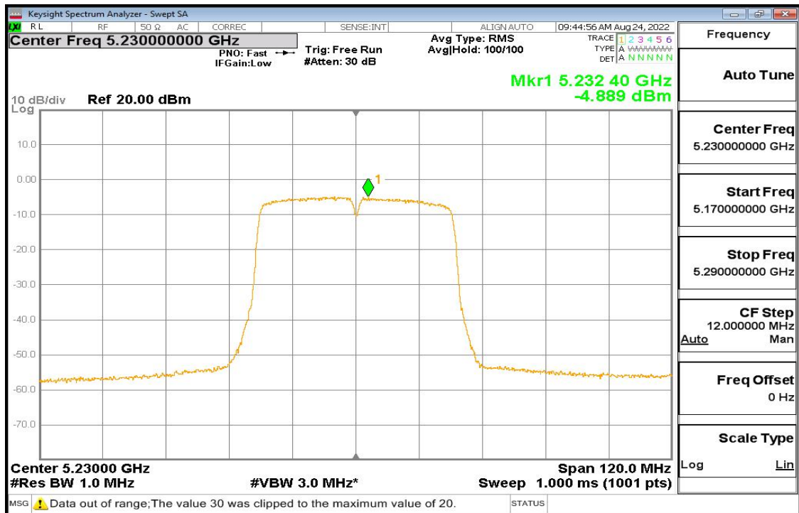
11ac-40 Pic2
