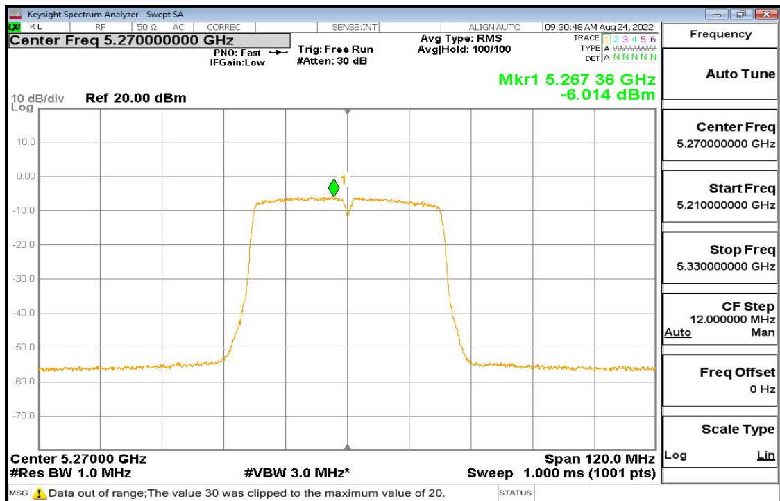
11n-40 Pic3
