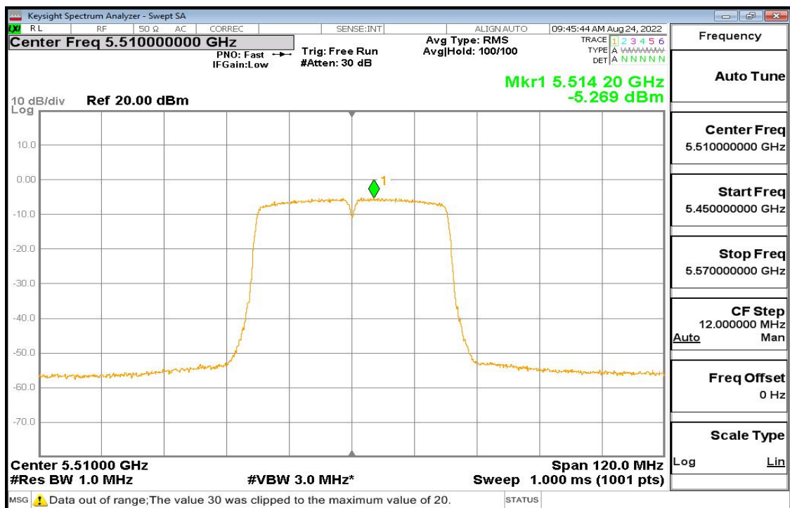
11ac-40 Pic5
