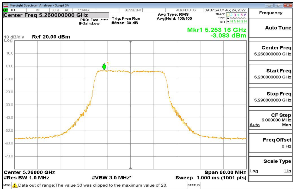
11ac-20 Pic4
