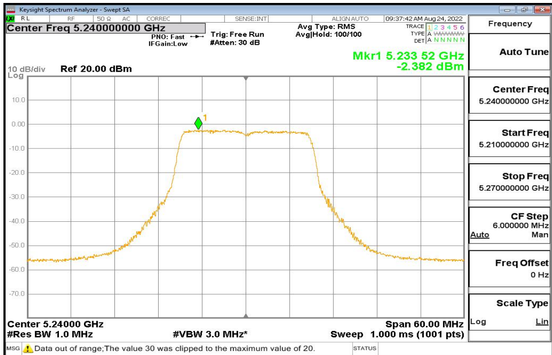
11ac-20 Pic3
