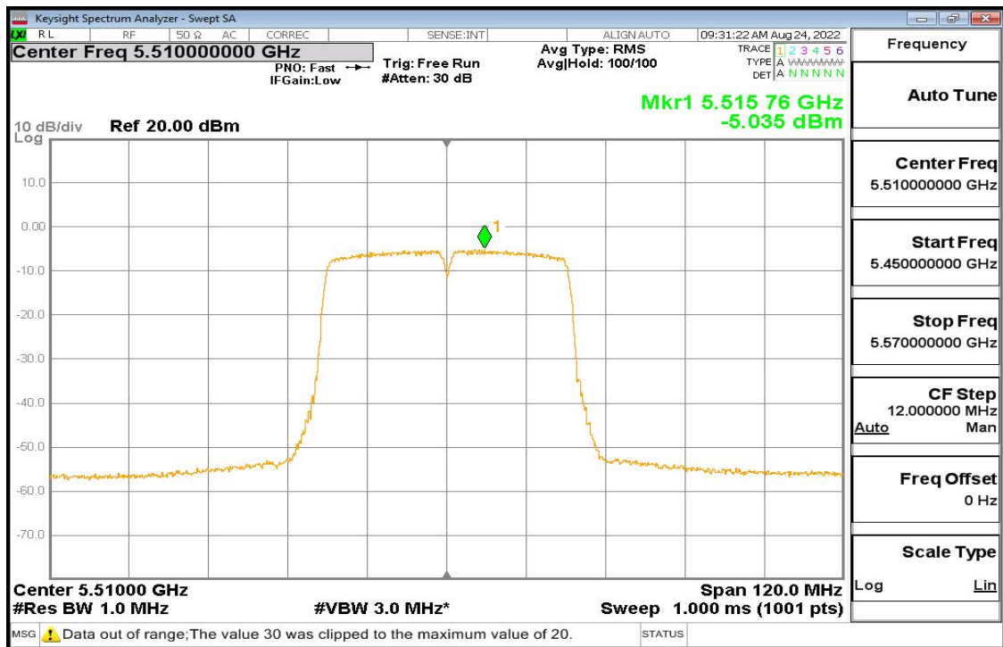
11n-40 Pic5
