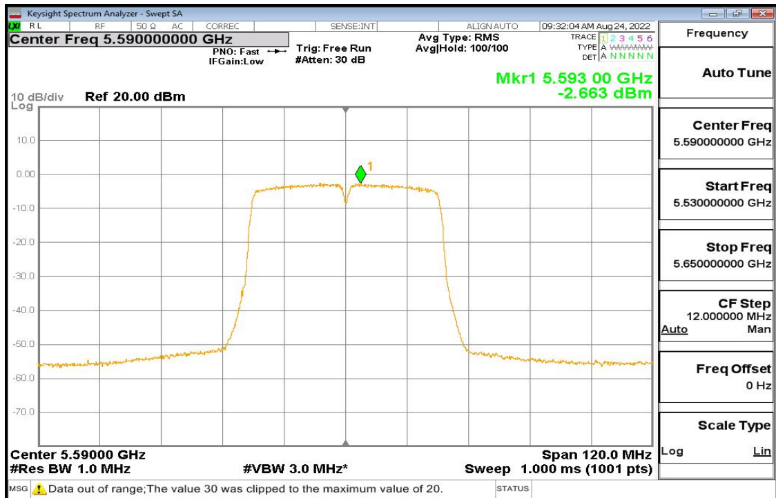
11n-40 Pic6
