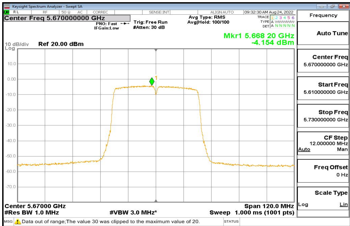
11n-40 Pic7
