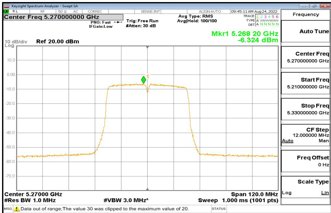
11ac-40 Pic3
