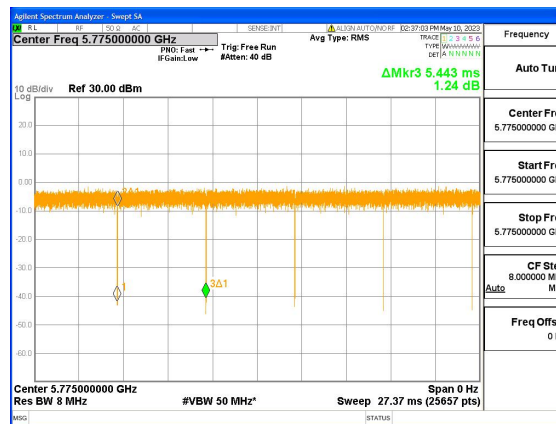
UNII-3-11ac-VHT80-Duty cycle
