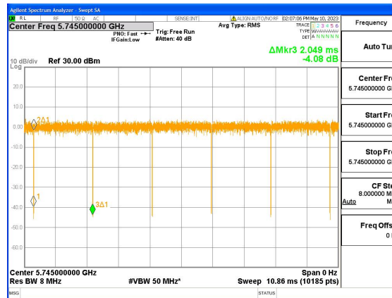
UNII-3-11a-Duty cycle
