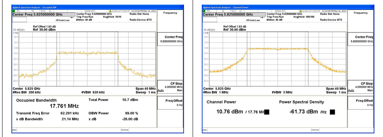
pic3_Obw
