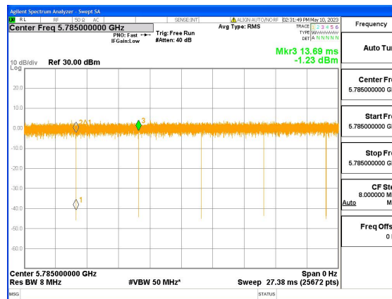
UNII-3-11ac-VHT20-Duty cycle
