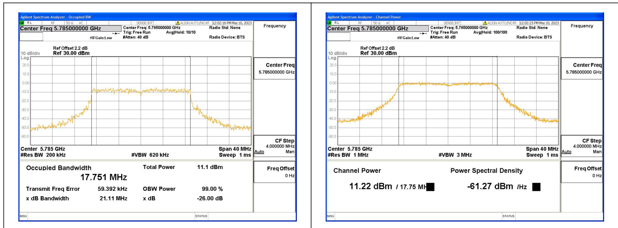
pic3_Obw
