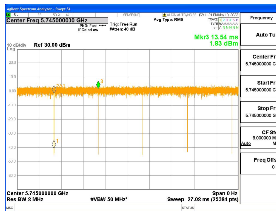
UNII-3-11n-HT20-Duty cycle
