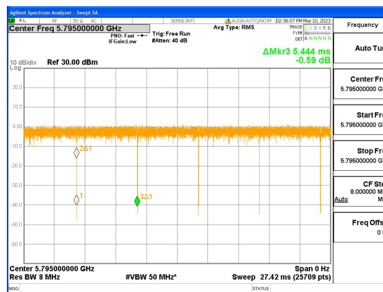
UNII-3-11ac-VHT40-Duty cycle
