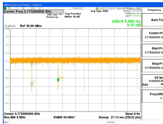
UNII-3-11ax-HE80-Duty cycle
