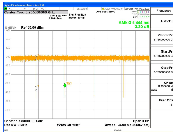
UNII-3-11n-HT40-Duty cycle
