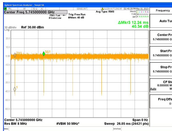
UNII-3-11ax-HE20-Duty cycle
