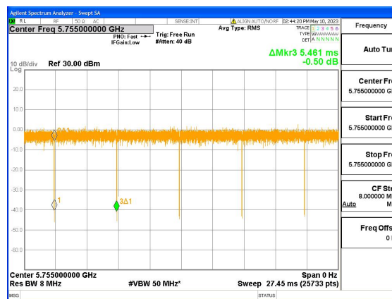
UNII-3-11ax-HE40-Duty cycle
