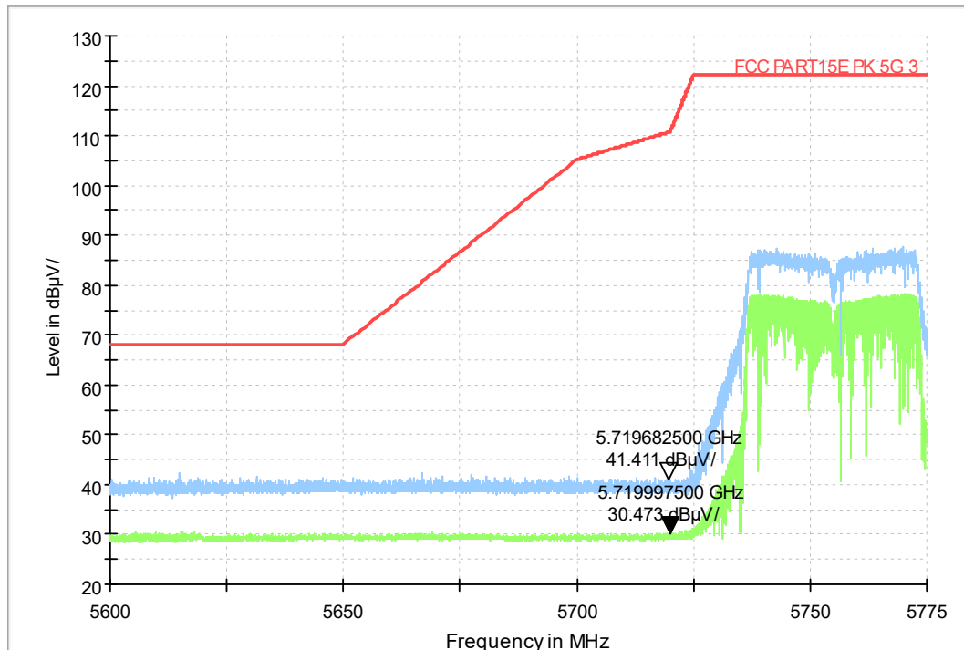
Fig.5 Frequency Band Edge: Ch151,11n 40M
