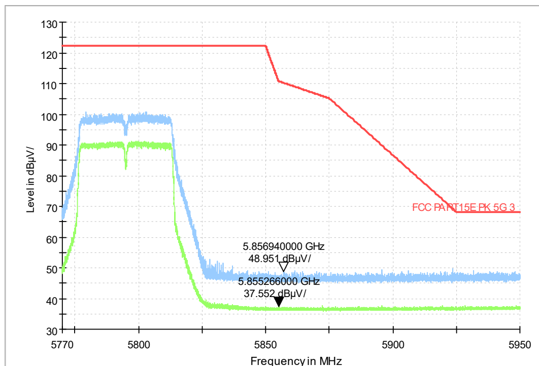
Fig.6 Frequency Band Edge: Ch159,11n 40M
