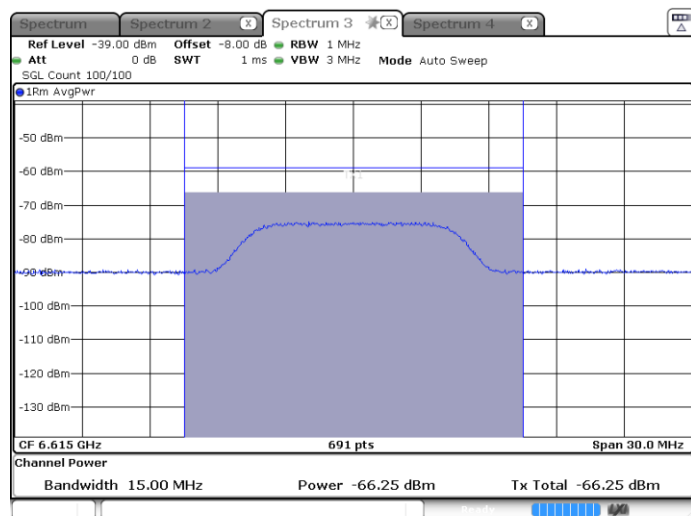
802.11ax (HE20)-Channel 133
