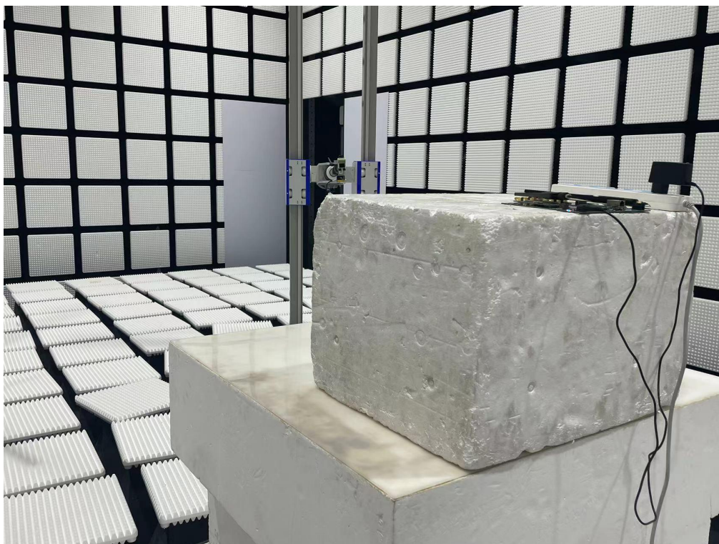
Pic4. Radiated emissions (26.5GHz-40GHz)
