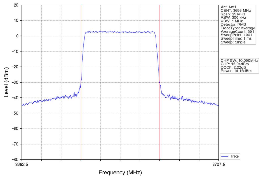
Band48_10MHz_16QAM_HCH_3695MHz_RB_50_0_NTNV
