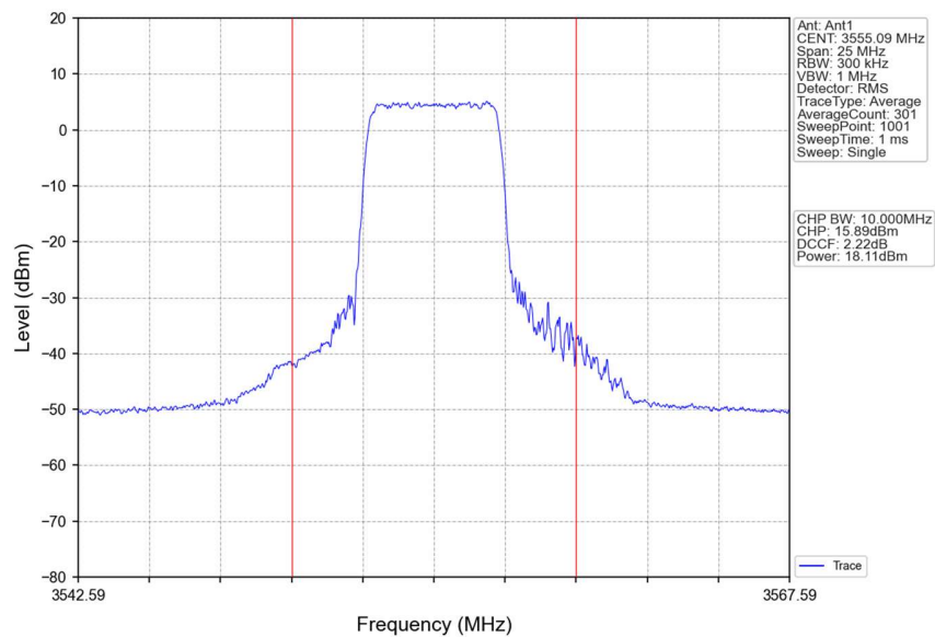
Band48_10MHz_16QAM_LCH_3555MHz_RB_25_13_NTNV
