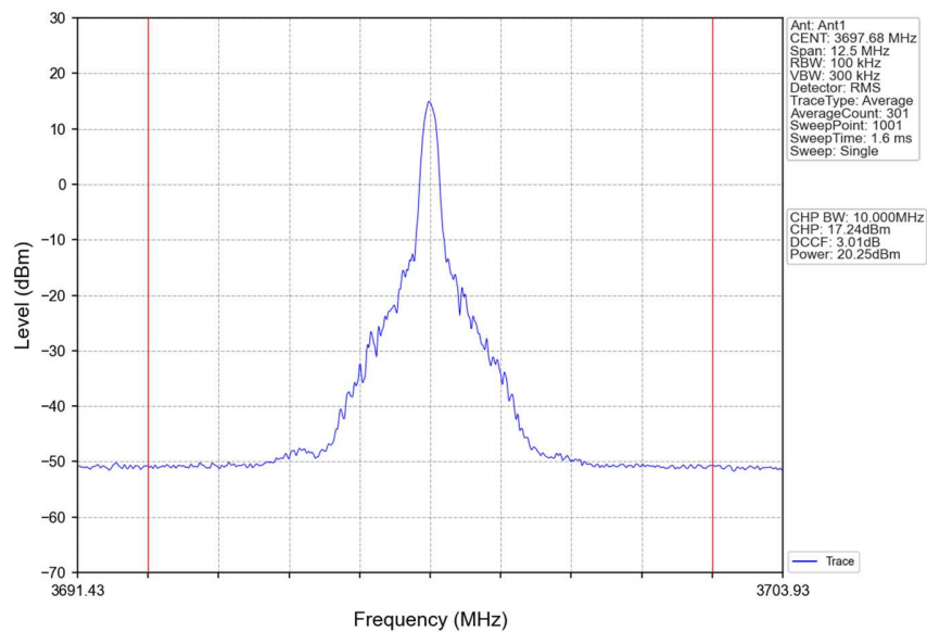
Band48_5MHz_64QAM_HCH_3697.5MHz_RB_1_13_NTNV
