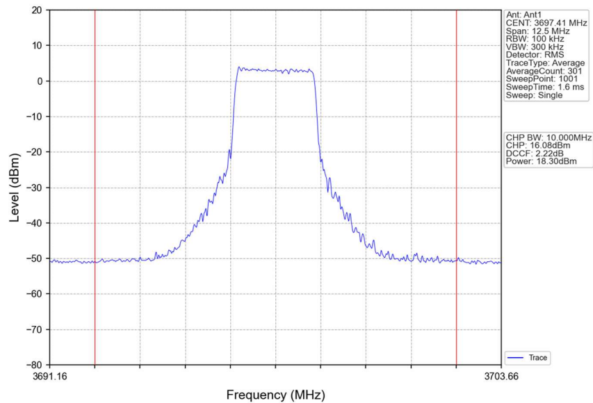
Band48_5MHz_64QAM_HCH_3697.5MHz_RB_12_13_NTNV
