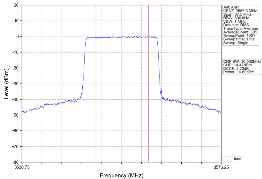
Band48_15MHz_16QAM_LCH_3557.5MHz_RB_75_0_NTNV
