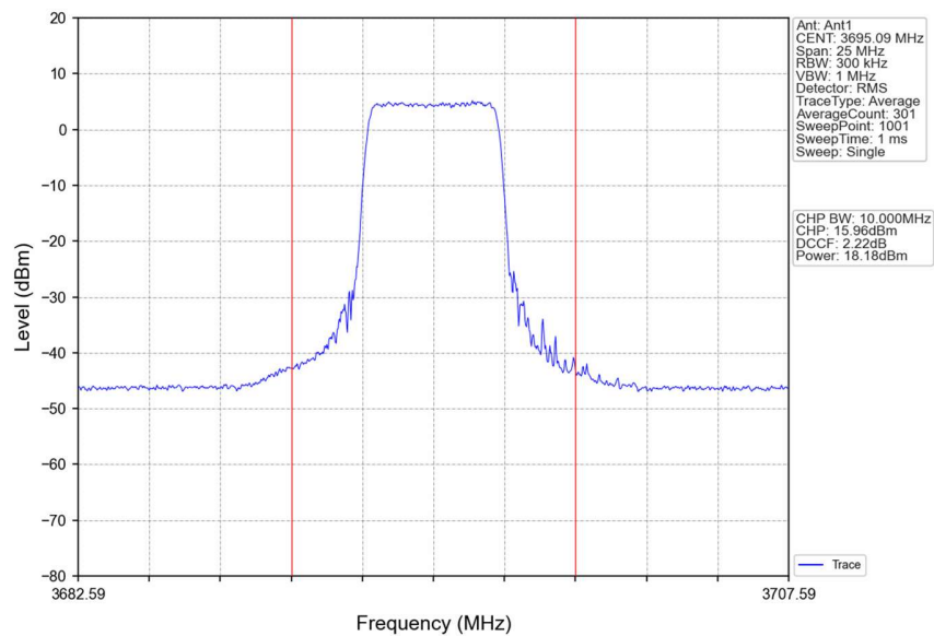
Band48_10MHz_64QAM_HCH_3695MHz_RB_25_25_NTNV
