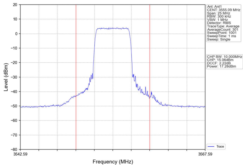
Band48_10MHz_64QAM_LCH_3555MHz_RB_25_25_NTNV
