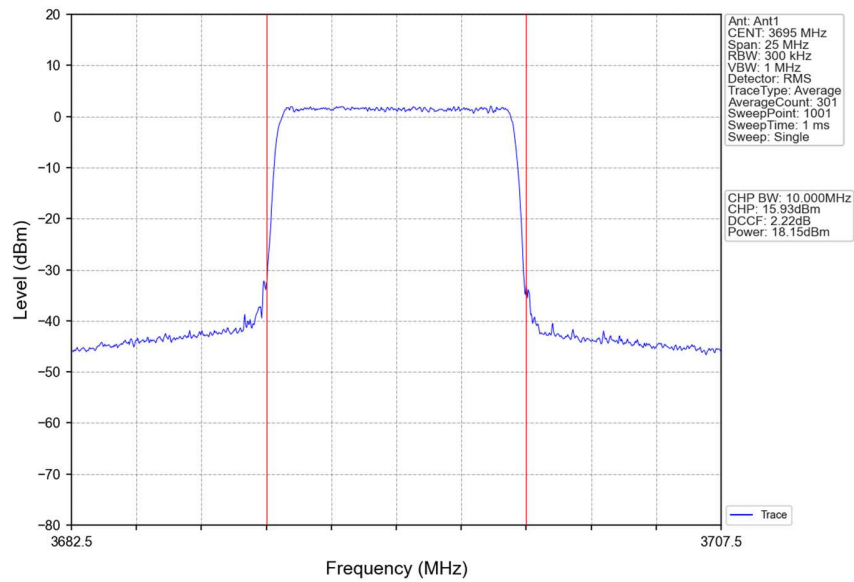
Band48_10MHz_64QAM_HCH_3695MHz_RB_50_0_NTNV
