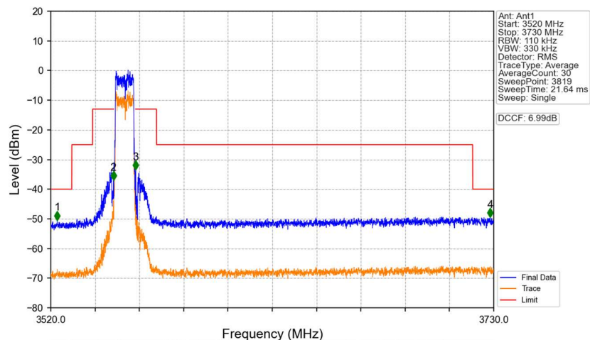
n48_30kHz_SISO_NTNV_10MHz_CP-OFDM QPSK_3555MHz_Outer_Full
