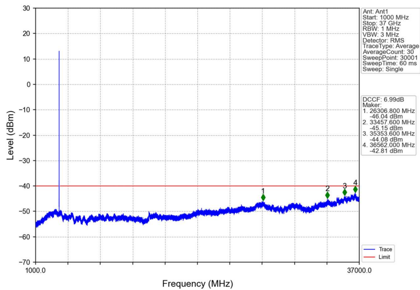
n48_30kHz_SISO_NTNV_10MHz_DFT-s-OFDM QPSK_3694.98MHz_Edge_1RB_Right
