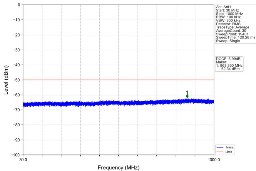
n48_30kHz_SISO_NTNV_10MHz_CP-OFDM QPSK_3694.98MHz_Edge_1RB_Right
