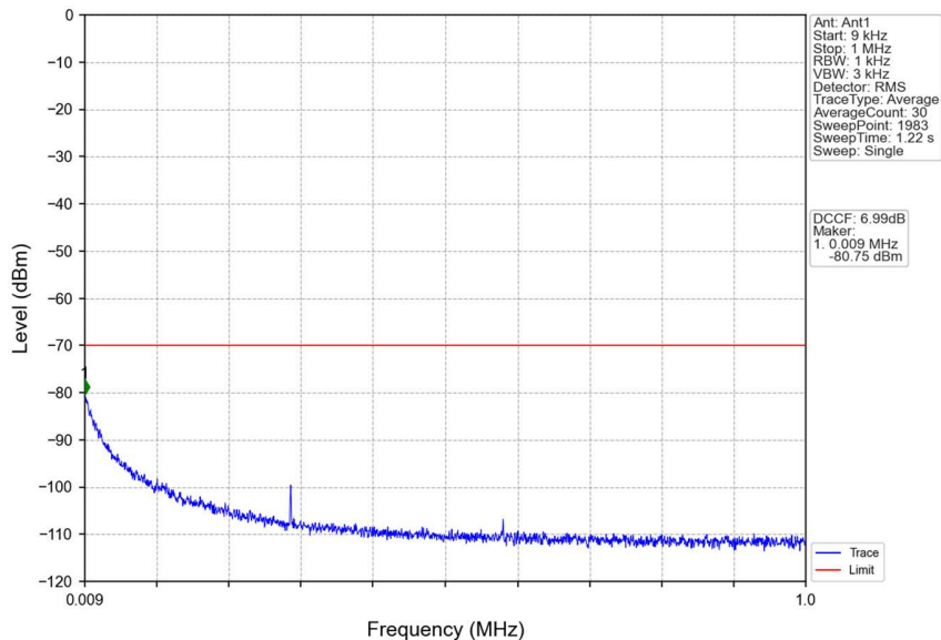
n48_30kHz_SISO_NTNV_10MHz_DFT-s-OFDM QPSK_3624.99MHz_Edge_1RB_Left
