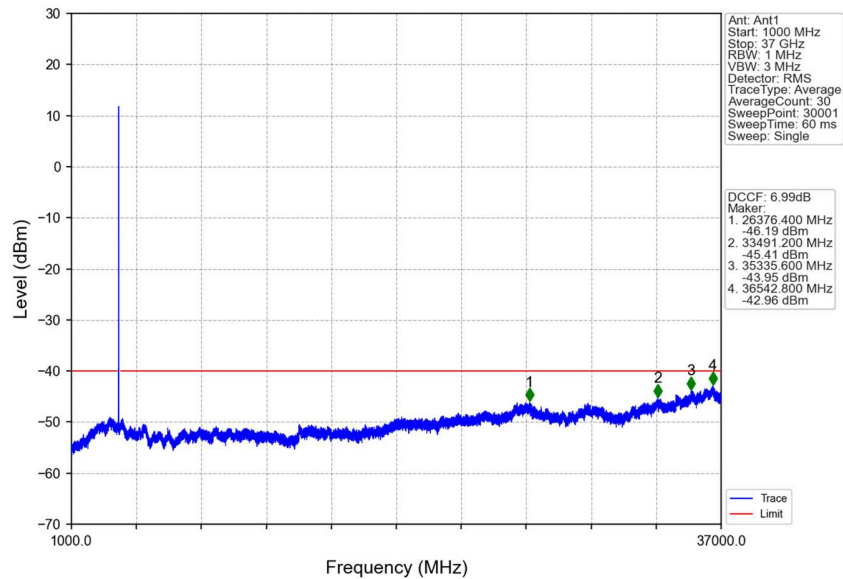
n48_30kHz_SISO_NTNV_10MHz_CP-OFDM QPSK_3624.99MHz_Edge_1RB_Left
