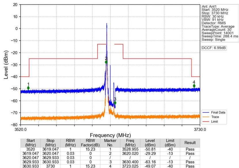
n48_30kHz_SISO_NTNV_10MHz_CP-OFDM QPSK_3624.99MHz_Edge_1RB_Left
