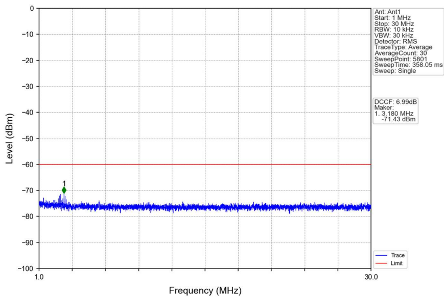
n48_30kHz_SISO_NTNV_10MHz_DFT-s-OFDM QPSK_3694.98MHz_Outer_Full
