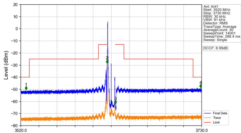
n48_30kHz_SISO_NTNV_10MHz_DFT-s-OFDM QPSK_3624.99MHz_Edge_1RB_Left
