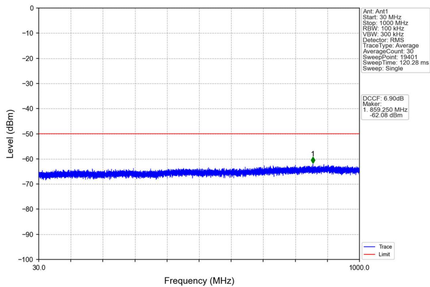
n48_30kHz_SISO_NTNV_10MHz_DFT-s-OFDM QPSK_3694.98MHz_Edge_1RB_Right
