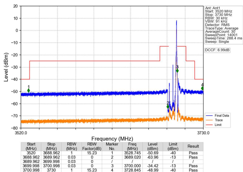
n48_30kHz_SISO_NTNV_10MHz_CP-OFDM QPSK_3694.98MHz_Edge_1RB_Right
