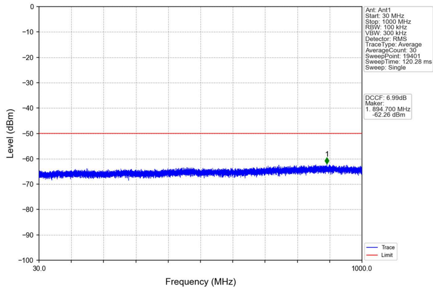
n48_30kHz_SISO_NTNV_10MHz_CP-OFDM QPSK_3624.99MHz_Edge_1RB_Left
