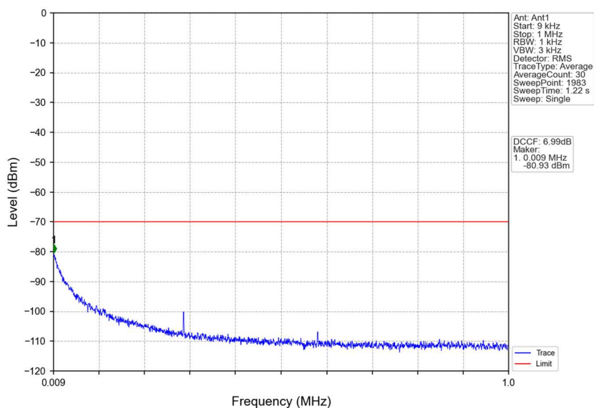
n48_30kHz_SISO_NTNV_10MHz_CP-OFDM QPSK_3694.98MHz_Edge_1RB_Right
