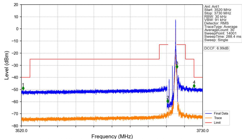
n48_30kHz_SISO_NTNV_10MHz_DFT-s-OFDM QPSK_3694.98MHz_Inner_1RB_Right
