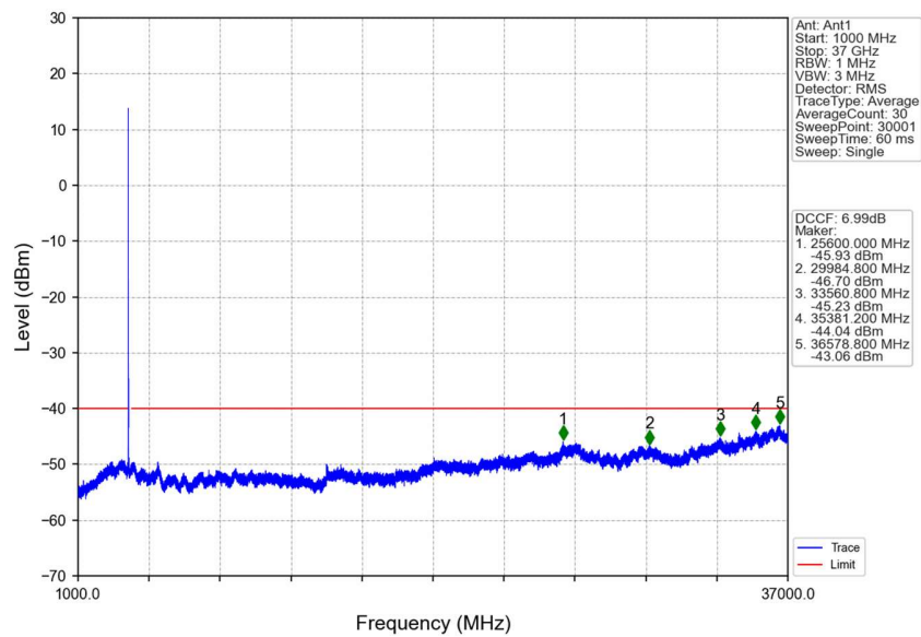
n48_30kHz_SISO_NTNV_10MHz_CP-OFDM QPSK_3555MHz_Outer_Full
