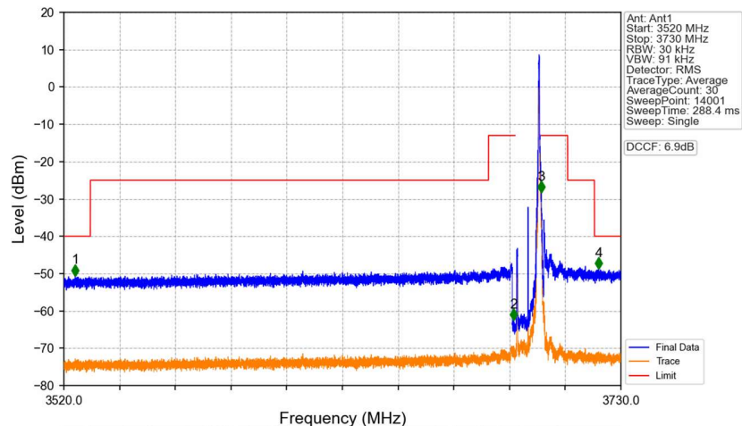
n48_30kHz_SISO_NTNV_10MHz_DFT-s-OFDM QPSK_3694.98MHz_Edge_1RB_Right
