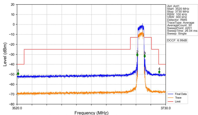
n48_30kHz_SISO_NTNV_10MHz_CP-OFDM QPSK_3694.98MHz_Outer_Full
