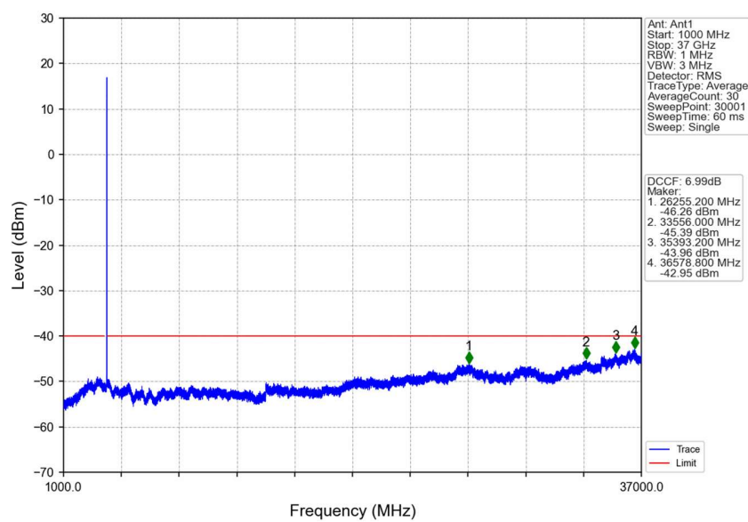
n48_30kHz_SISO_NTNV_10MHz_CP-OFDM QPSK_3694.98MHz_Outer_Full
