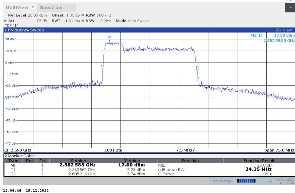
LTE CA band N41 , 5MHz+20MHz Bandwidth,16QAM (-26dBc BW)
