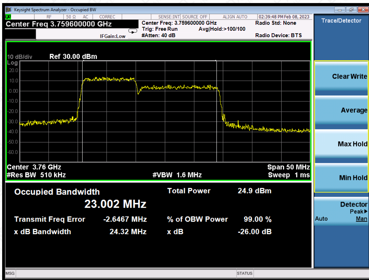
LTE CA band 43Part27 , 10MHz+15MHz Bandwidth,64QAM (-26dB BW)
