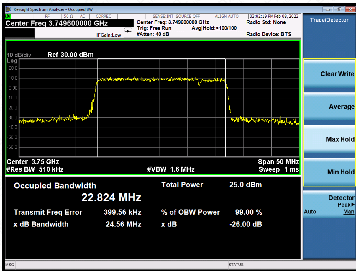
LTE CA band 43Part27 , 20MHz+5MHz Bandwidth,64QAM (-26dBc BW)
