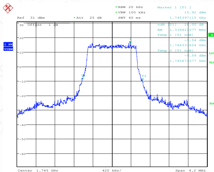
LTE band 66 , 1.4MHz Bandwidth,MID,QPSK (-26dBc BW)
