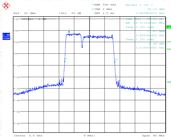
LTE CA band 42Part27 , 10MHz+20MHz Bandwidth,QPSK (-26dBc BW)
