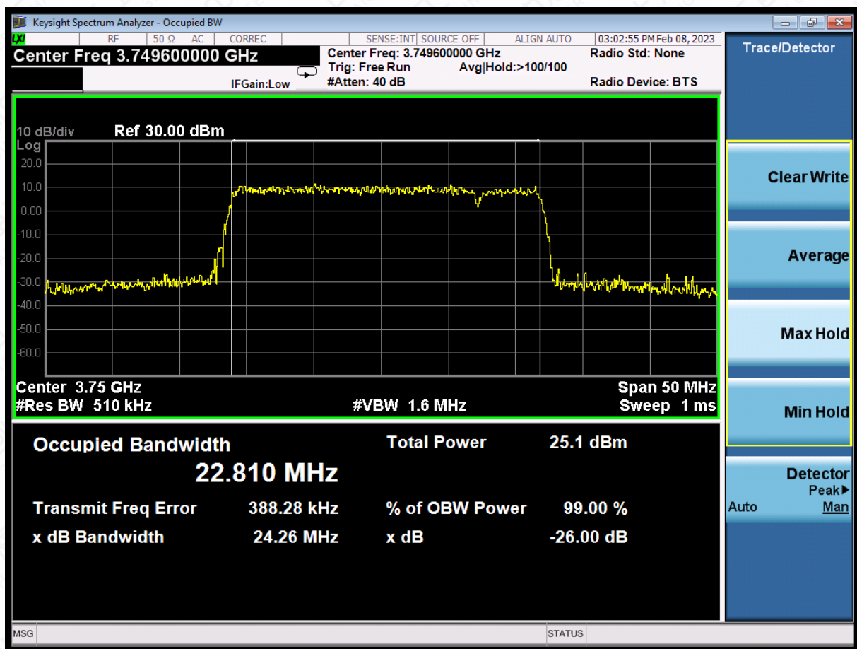
LTE CA band 43Part27,20MHz+5MHz(-26dBc)*
