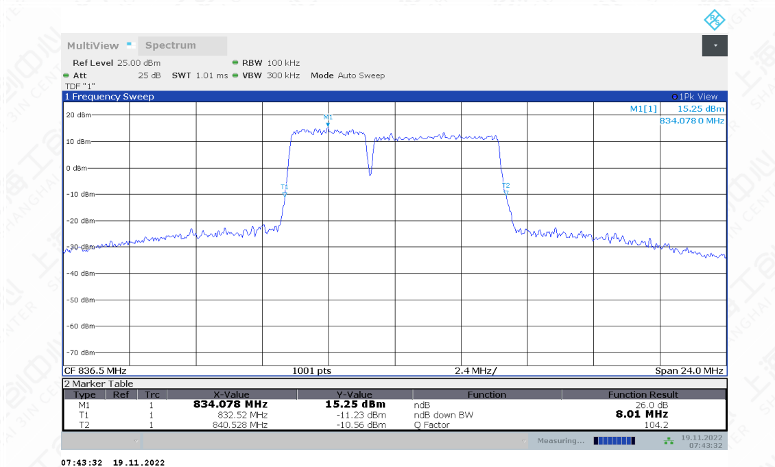
LTE CA band 5 , 3MHz+5MHz Bandwidth,QPSK (-26dBc BW)
