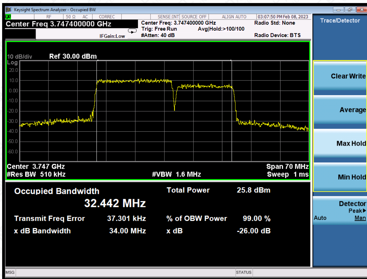
LTE CA band 43Part27 , 20MHz+15MHz Bandwidth,16QAM (-26dBc BW)
