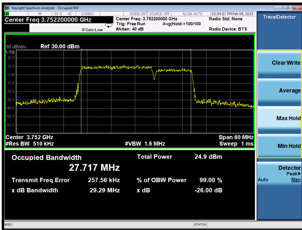
LTE CA band 43Part27,20MHz+15MHz(-26dBc)*
