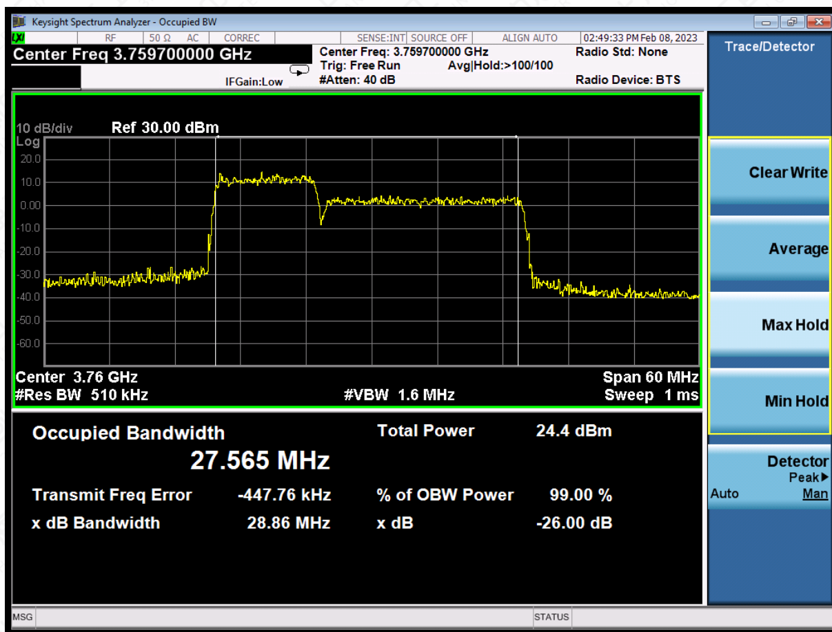
LTE CA band 43Part27,15MHz+10MHz(-26dBc)*
