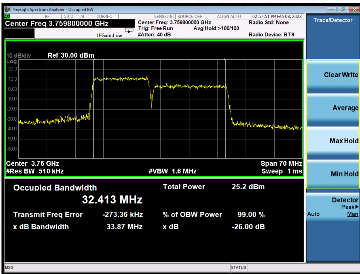
LTE CA band 43Part27,20MHz+10MHz(-26dBc)*
