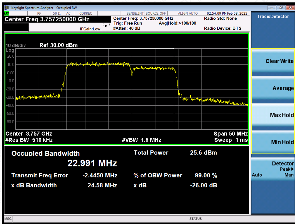
LTE CA band 43Part27 ,15MHz+10MHz Bandwidth,16QAM (-26dBc BW)
