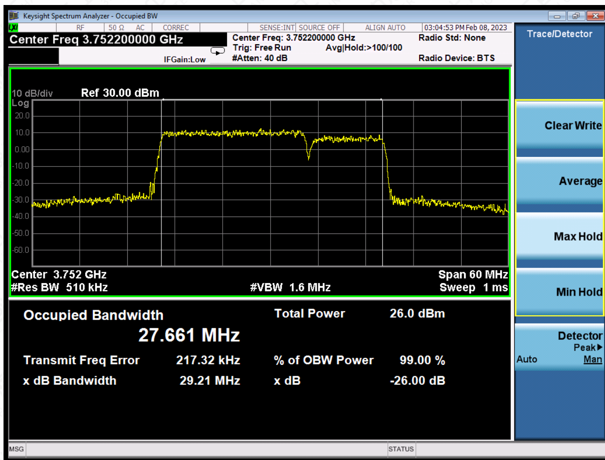
LTE CA band 43Part27 , 20MHz+10MHz Bandwidth,16QAM (-26dB BW)
