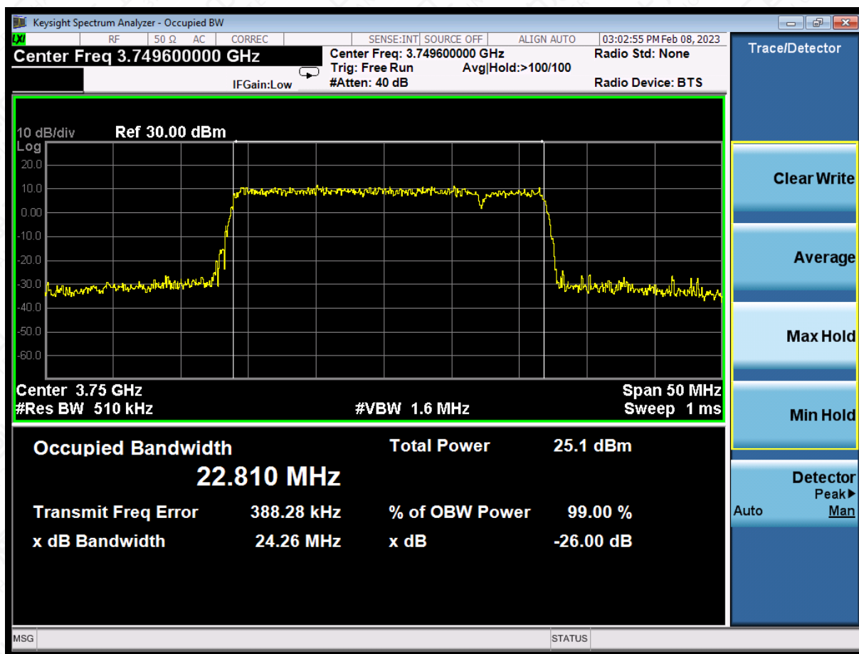
LTE CA band 43Part27,15MHz+20MHz(-26dBc)*
