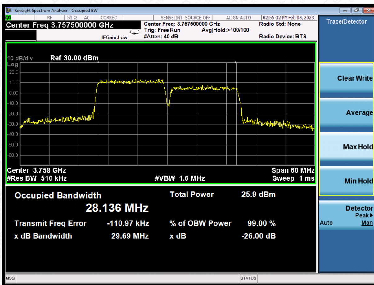
LTE CA band 43Part27 ,15MHz+15MHz Bandwidth,16QAM (-26dBc BW)
