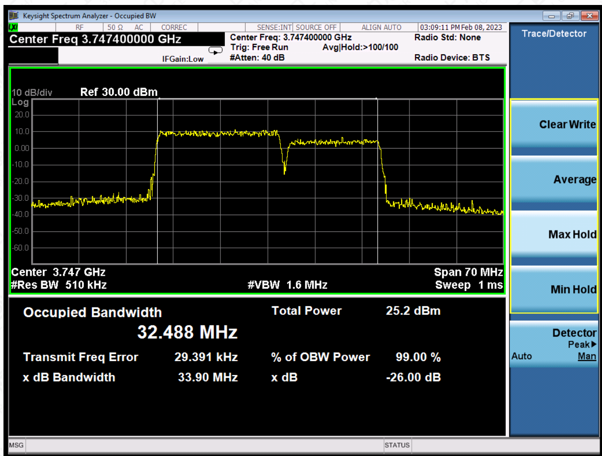
LTE CA band 43Part27,20MHz+20MHz(-26dBc)*
