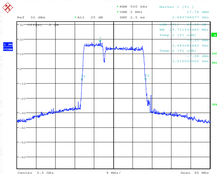
LTE CA band N42Part27 , 10MHz+20MHz Bandwidth,16QAM (-26dBc BW)
