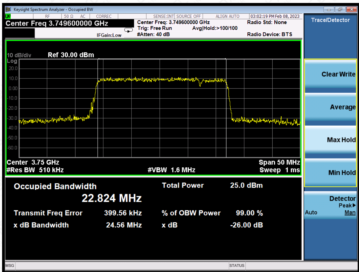
LTE CA band 43Part27 , 20MHz+5MHz Bandwidth,64QAM (-26dBc BW)
