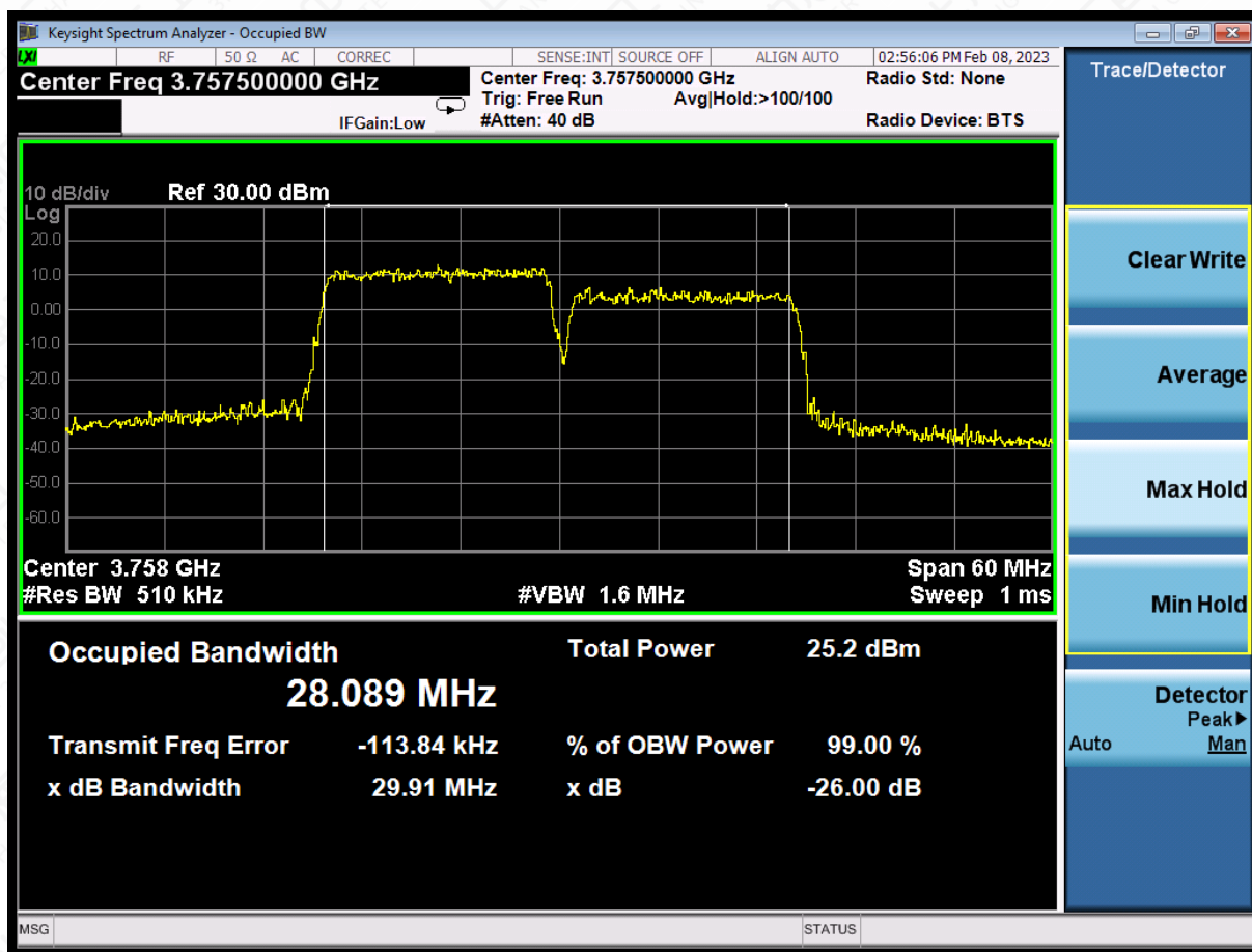
LTE CA band 43Part27 , 15MHz+15MHz Bandwidth,64QAM (-26dBc BW)
