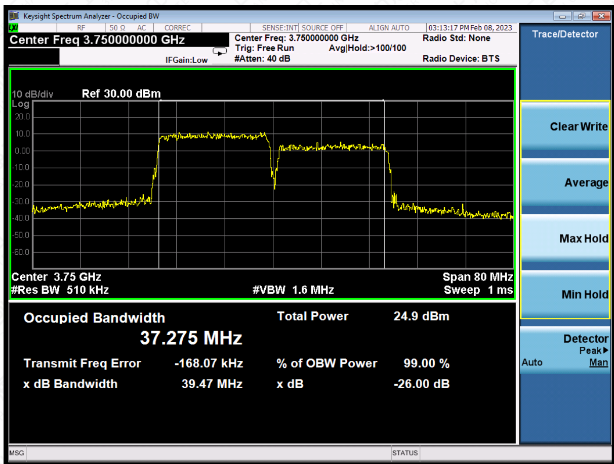
LTE CA band 43Part27 , 20MHz+20MHz Bandwidth,64QAM (-26dBc BW)
