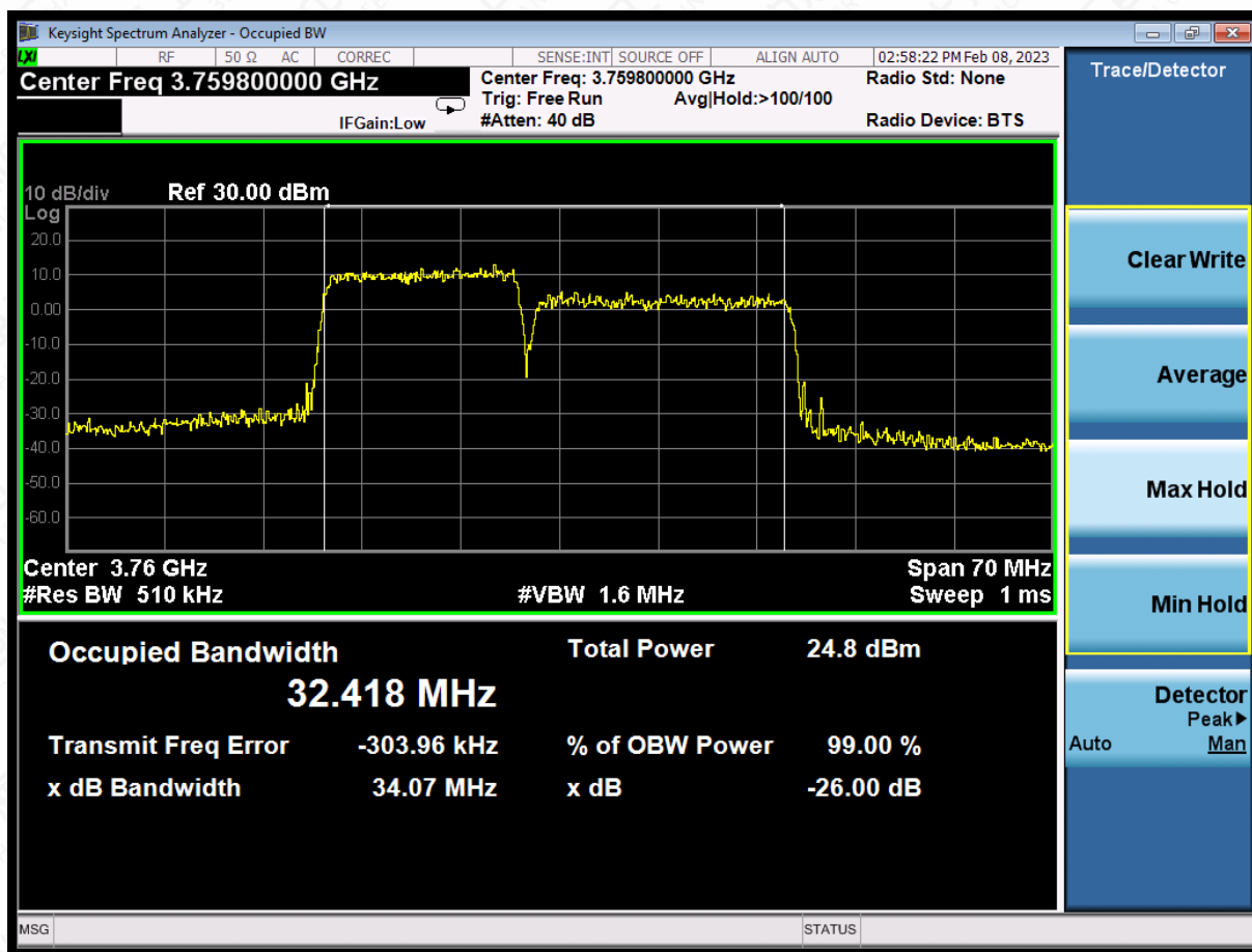
LTE CA band 43Part27 , 15MHz+20MHz Bandwidth,64QAM (-26dB BW)
