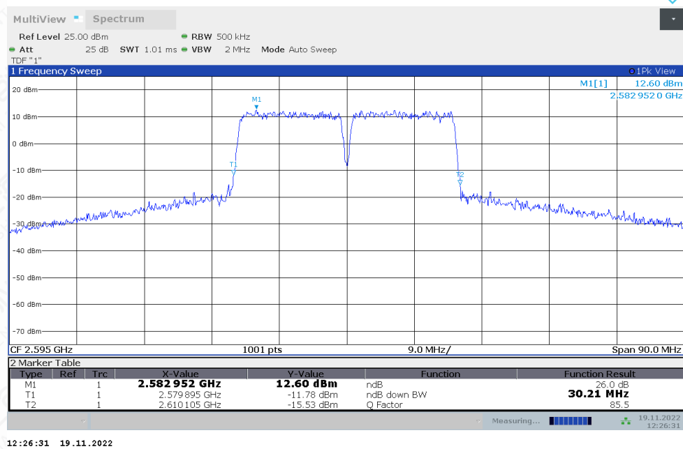
LTE CA band N38 , 15MHz+15MHz Bandwidth,16QAM (-26dBc BW)
