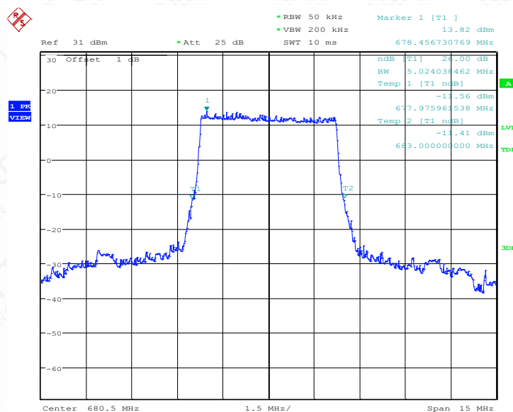
LTE band 71 , 5MHz Bandwidth,MID,QPSK (-26dBc BW)
