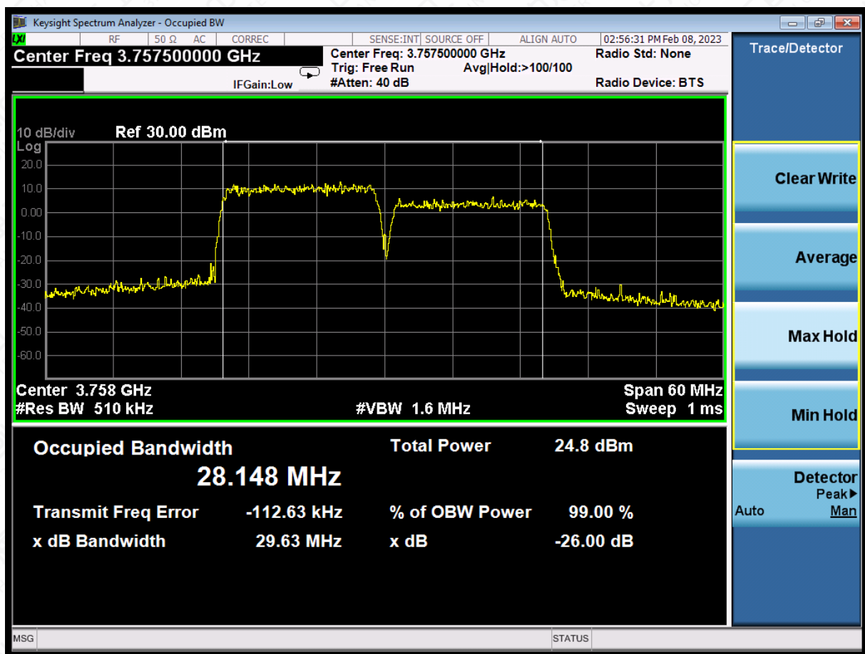
LTE CA band 43Part27,10MHz+15MHz(-26dBc)*
