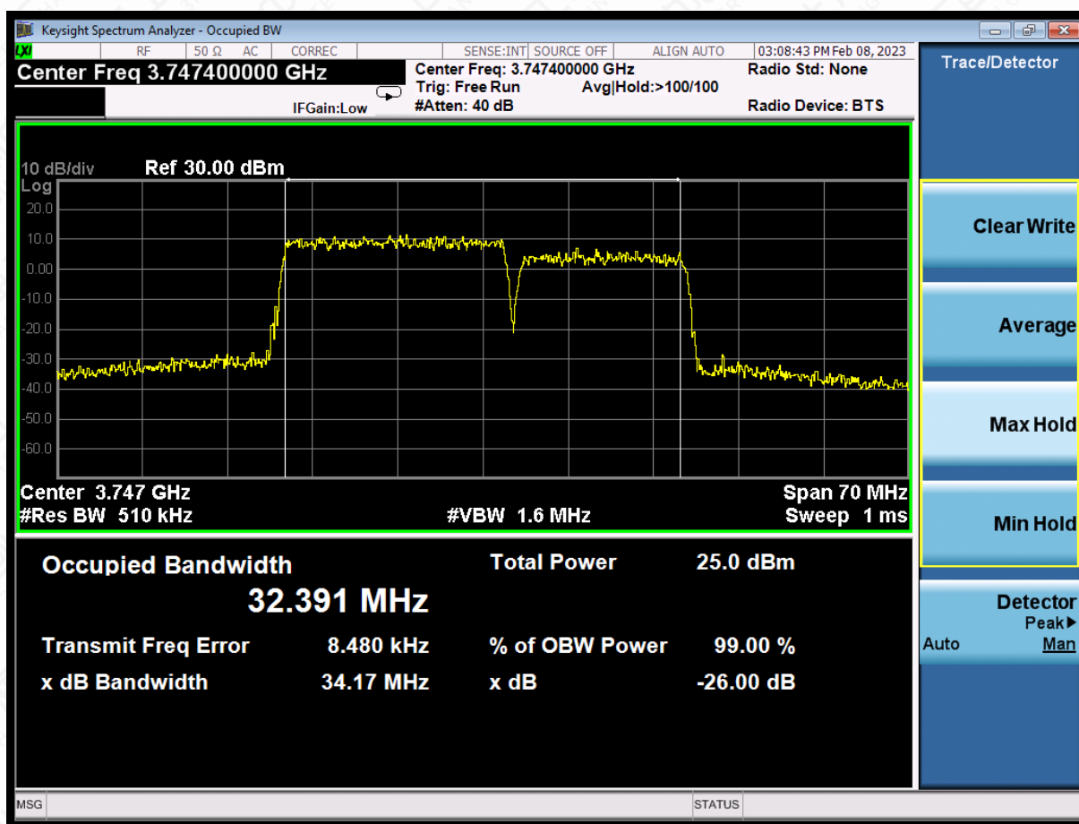
LTE CA band 43Part27 , 20MHz+15MHz Bandwidth,64QAM (-26dB BW)
