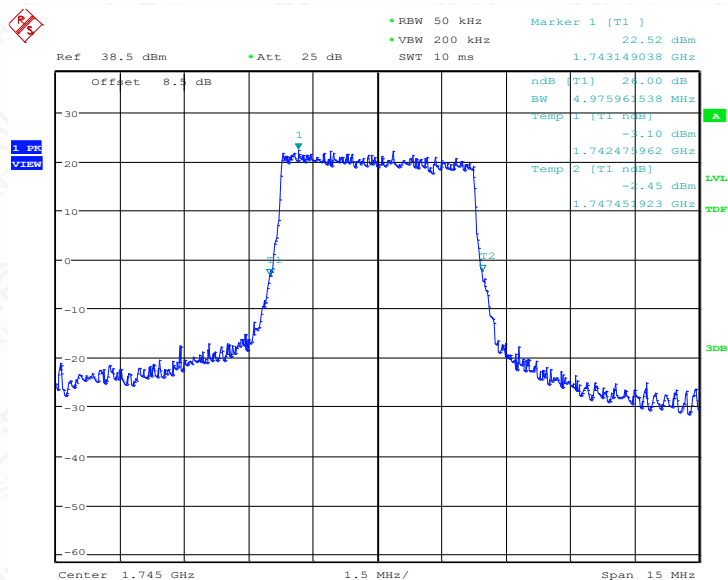
LTE band 66@CA_2+66, 5MHz Bandwidth, QPSK (-26dB BW)
