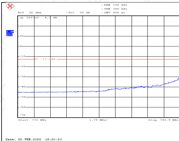
FDD14_5MHz_795.5_QPSK_fullRB_ExtraBand ds_Range_775~792.9
