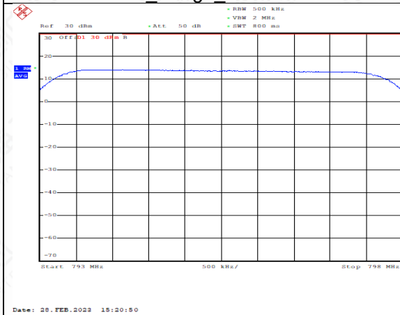
FDD14_5MHz_795.5_QPSK_fullRB_ExtraBand ds_Range_793~798
