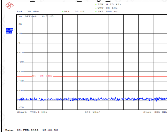
LowRange_FDD14_10MHz_793_fullRB _Low_QPSK
