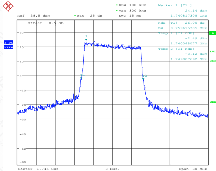
LTE band 66@CA_2+66, 10MHz Bandwidth, QPSK (-26dBc BW)
