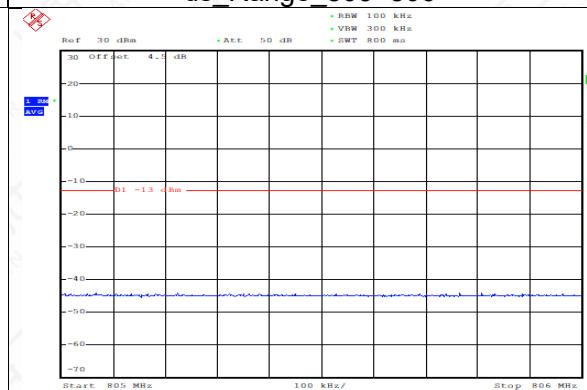
FDD14_5MHz_790.5_QPSK_fullRB_ExtraBands_Range_805~806
