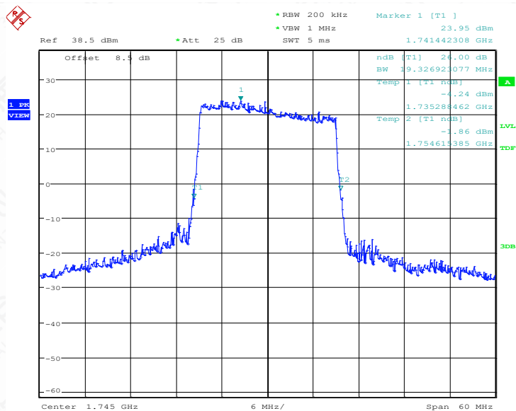
LTE band 66@CA_2+66, 20MHz Bandwidth, 64QAM (-26dBc BW)
