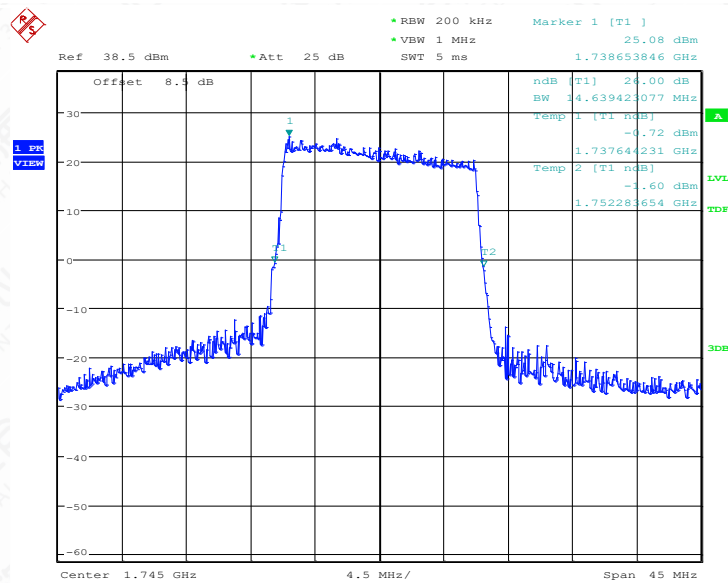
LTE band 66@CA_2+66, 15MHz Bandwidth, 64QAM (-26dBc BW)
