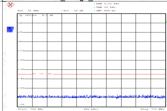
FDD14_5MHz_790.5_QPSK_fullRB_ExtraBand ds_Range_769~775
