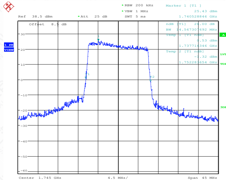
LTE band 66@CA_2+66, 15MHz Bandwidth, QPSK (-26dBc BW)
