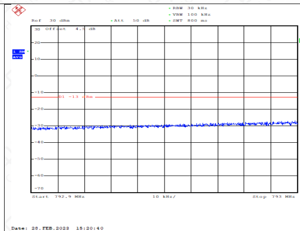
FDD14_5MHz_795.5_QPSK_fullRB_ExtraBand ds_Range_792.9~793
