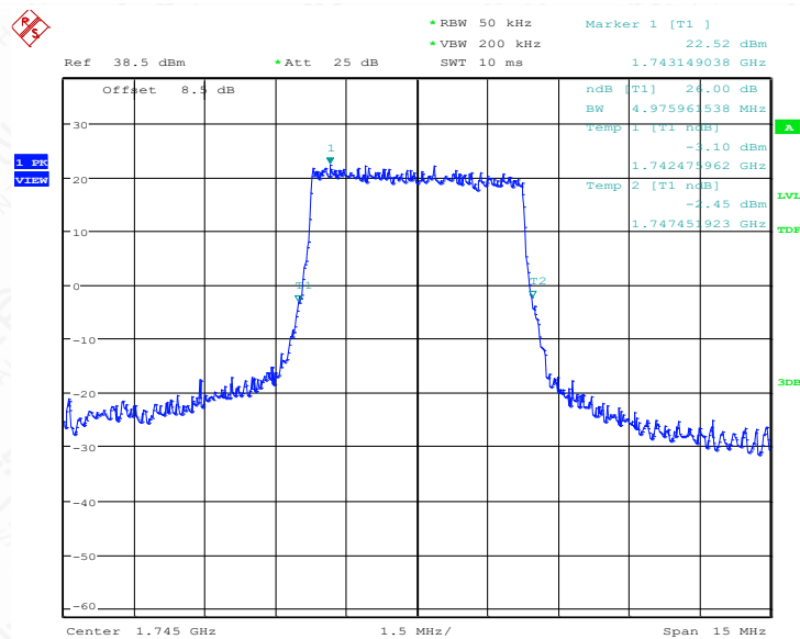
LTE band 66@CA_2+66, 5MHz Bandwidth, QPSK (-26dB BW)
