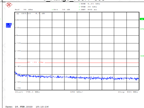
FDD14_5MHz_795.5_OneRB_high_QPSKHighRange
