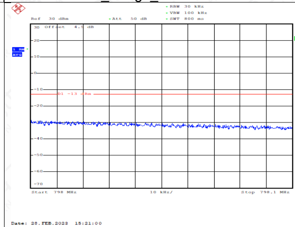
FDD14_5MHz_795.5_QPSK_fullRB_ExtraBand ds_Range_798~798.1
