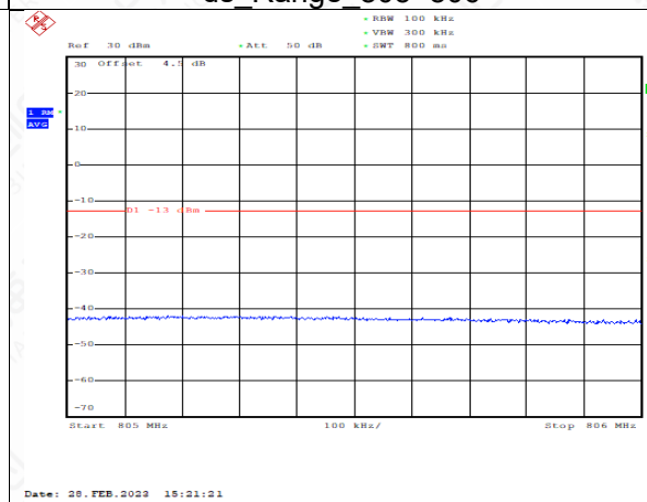
FDD14_5MHz_795.5_QPSK_fullRB_ExtraBand ds_Range_805~806
