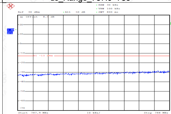
FDD14_5MHz_790.5_QPSK_fullRB_ExtraBand ds_Range_787.9~788
