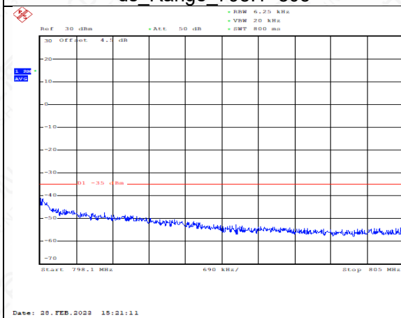
FDD14_5MHz_795.5_QPSK_fullRB_ExtraBand ds_Range_798.1~805
