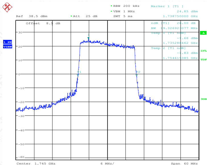
LTE band 66@CA_2+66, 20MHz Bandwidth, QPSK (-26dBc BW)
