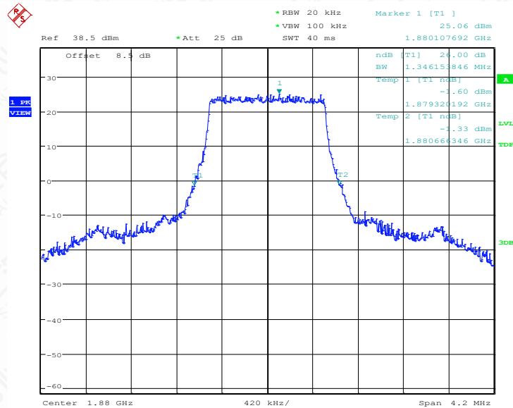
LTE band 2@CA_2+66, 1.4MHz Bandwidth, QPSK (-26dB BW)
