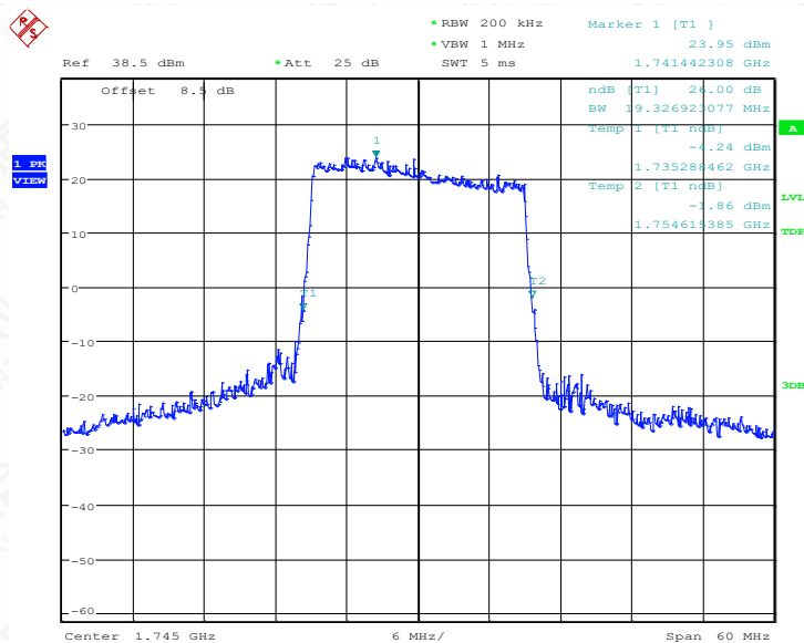
LTE band 66@CA_2+66, 20MHz Bandwidth, 64QAM (-26dBc BW)
