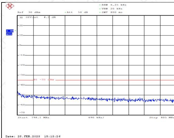
LowRange_FDD14_5MHz_790.5_OneRB_low_Low_QPSK
