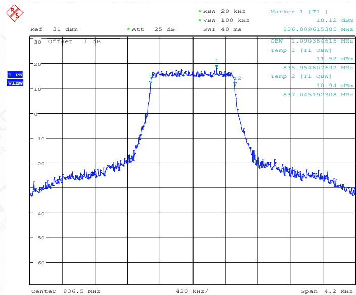
LTE band 5 , 1.4MHz Bandwidth,MID,QPSK (99% BW)
