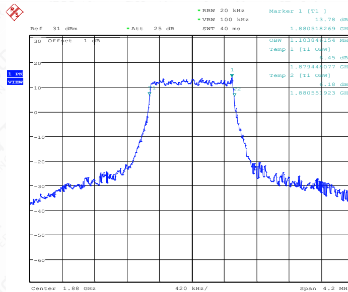
LTE band 2 , 1.4MHz Bandwidth,MID,16QAM (99% BW)
