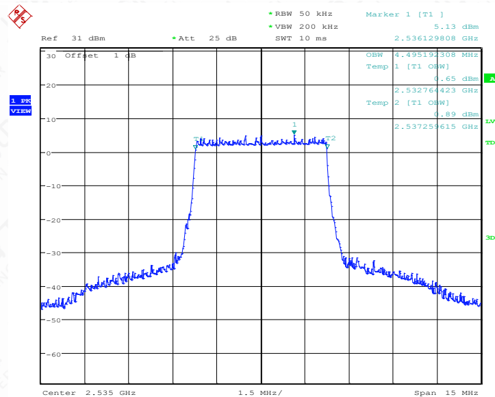
LTE band 7 , 5MHz Bandwidth,MID,QPSK (99% BW)
