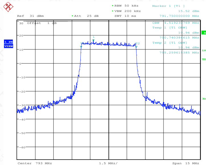
LTE band 14 , 5MHz Bandwidth,MID,QPSK (99% BW)
