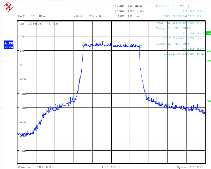
LTE band 13 , 5MHz Bandwidth,MID,QPSK (99% BW)
