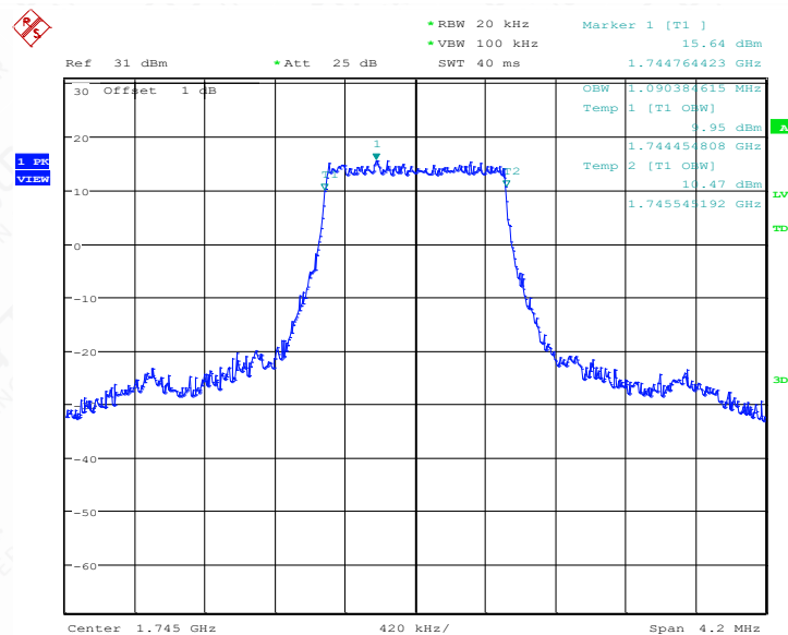
LTE band 66 , 1.4MHz Bandwidth,MID,QPSK (99% BW)
