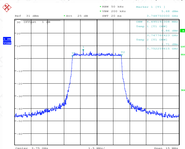
LTE band 43 , 5MHz Bandwidth,MID,QPSK (99% BW)
