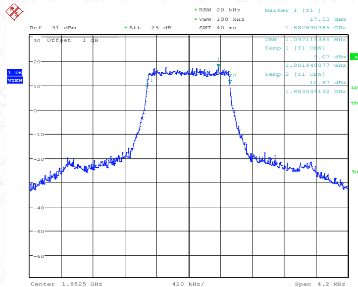
LTE band 25 , 1.4MHz Bandwidth,MID,QPSK (99% BW)
