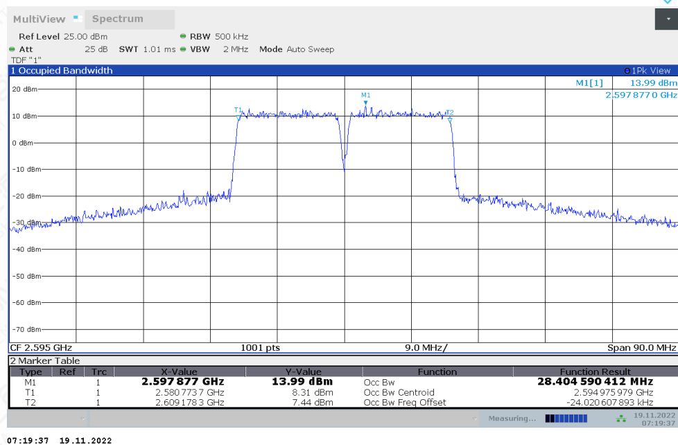
LTE CA band 38 , 15MHz+15MHz Bandwidth,16QAM (99% BW)
