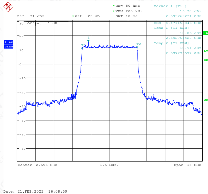
LTE band 38 , 5MHz Bandwidth,MID,QPSK (99% BW)
