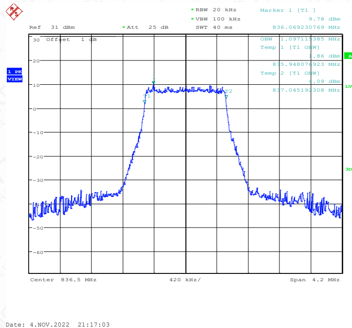
LTE band 26 , 1.4MHz Bandwidth,MID,64QAM (99% BW)
