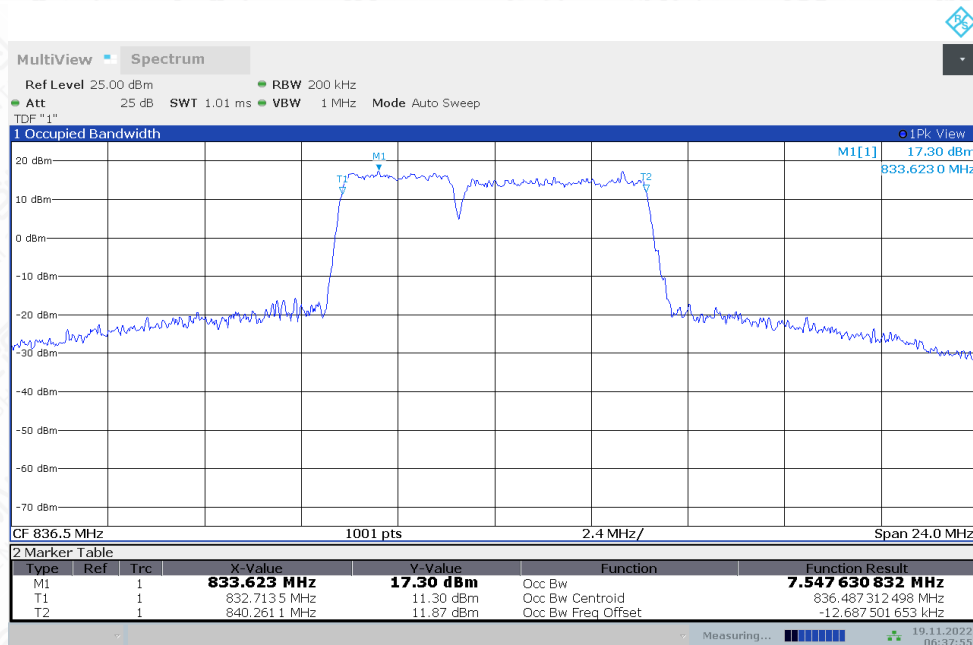
LTE CA band 5 , 3MHz+5MHz Bandwidth,QPSK (99% BW)
