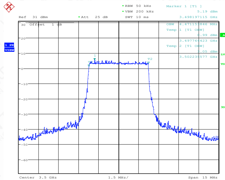
LTE band 42 , 5MHz Bandwidth,MID,QPSK (99% BW)
