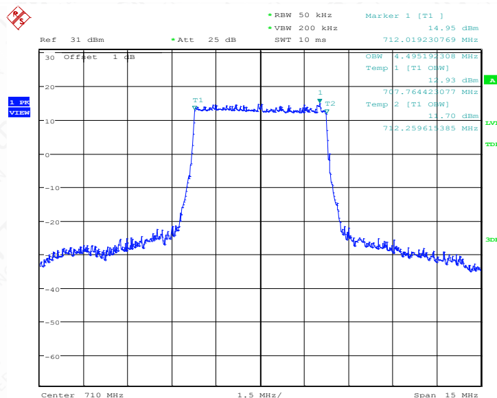
LTE band 17 , 5MHz Bandwidth,MID,QPSK (99% BW)
