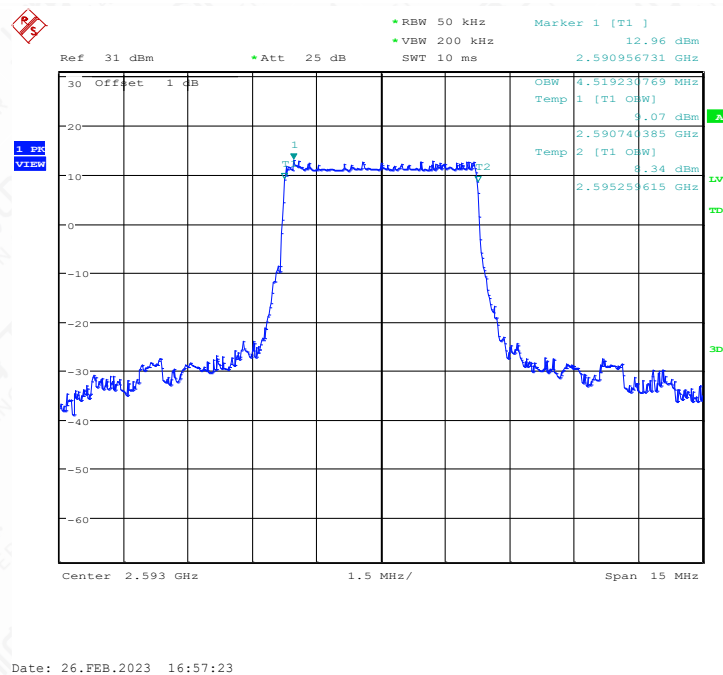
LTE band 41 , 5MHz Bandwidth,MID,QPSK (99% BW)
