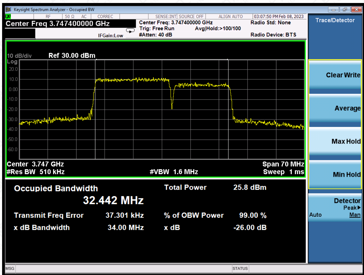
LTE CA band 43Part27 , 20MHz+15MHz Bandwidth,16QAM (99% BW)
