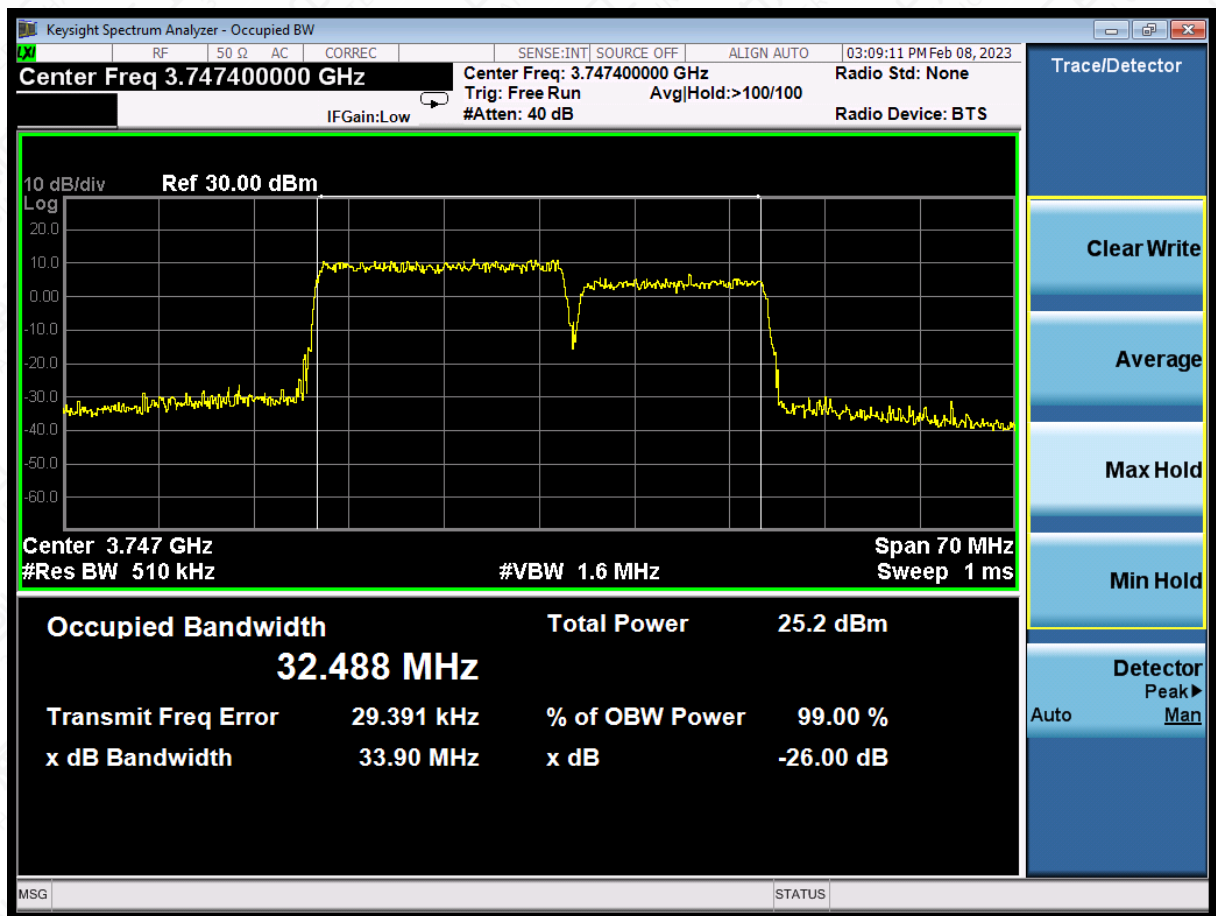
LTE CA band 43Part27,20MHz+20MHz(99%)*
