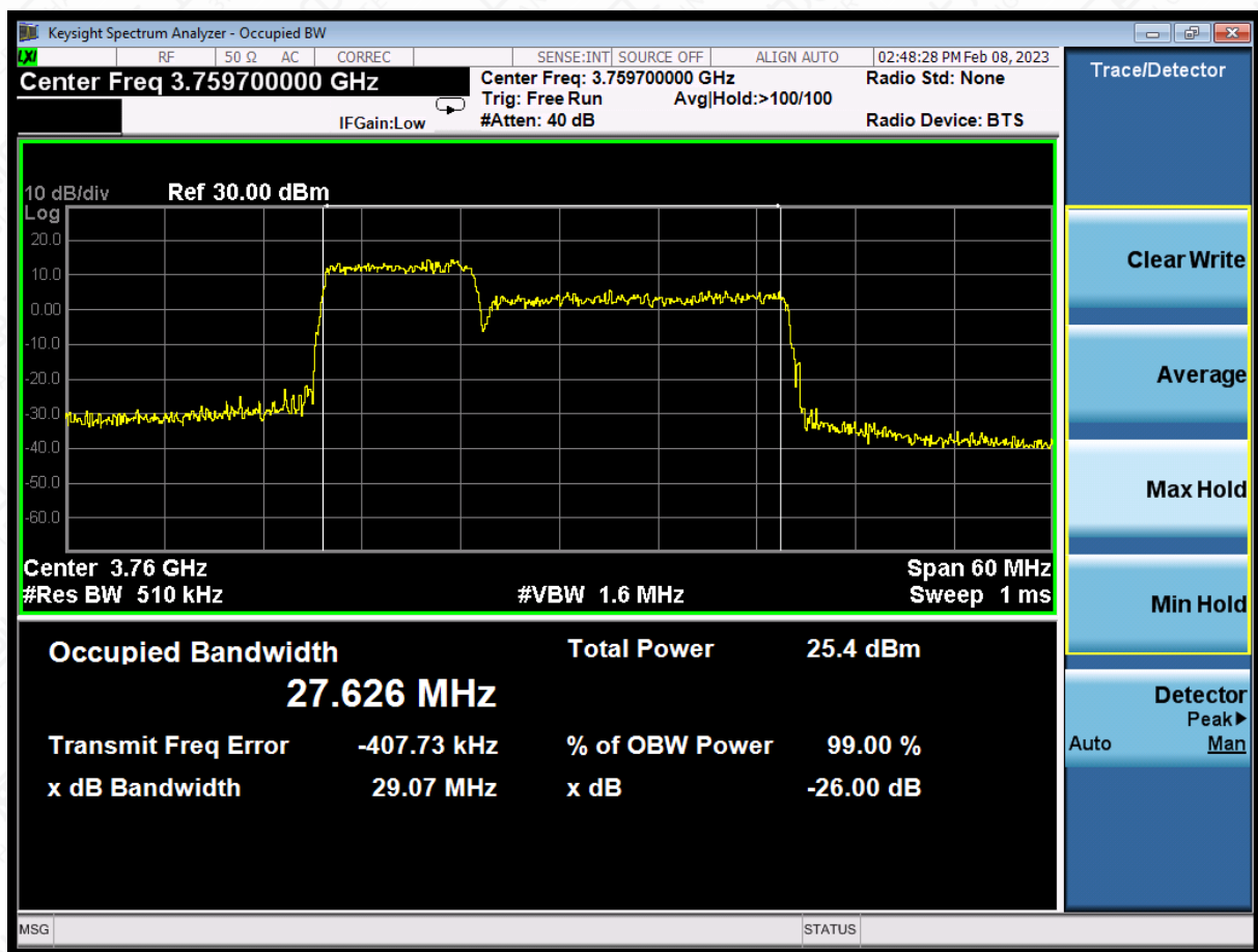
LTE CA band 43Part27 , 10MHz+20MHz Bandwidth,16QAM (99% BW)
