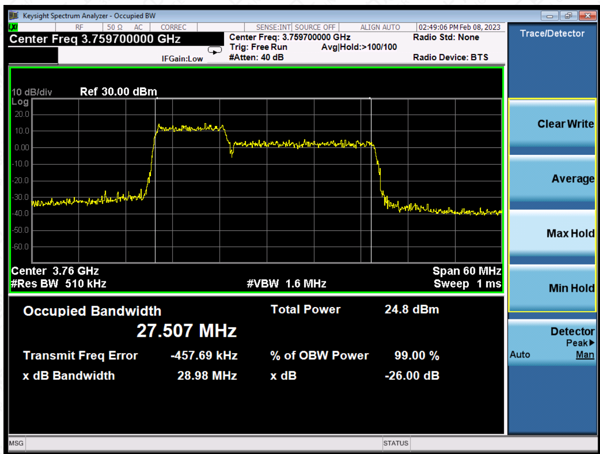
LTE CA band 43Part27 , 10MHz+20MHz Bandwidth,64QAM (99% BW)
