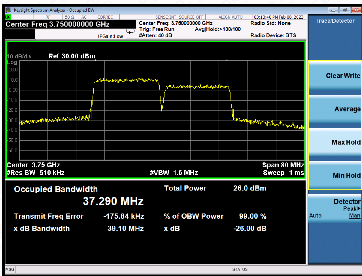
LTE CA band 43Part27 , 20MHz+20MHz Bandwidth,16QAM (99% BW)
