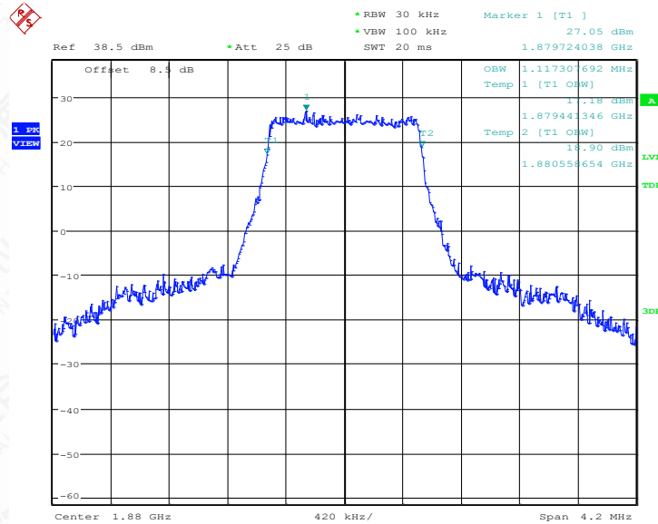
LTE band 2@CA_2+66, 1.4MHz Bandwidth, 64QAM (99% BW)
