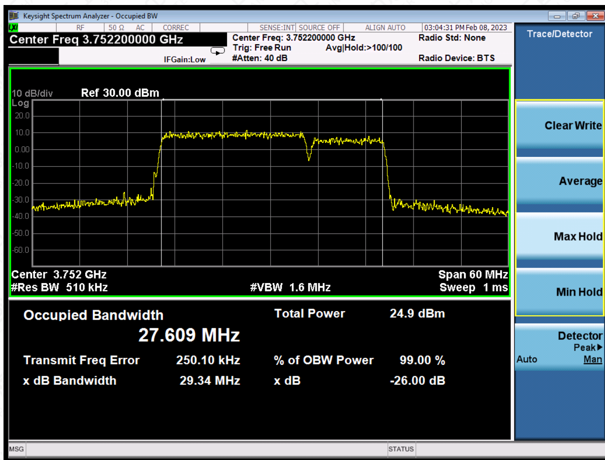
LTE CA band 43Part27 , 20MHz+10MHz Bandwidth,64QAM (99% BW)
