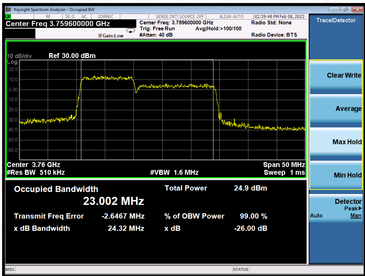
LTE CA band 43Part27 , 10MHz+15MHz Bandwidth,64QAM (99% BW)
