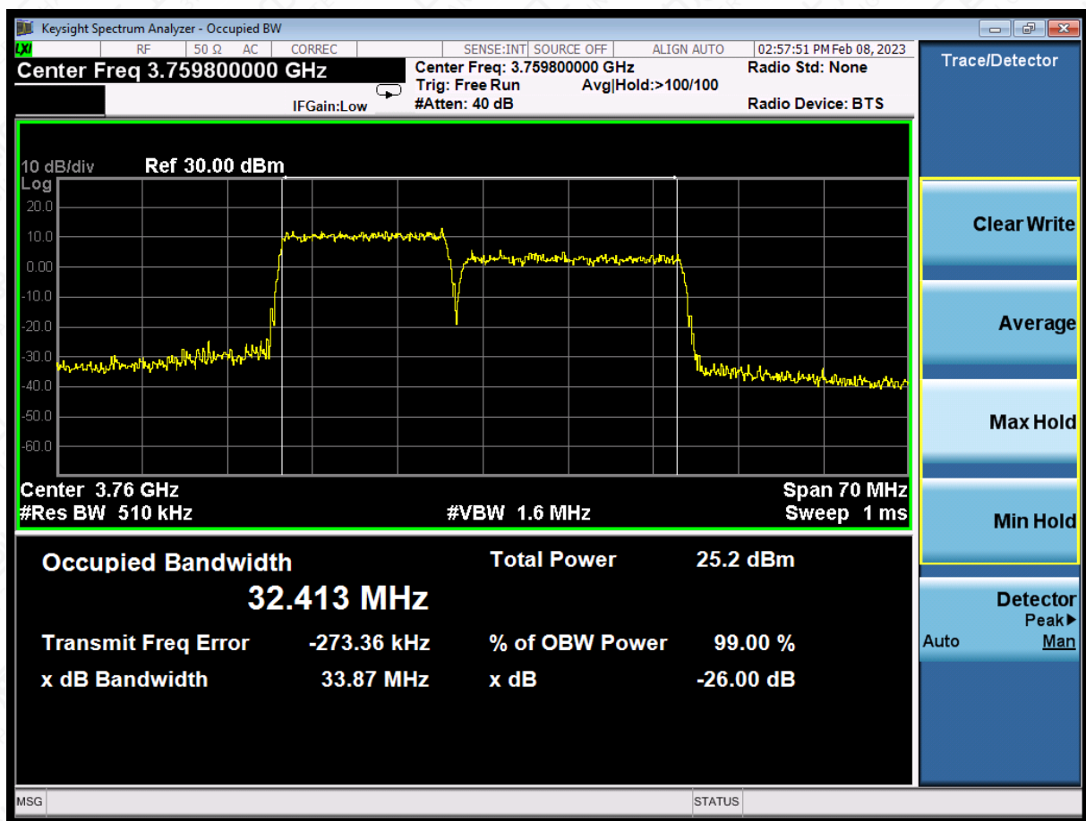
LTE CA band 43Part27,20MHz+10MHz(99%)*
