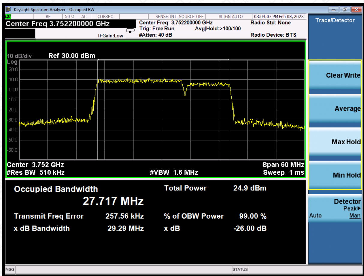
LTE CA band 43Part27,20MHz+15MHz(99%)*
