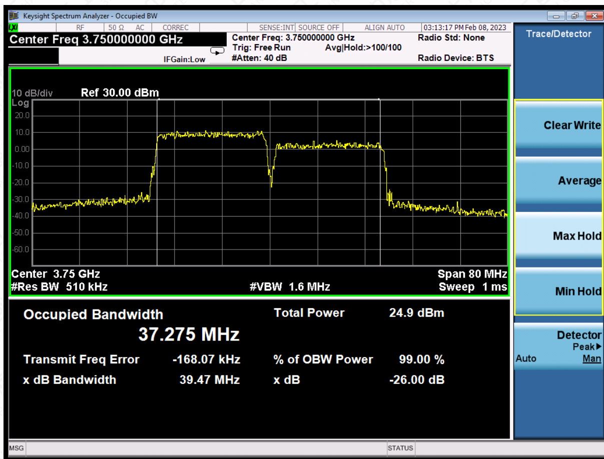
LTE CA band 43Part27 , 20MHz+20MHz Bandwidth,64QAM (99% BW)
