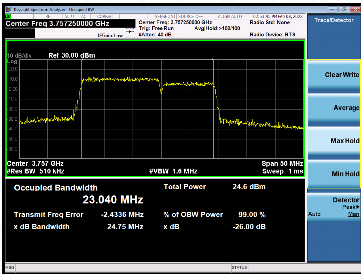
LTE CA band 43Part27 , 15MHz+10MHz Bandwidth,64QAM (99% BW)
