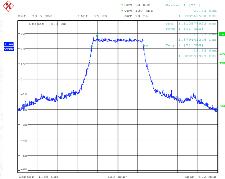
LTE band 2@CA_2+66, 1.4MHz Bandwidth, QPSK (99% BW)
