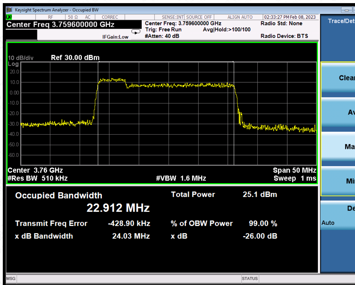
LTE CA band 43Part27,20MHz+5MHz(99%)*
