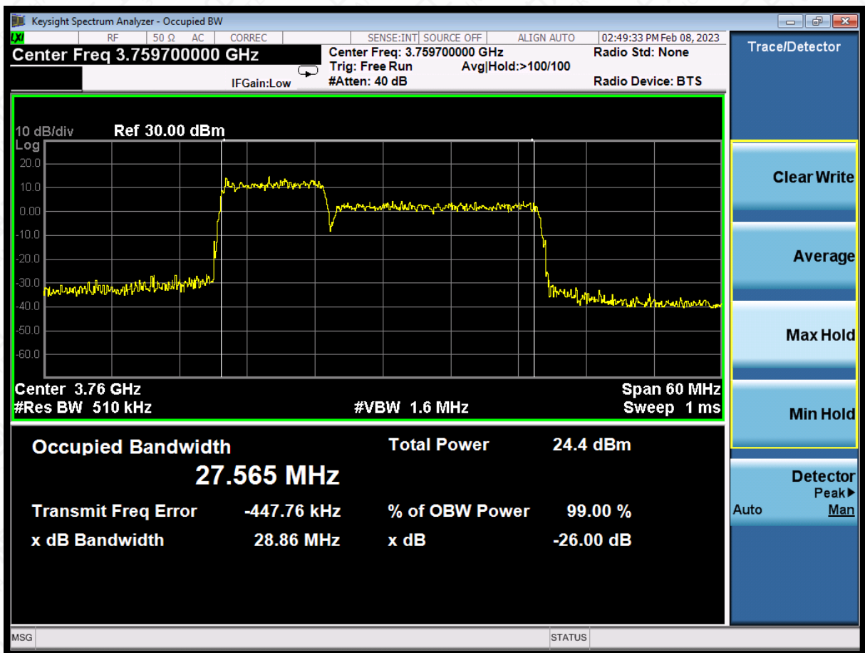
LTE CA band 43Part27,15MHz+10MHz(99%)*
