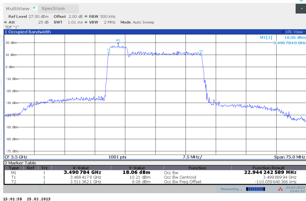
LTE CA band 42Part27 , 5MHz+20MHz Bandwidth,16QAM (99% BW)
