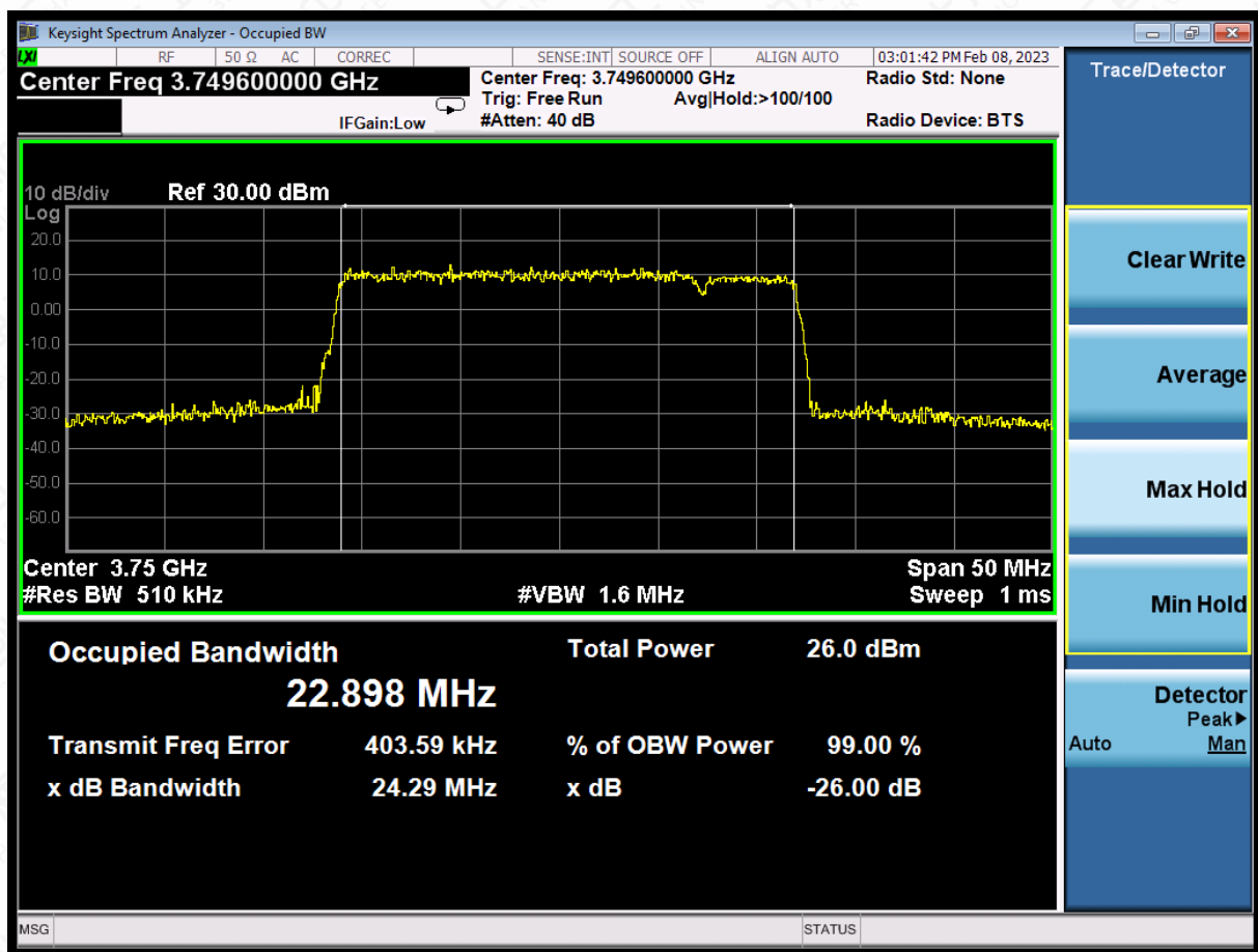
LTE CA band 43Part27 , 20MHz+5MHz Bandwidth,16QAM (99% BW)
