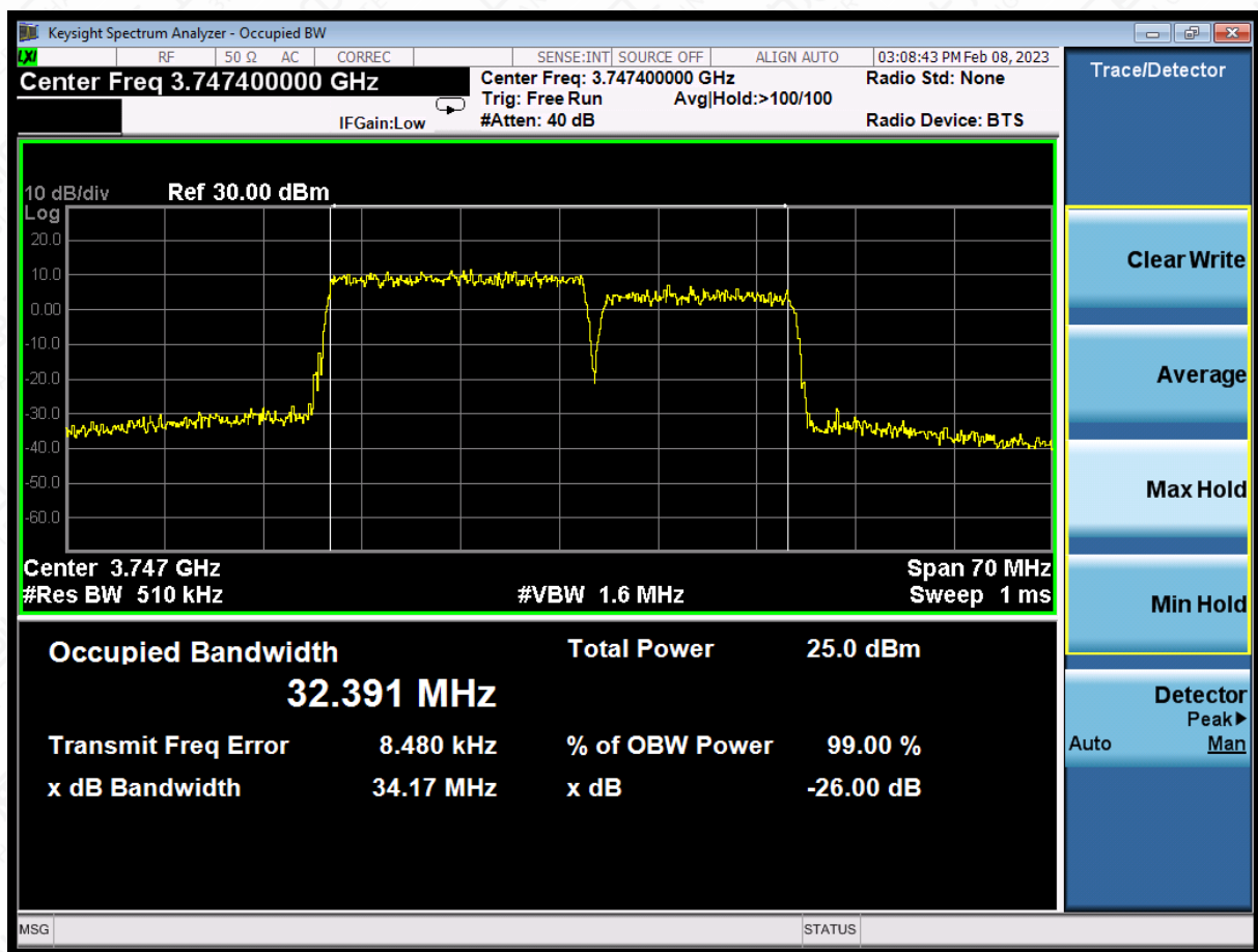
LTE CA band 43Part27 , 20MHz+15MHz Bandwidth,64QAM (99% BW)
