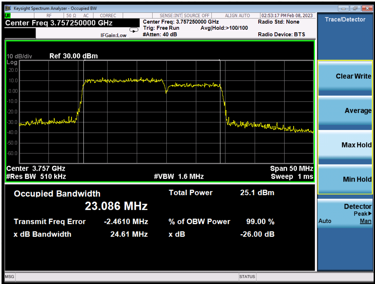
LTE CA band 43Part27,15MHz+15MHz(99%)*
