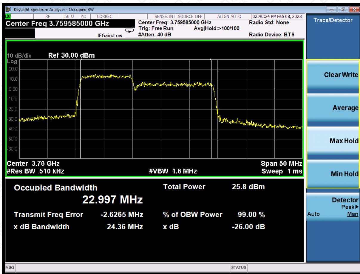
LTE CA band 43Part27 , 10MHz+15MHz Bandwidth,16QAM (99% BW)
