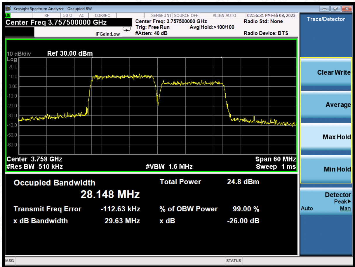
LTE CA band 43Part27,10MHz+15MHz(99%)*
