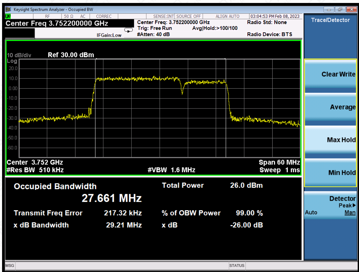
LTE CA band 43Part27 , 20MHz+10MHz Bandwidth,16QAM (99% BW)
