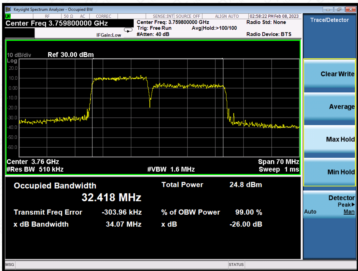
LTE CA band 43Part27 , 15MHz+20MHz Bandwidth,64QAM (99% BW)
