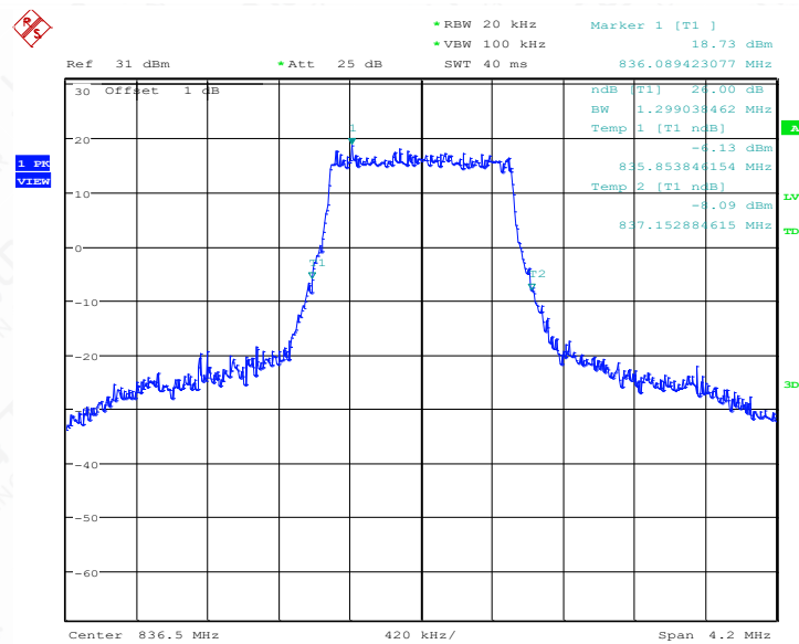
LTE band 5 , 1.4MHz Bandwidth,MID,QPSK (-26dBc BW)
