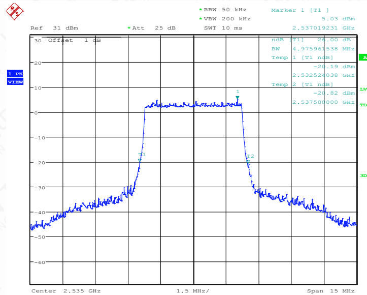
LTE band 7 , 5MHz Bandwidth,MID,QPSK (-26dB BW)
