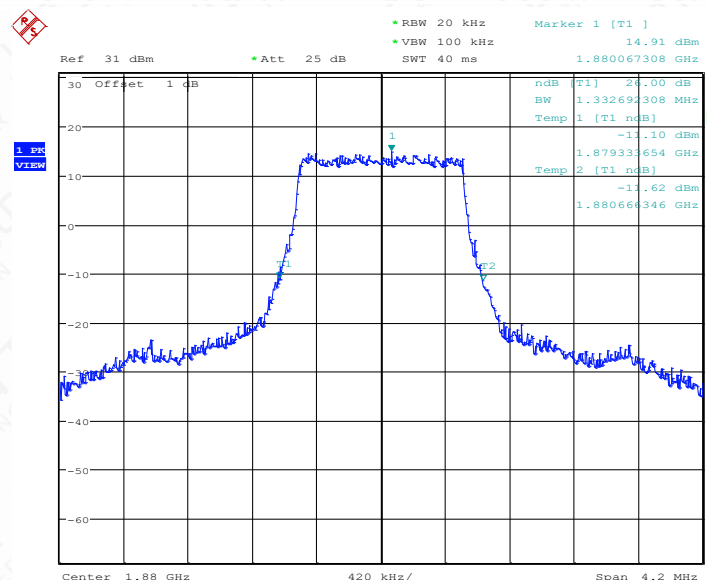
LTE band 2 , 1.4MHz Bandwidth,MID,QPSK (-26dBc BW)
