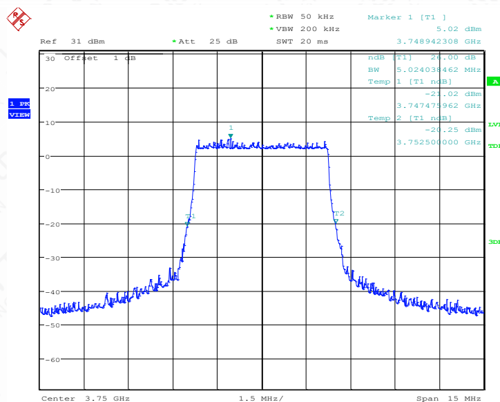
LTE band 43 , 5MHz Bandwidth,MID,QPSK (-26dBc BW)
