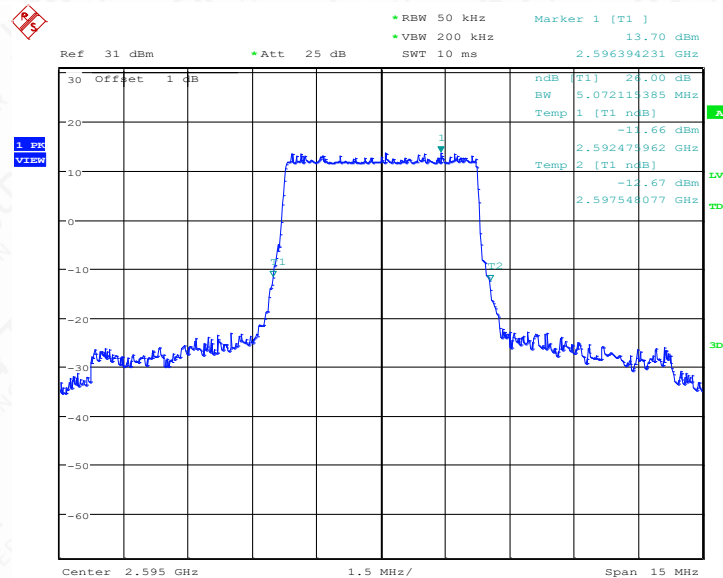
LTE band 38 , 5MHz Bandwidth,MID,QPSK (-26dBc BW)
