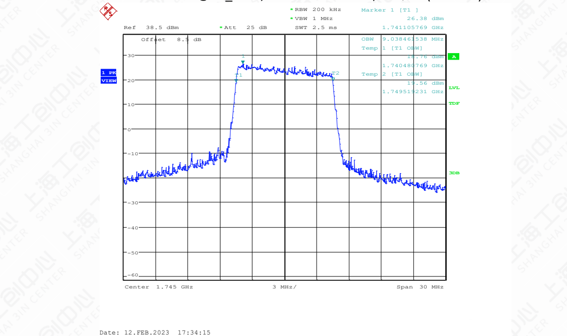
LTE band 66@CA_2+66, 10MHz Bandwidth, 64QAM (99% BW)
