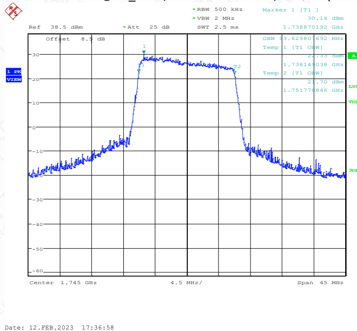
LTE band 66@CA_2+66, 15MHz Bandwidth, 64QAM (99% BW)
