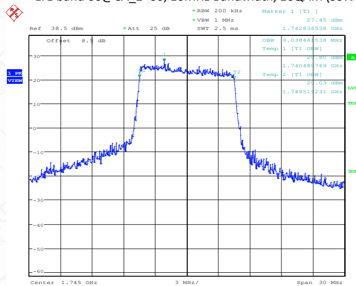
LTE band 66@CA_2+66, 10MHz Bandwidth, 16QAM (99% BW)
