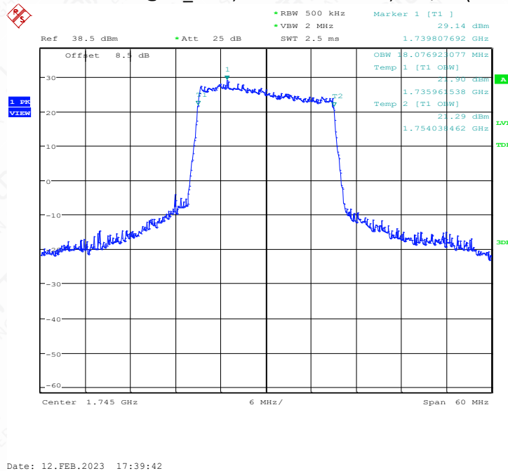
LTE band 66@CA_2+66, 20MHz Bandwidth, 64QAM (99% BW)
