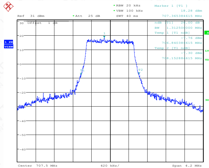
LTE band 12 , 1.4MHz Bandwidth,MID,QPSK (-26dBc BW)
