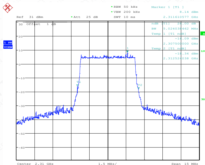
LTE band 30 , 5MHz Bandwidth,MID,64QAM (-26dBc BW)
