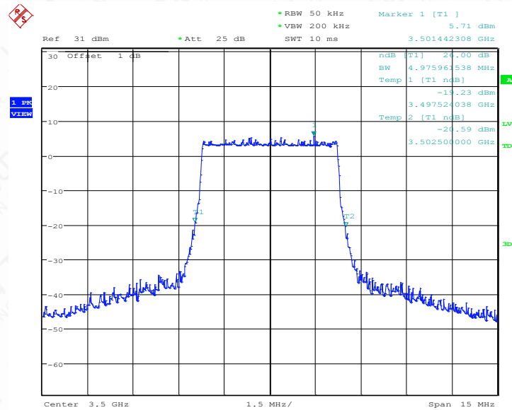
LTE band 42 , 5MHz Bandwidth,MID,QPSK (-26dBc BW)
