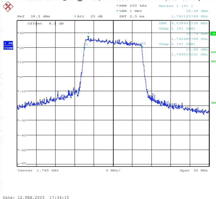
LTE band 66@CA_2+66, 10MHz Bandwidth, 64QAM (99% BW)
