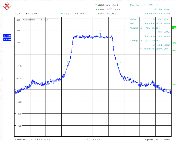
LTE band 4 , 1.4MHz Bandwidth,MID,QPSK (-26dBc BW)
