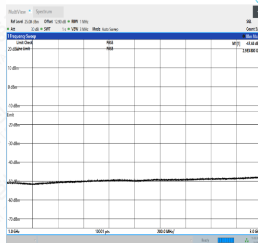
NTNV_N71_PC3_15_15_L_TID2_N/A_1000_3000_#1
