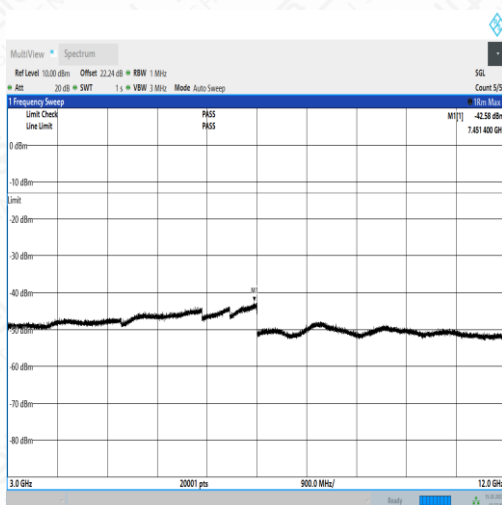
NTNV_N71_PC3_15_5_M_TID2_N/A_3000_12000_#1
