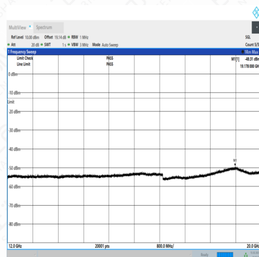
NTNV_N71_PC3_15_15_M_TID4_N/A_12000_20000_#1
