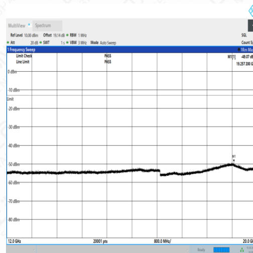
NTNV_N71_PC3_15_5_M_TID3_N/A_12000_20000_#1
