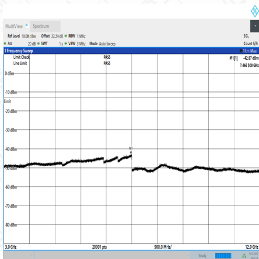
NTNV_N71_PC3_15_15_L_TID4_N/A_3000_12000_#1
