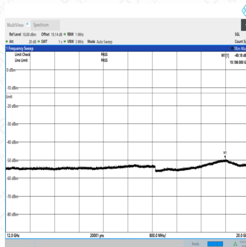
NTNV_N71_PC3_15_5_M_TID4_N/A_12000_20000_#1
