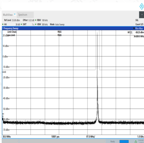
NTNV_N71_PC3_15_5_M_TID3_N/A_30_1000_#1
