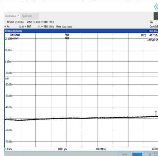
NTNV_N71_PC3_15_5_M_TID2_N/A_1000_3000_#1
