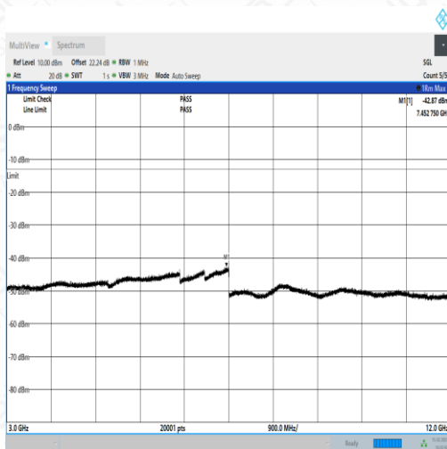
NTNV_N71_PC3_15_5_H_TID2_N/A_3000_12000_#1
