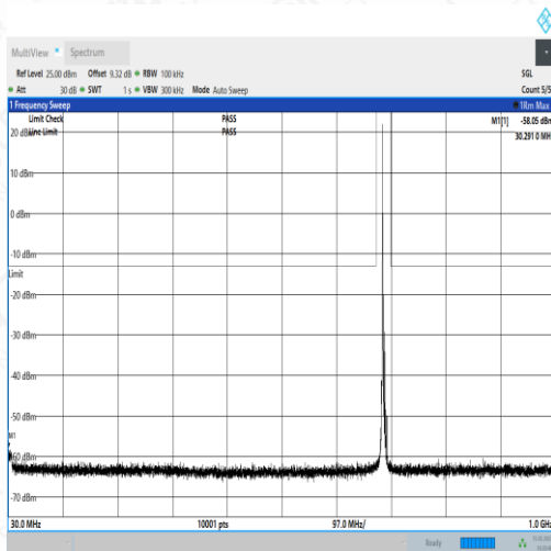
NTNV_N71_PC3_15_5_H_TID3_N/A_30_1000_#1
