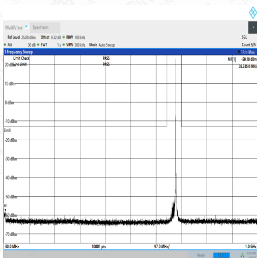
NTNV_N71_PC3_15_15_M_TID2_N/A_30_1000_#1
