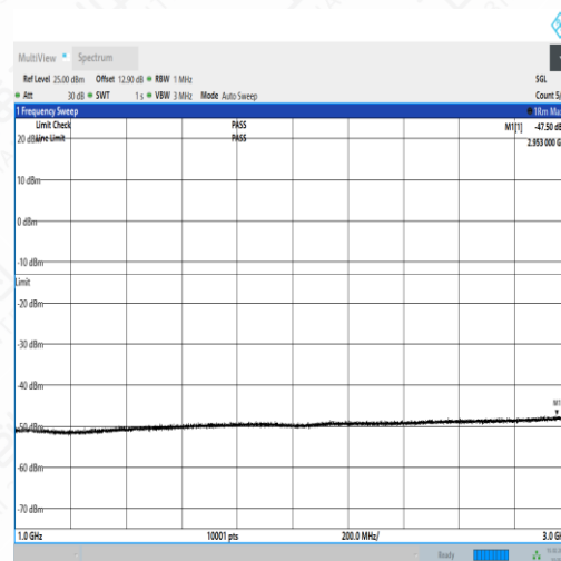
NTNV_N71_PC3_15_5_H_TID4_N/A_1000_3000_#1
