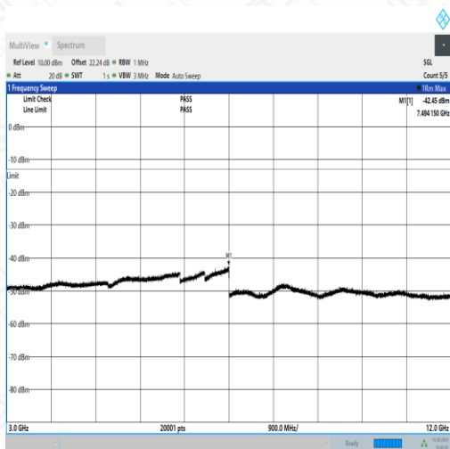
NTNV_N71_PC3_15_15_M_TID2_N/A_3000_12000_#1
