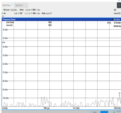
NTNV_N71_PC3_15_15_L_TID2_N/A_0.009_0.15_#1
