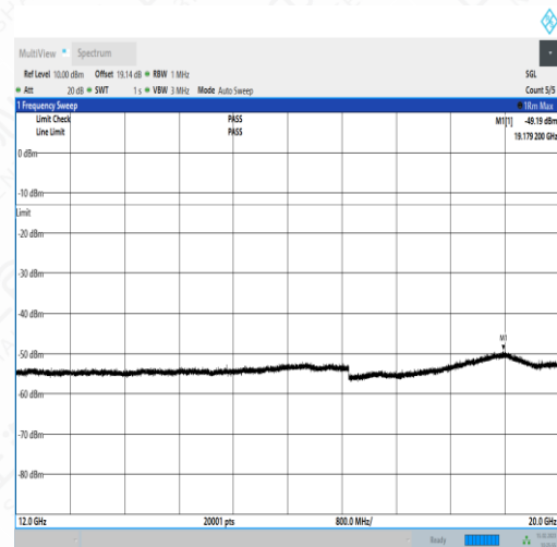
NTNV_N71_PC3_15_5_M_TID1_N/A_12000_20000_#1
