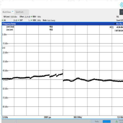
NTNV_N71_PC3_15_5_H_TID1_N/A_3000_12000_#1
