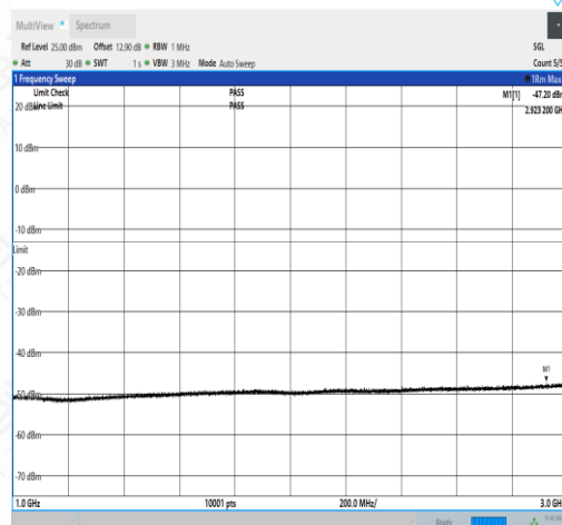
NTNV_N71_PC3_15_15_M_TID1_N/A_1000_3000_#1
