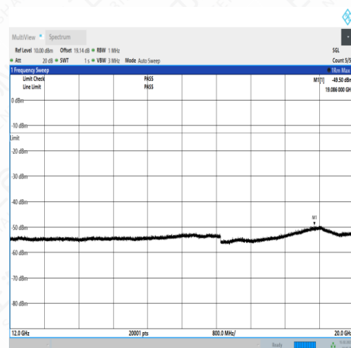
NTNV_N71_PC3_15_15_M_TID3_N/A_12000_20000_#1
