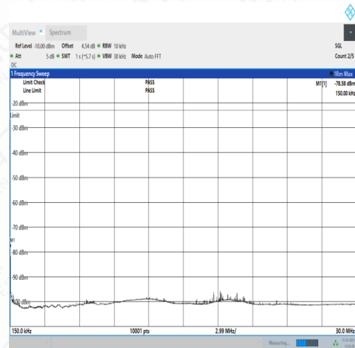
NTNV_N71_PC3_15_15_L_TID1_N/A_0.15_30_#1
