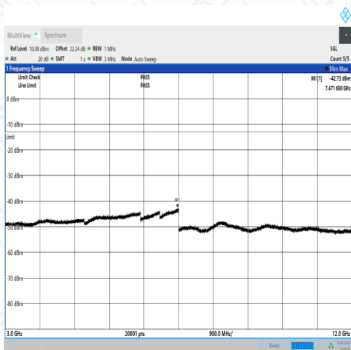
NTNV_N71_PC3_15_5_M_TID3_N/A_3000_12000_#1
