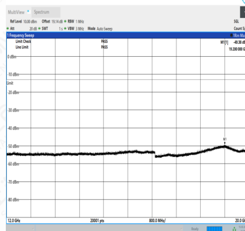
NTNV_N71_PC3_15_15_L_TID2_N/A_12000_20000_#1
