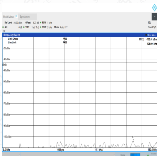
NTNV_N71_PC3_15_5_M_TID4_N/A_0.009_0.15_#1
