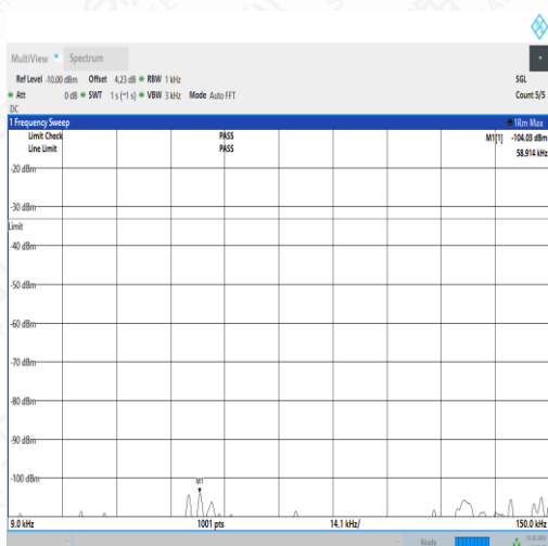
NTNV_N71_PC3_15_15_M_TID2_N/A_0.009_0.15_#1
