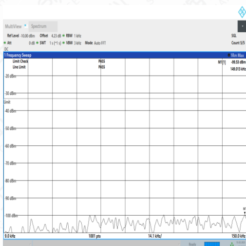
NTNV_N71_PC3_15_15_L_TID4_N/A_0.009_0.15_#1
