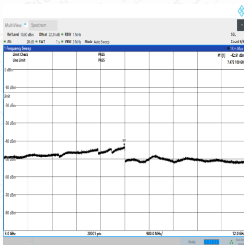
NTNV_N71_PC3_15_5_L_TID1_N/A_3000_12000_#1
