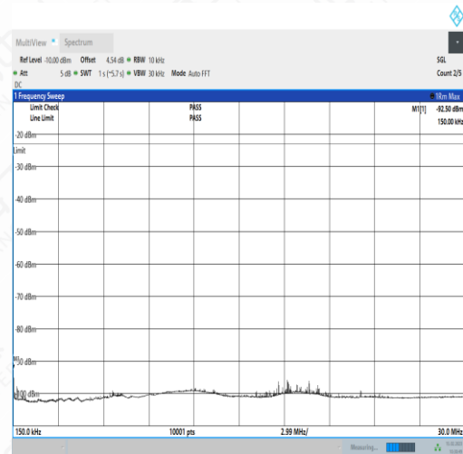
NTNV_N71_PC3_15_5_H_TID1_N/A_0.15_30_#1
