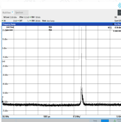
NTNV_N71_PC3_15_15_M_TID3_N/A_30_1000_#1
