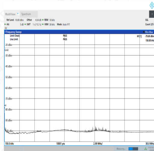
NTNV_N71_PC3_15_5_L_TID2_N/A_0.15_30_#1
