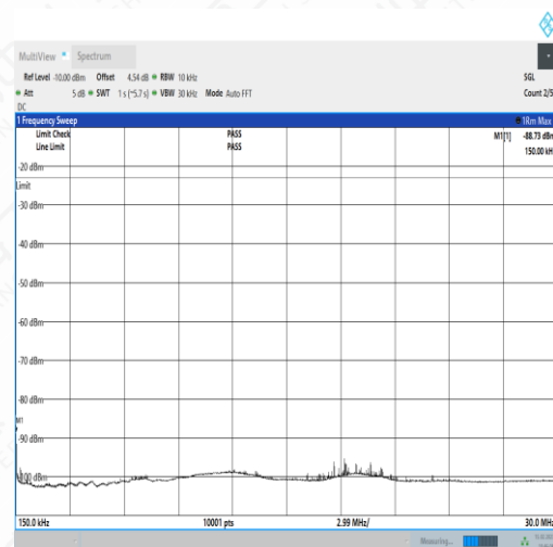
NTNV_N71_PC3_15_15_M_TID4_N/A_0.15_30_#1
