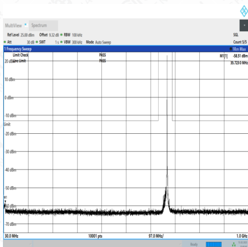
NTNV_N71_PC3_15_15_L_TID4_N/A_30_1000_#1
