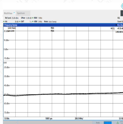
NTNV_N71_PC3_15_5_L_TID3_N/A_1000_3000_#1
