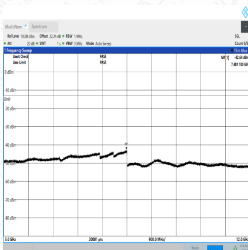
NTNV_N71_PC3_15_15_M_TID4_N/A_3000_12000_#1
