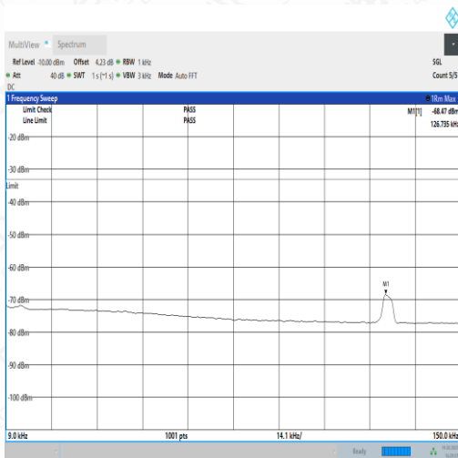
NTNV_N5_PC3_15_15_H_TID4_NS_01_0.009_0.15_#1
