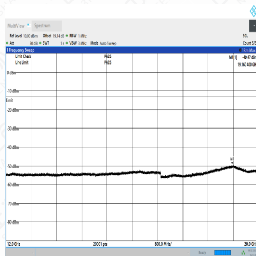
NTNV_N5_PC3_15_5_H_TID4_NS_01_12000_20000_#1
