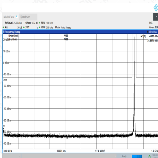
NTNV_N5_PC3_15_5_H_TID2_NS_01_30_1000_#1
