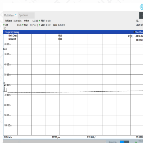
NTNV_N5_PC3_15_5_M_TID1_NS_01_0.15_30_#1
