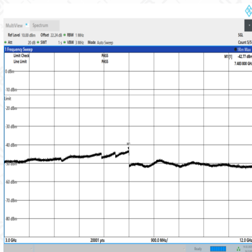
NTNV_N5_PC3_15_5_H_TID3_NS_01_3000_12000_#1
