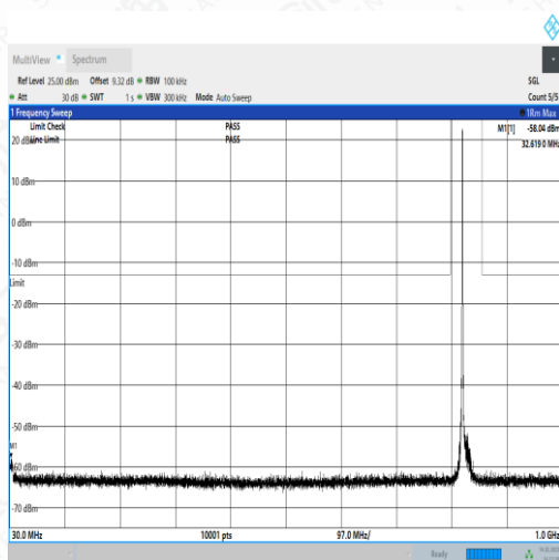
NTNV_N5_PC3_15_15_L_TID3_NS_01_30_1000_#1
