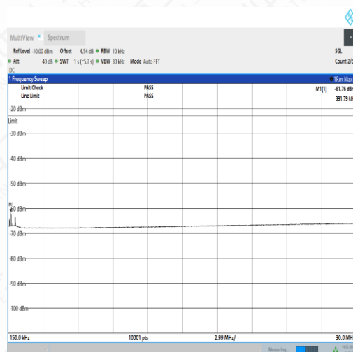
NTNV_N5_PC3_15_15_H_TID1_NS_01_0.15_30_#1
