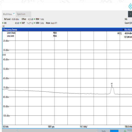
NTNV_N5_PC3_15_5_H_TID4_NS_01_0.009_0.15_#1
