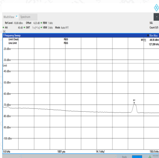
NTNV_N5_PC3_15_15_M_TID3_NS_01_0.009_0.15_#1
