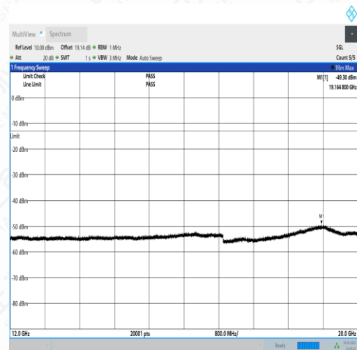
NTNV_N5_PC3_15_15_M_TID1_NS_01_12000_20000_#
