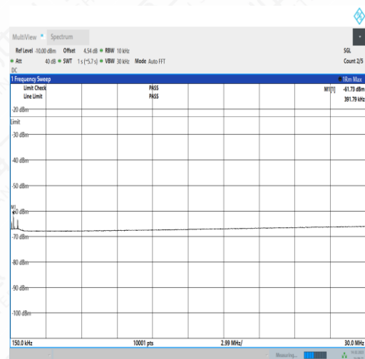
NTNV_N5_PC3_15_5_M_TID2_NS_01_0.15_30_#1
