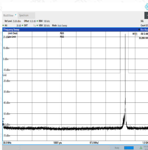
NTNV_N5_PC3_15_15_L_TID4_NS_01_30_1000_#1
