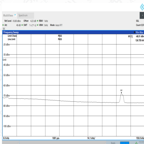
NTNV_N5_PC3_15_5_H_TID3_NS_01_0.009_0.15_#1
