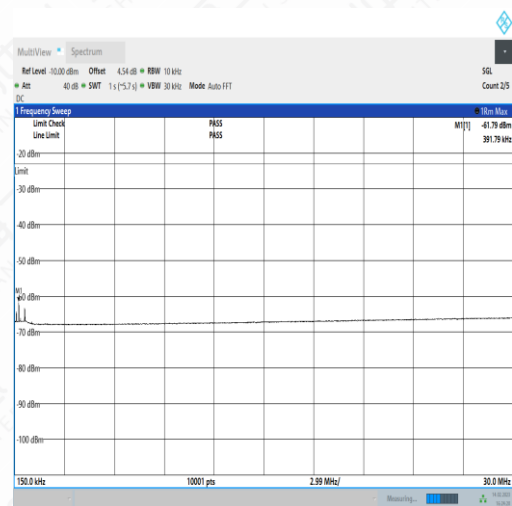
NTNV_N5_PC3_15_15_M_TID4_NS_01_0.15_30_#1
