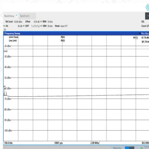
NTNV_N5_PC3_15_5_H_TID4_NS_01_0.15_30_#1
