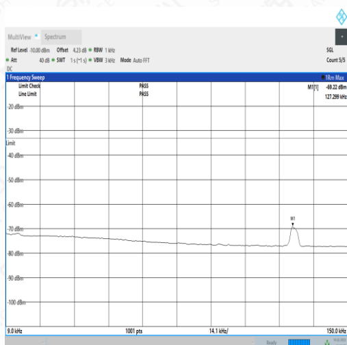
NTNV_N5_PC3_15_20_M_TID3_NS_01_0.009_0.15_#1
