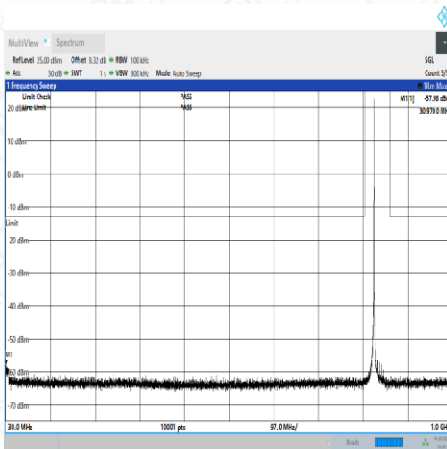
NTNV_N5_PC3_15_15_M_TID1_NS_01_30_1000_#1
