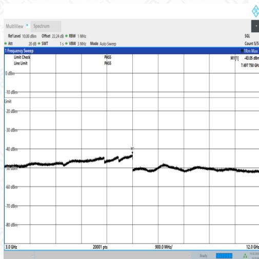
NTNV_N5_PC3_15_20_L_TID2_NS_01_3000_12000_#
