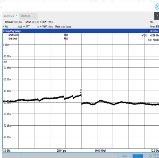
NTNV_N5_PC3_15_5_H_TID2_NS_01_3000_12000_#1
