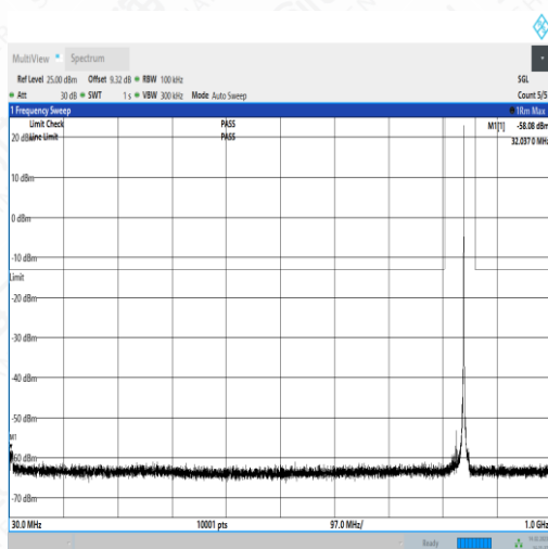
NTNV_N5_PC3_15_15_M_TID2_NS_01_30_1000_#1
