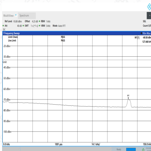
NTNV_N5_PC3_15_15_H_TID2_NS_01_0.009_0.15_#1
