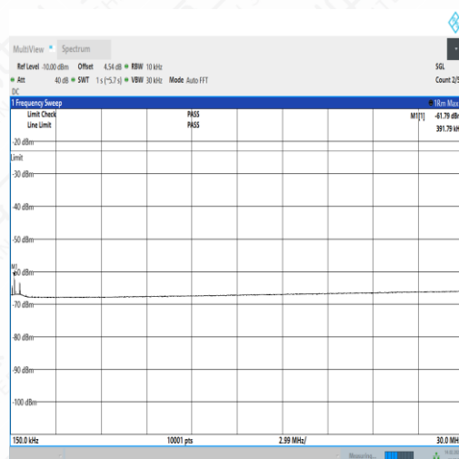
NTNV_N5_PC3_15_15_L_TID3_NS_01_0.15_30_#1
