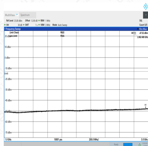
NTNV_N5_PC3_15_5_M_TID2_NS_01_1000_3000_#1
