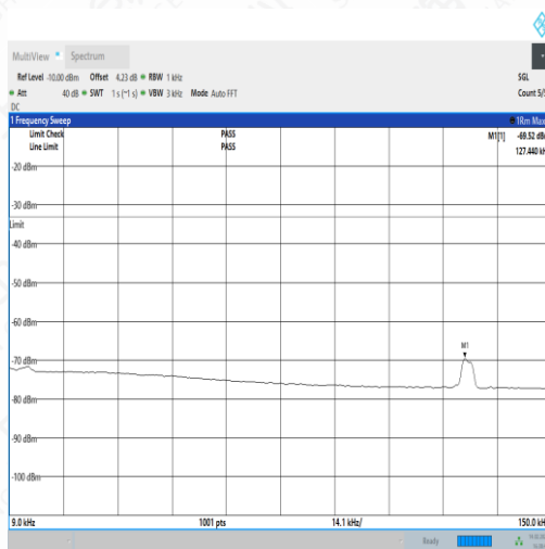
NTNV_N5_PC3_15_20_M_TID2_NS_01_0.009_0.15_#1
