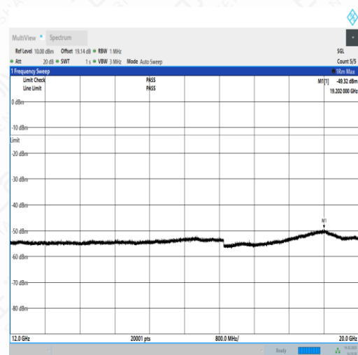
NTNV_N5_PC3_15_15_L_TID4_NS_01_12000_20000_#
