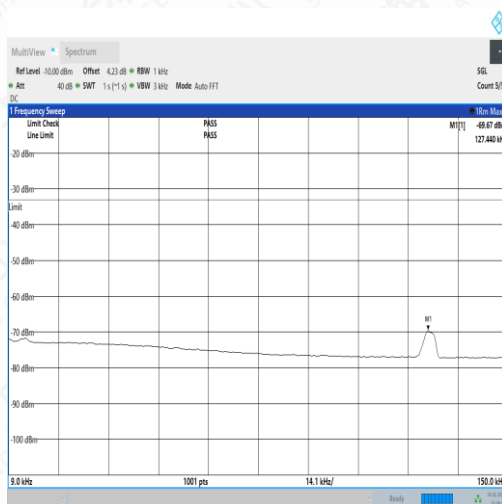
NTNV_N5_PC3_15_5_M_TID2_NS_01_0.009_0.15_#1
