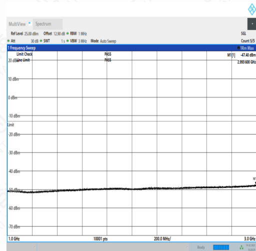
NTNV_N5_PC3_15_15_M_TID1_NS_01_1000_3000_#1
