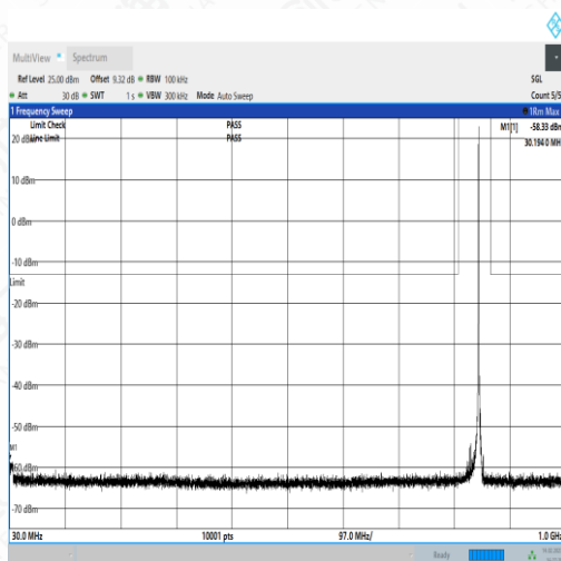
NTNV_N5_PC3_15_15_H_TID2_NS_01_30_1000_#1
