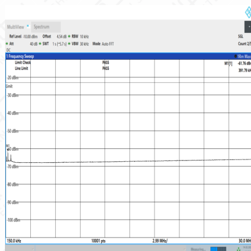
NTNV_N5_PC3_15_20_M_TID3_NS_01_0.15_30_#1
