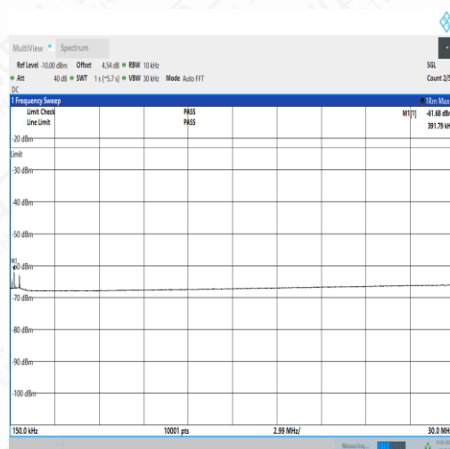
NTNV_N5_PC3_15_15_M_TID2_NS_01_0.15_30_#1
