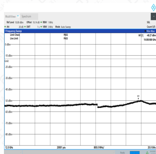
NTNV_N5_PC3_15_5_M_TID2_NS_01_12000_20000_#1
