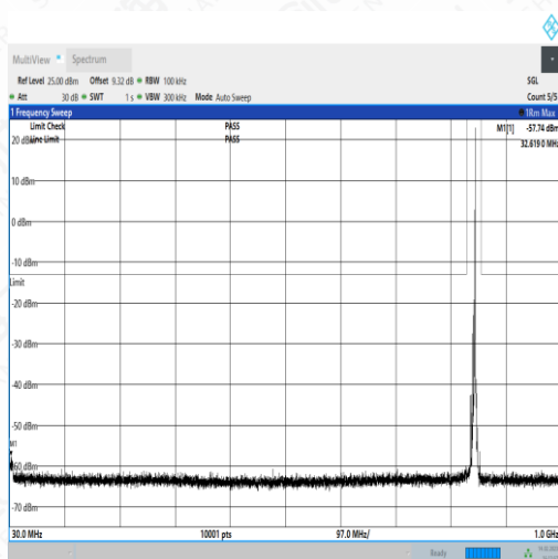
NTNV_N5_PC3_15_5_H_TID4_NS_01_30_1000_#1
