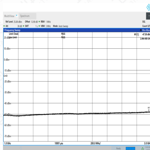
NTNV_N5_PC3_15_15_M_TID2_NS_01_1000_3000_#1
