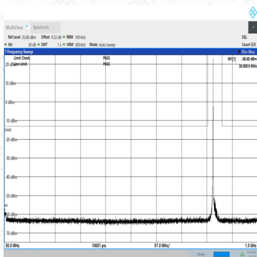
NTNV_N5_PC3_15_15_M_TID3_NS_01_30_1000_#1
