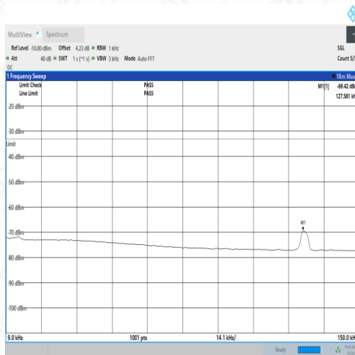
NTNV_N5_PC3_15_15_H_TID3_NS_01_0.009_0.15_#1
