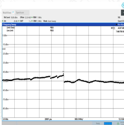
NTNV_N5_PC3_15_15_M_TID4_NS_01_3000_12000_#
