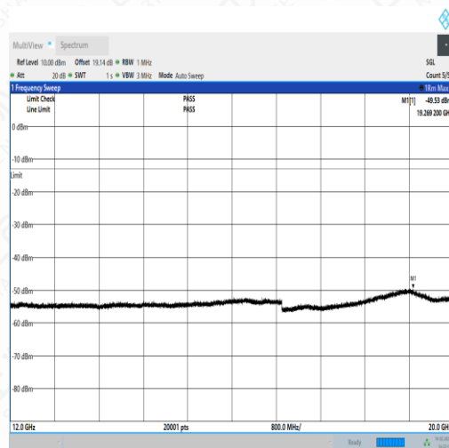
NTNV_N5_PC3_15_15_M_TID2_NS_01_12000_20000_#
