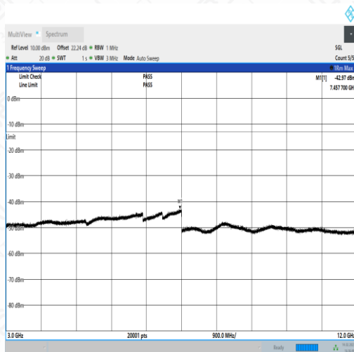
NTNV_N5_PC3_15_20_L_TID4_NS_01_3000_12000_#
