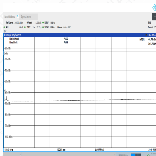
NTNV_N5_PC3_15_5_M_TID4_NS_01_0.15_30_#1
