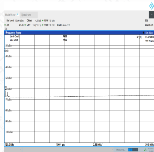
NTNV_N5_PC3_15_15_H_TID4_NS_01_0.15_30_#1
