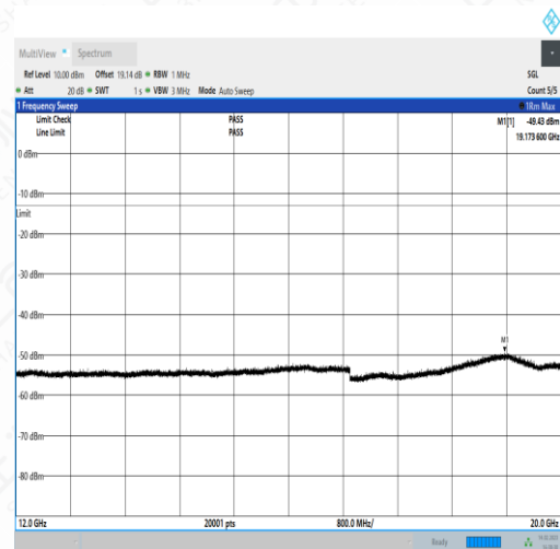
NTNV_N5_PC3_15_20_M_TID1_NS_01_12000_20000_#
