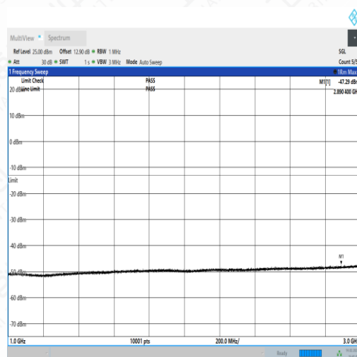
NTNV_N5_PC3_15_20_M_TID3_NS_01_1000_3000_#1
