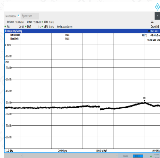
NTNV_N5_PC3_15_20_L_TID1_NS_01_12000_20000_#
