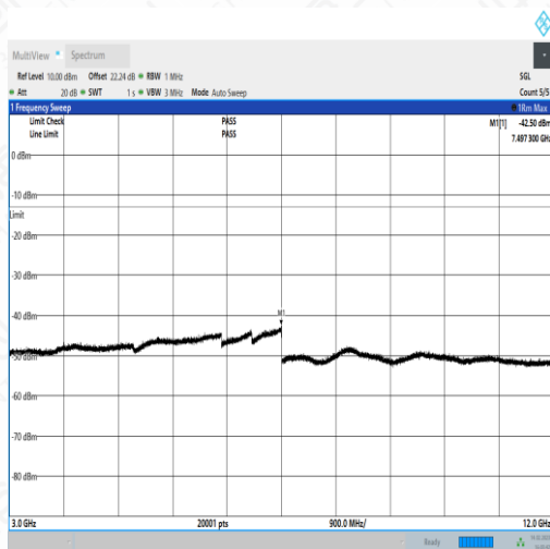
NTNV_N5_PC3_15_5_M_TID1_NS_01_3000_12000_#1
