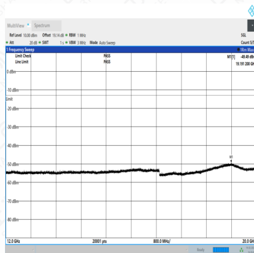
NTNV_N5_PC3_15_15_H_TID1_NS_01_12000_20000_#
