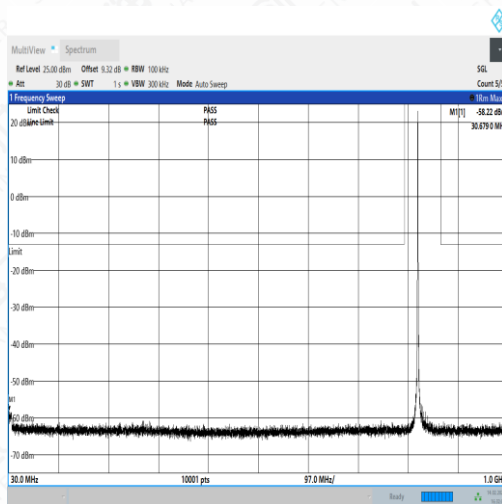
NTNV_N5_PC3_15_20_L_TID1_NS_01_30_1000_#1
