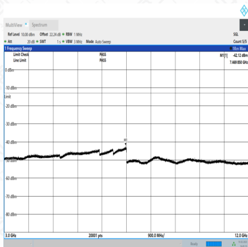
NTNV_N5_PC3_15_20_M_TID3_NS_01_3000_12000_#
