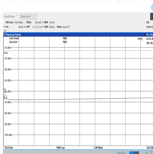
NTNV_N5_PC3_15_5_H_TID2_NS_01_0.15_30_#1
