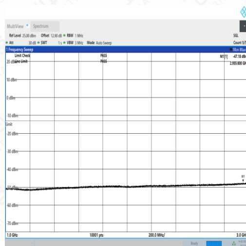
NTNV_N5_PC3_15_5_H_TID4_NS_01_1000_3000_#1
