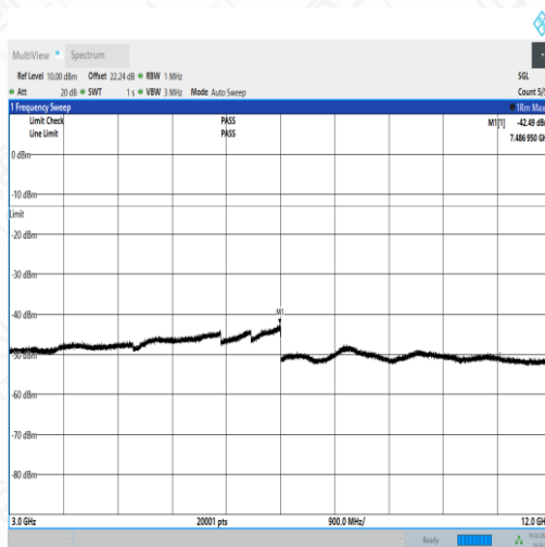
NTNV_N5_PC3_15_20_L_TID1_NS_01_3000_12000_#
