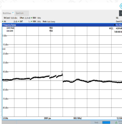
NTNV_N5_PC3_15_15_L_TID4_NS_01_3000_12000_#
