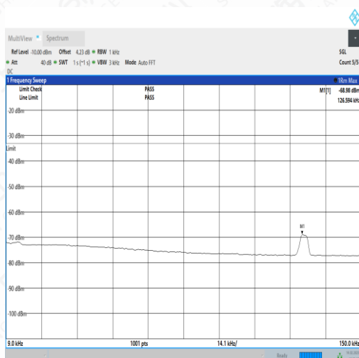
NTNV_N5_PC3_15_15_M_TID2_NS_01_0.009_0.15_#1
