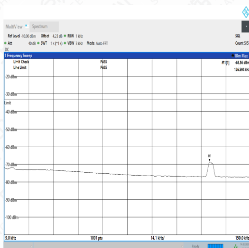
NTNV_N5_PC3_15_20_L_TID2_NS_01_0.009_0.15_#1
