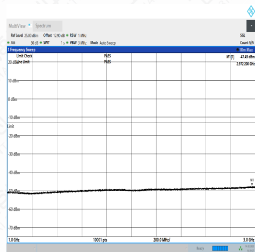
NTNV_N5_PC3_15_20_M_TID2_NS_01_1000_3000_#1
