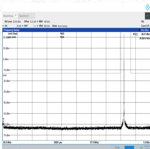
NTNV_N5_PC3_15_20_M_TID3_NS_01_30_1000_#1
