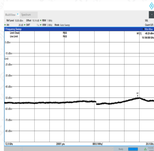
NTNV_N5_PC3_15_20_L_TID4_NS_01_12000_20000_#
