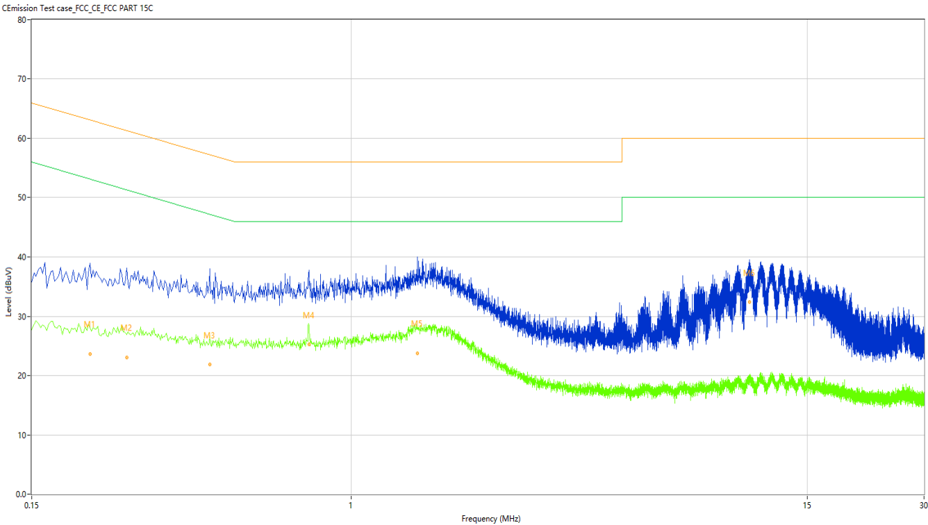
Figure 13: Conducted Emission on AC Mains, L Phase
