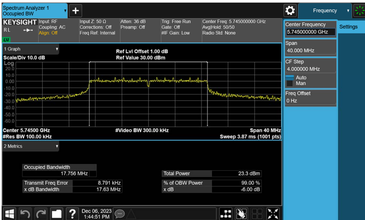
Figure 7: The plots of 6dB Bandwidth, 802.11ac(VHT20), 5745MHz
