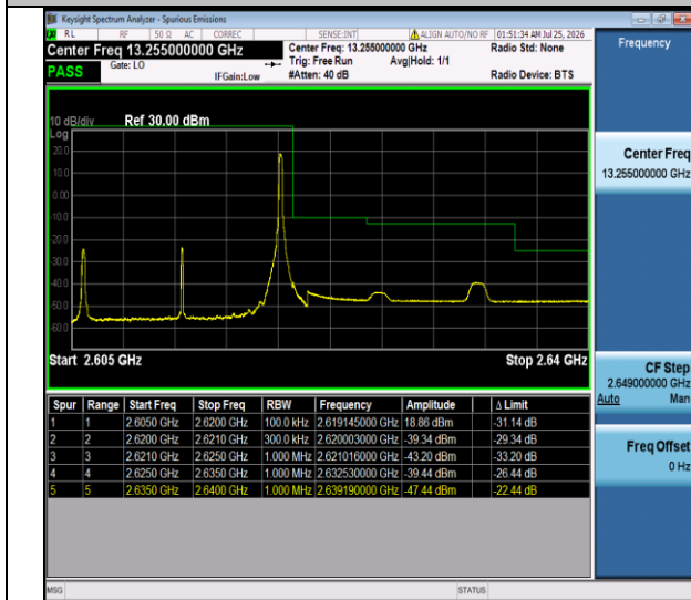
Band38-15MHz-QPSK-38175-1RB#74-PASS
