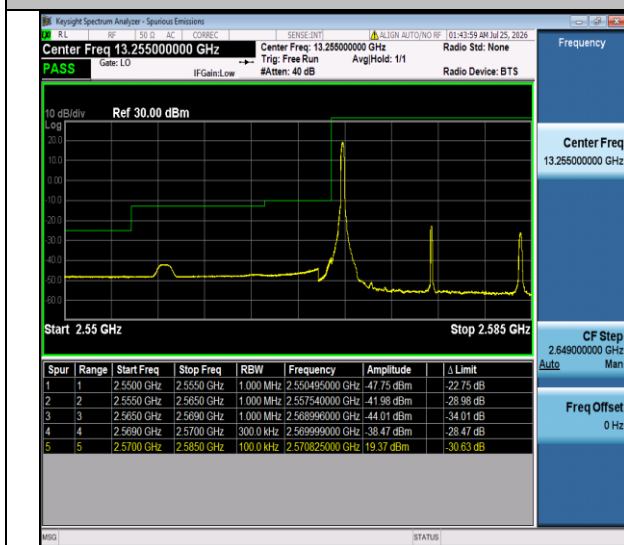
Band38-15MHz-QPSK-37825-1RB#0-PASS
