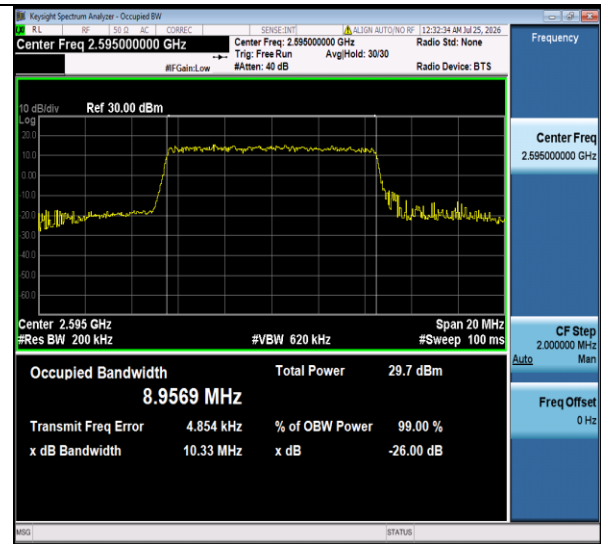
Band38-10MHz-16QAM-38000-50RB#0-PASS
