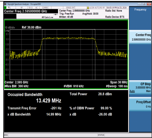
Band38-15MHz-64QAM-38000-75RB#0-PASS
