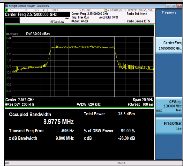
Band38-10MHz-64QAM-37800-50RB#0-PASS
