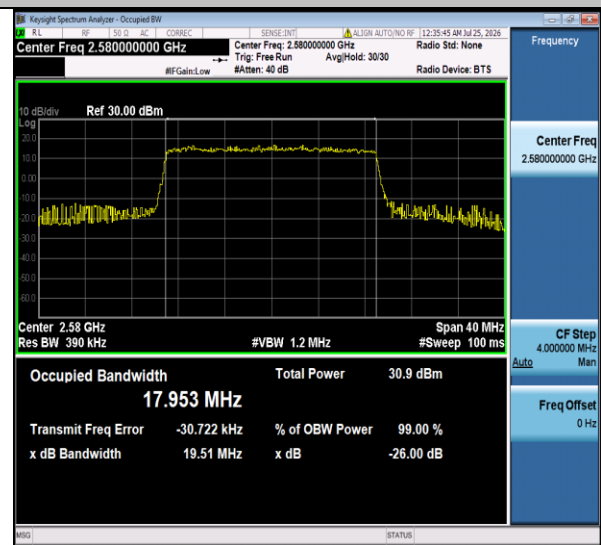
Band38-20MHz-QPSK-37850-100RB#0-PASS
