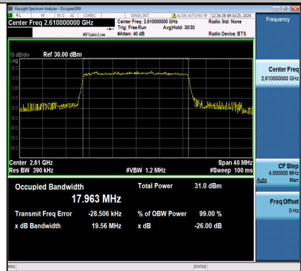
Band38-20MHz-QPSK-38150-100RB#0-PASS
