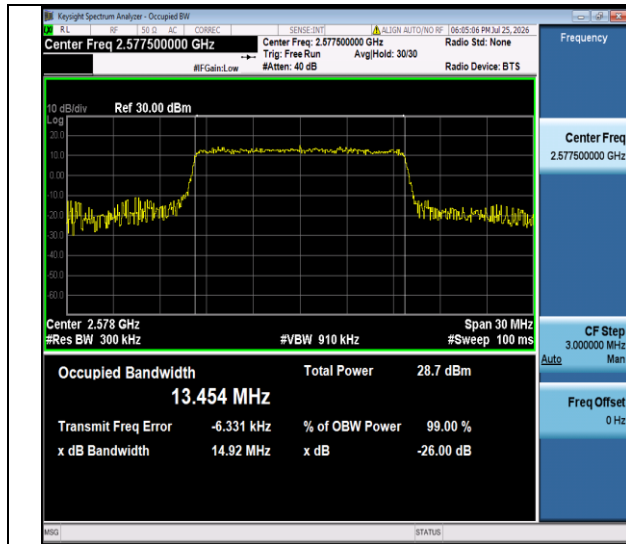
Band38-15MHz-64QAM-37825-75RB#0-PASS
