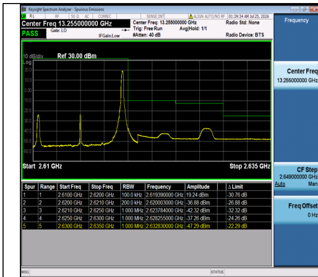
Band38-10MHz-QPSK-38200-1RB#49-PASS
