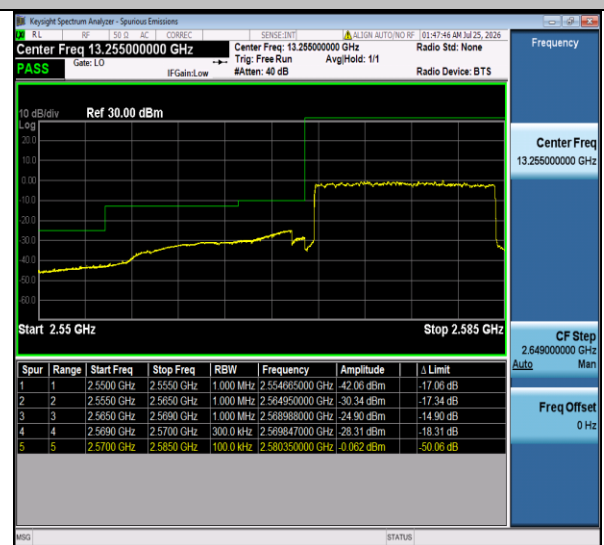
Band38-15MHz-QPSK-37825-75RB#0-PASS
