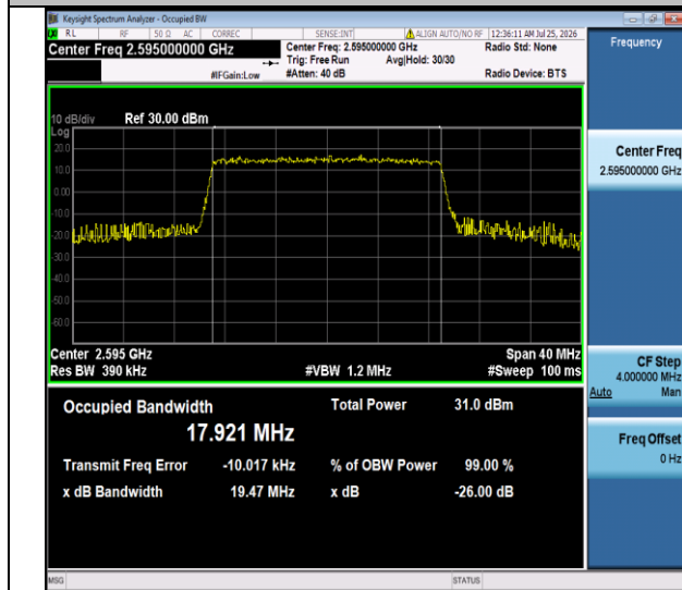
Band38-20MHz-QPSK-38000-100RB#0-PASS
