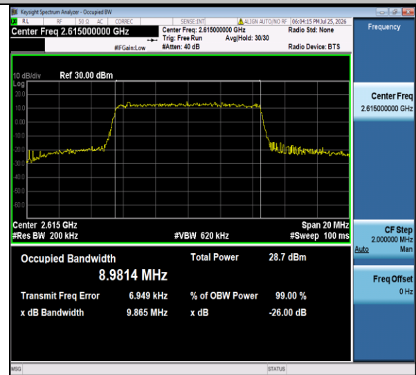
Band38-10MHz-64QAM-38200-50RB#0-PASS
