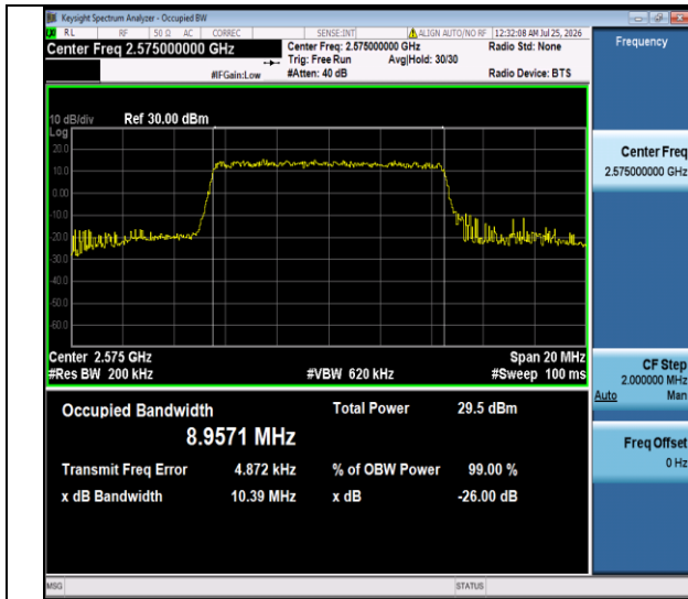
Band38-10MHz-16QAM-37800-50RB#0-PASS
