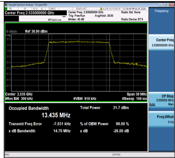
Band7-15MHz-QPSK-21100-75RB#0-PASS
