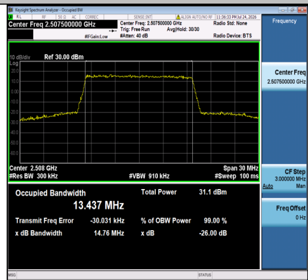
Band7-15MHz-16QAM-20825-75RB#0-PASS
