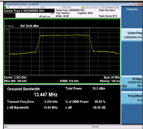
Band7-15MHz-16QAM-21375-75RB#0-PASS
