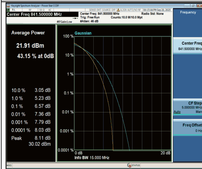
Band26(824-849)-15MHz-64QAM-26965-75RB#0-PASS
