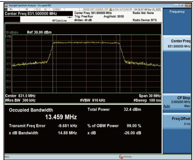
Band26(824-849)-15MHz-16QAM-26865-75RB#0-PASS
