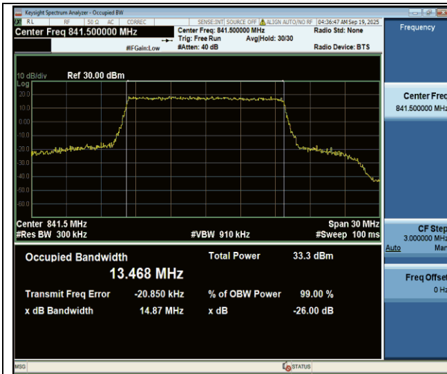
Band26(824-849)-15MHz-QPSK-26965-75RB#0-PASS
