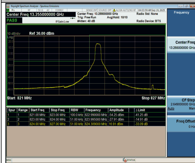
Band26(824-849)-5MHz-QPSK-26815-1RB#0-PASS
