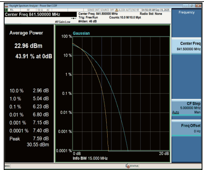
Band26(824-849)-15MHz-16QAM-26965-75RB#0-PASS
